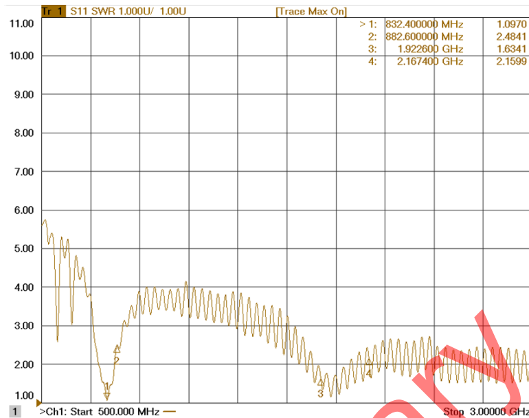
Figure 2-4-1 The antenna VSWR
