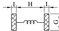
( PCB Pattern )
