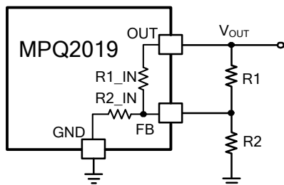
Figure 4. FB Divider for Fixed-Output Version
