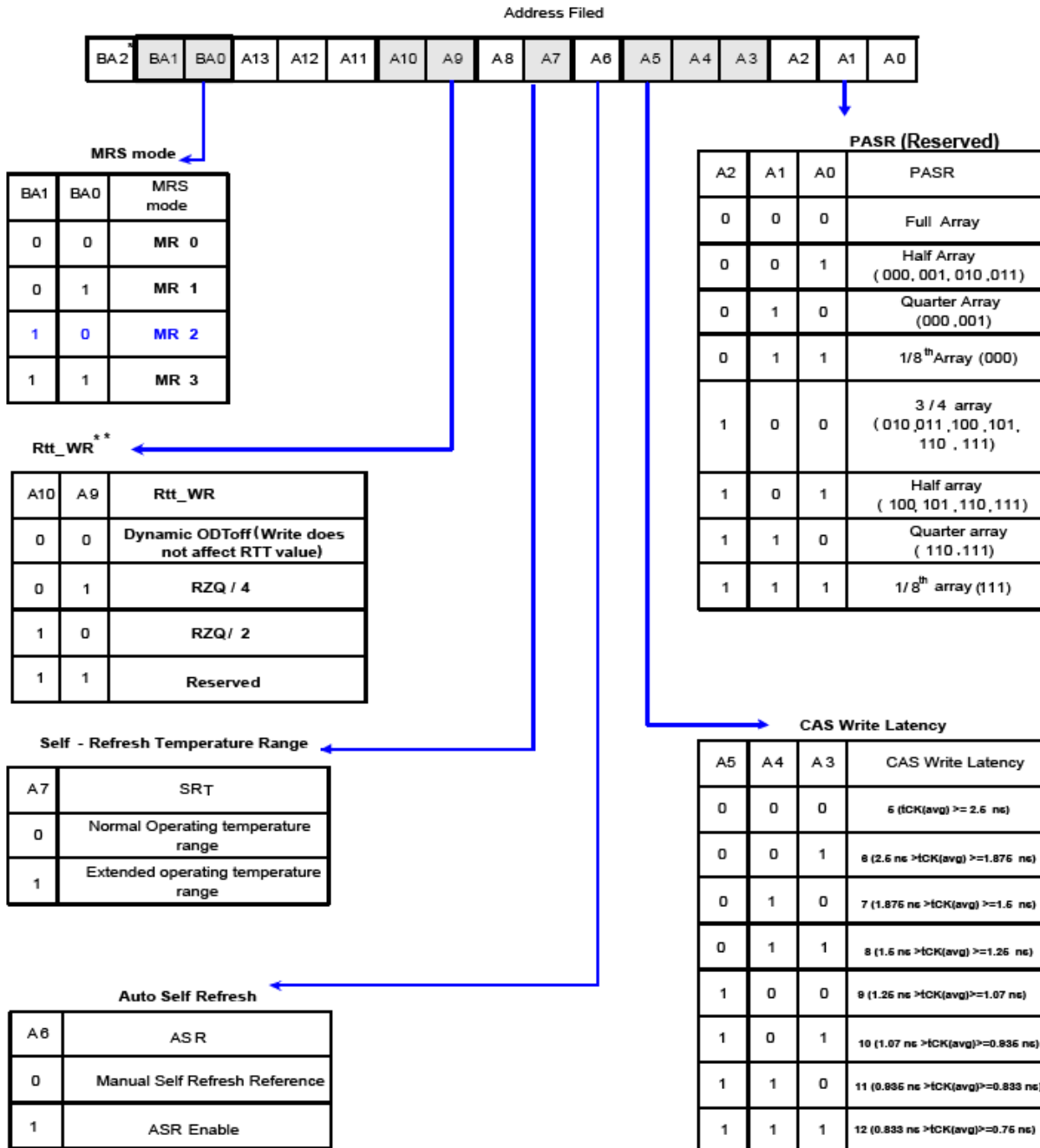
Fig. 7: MR2 Definition
