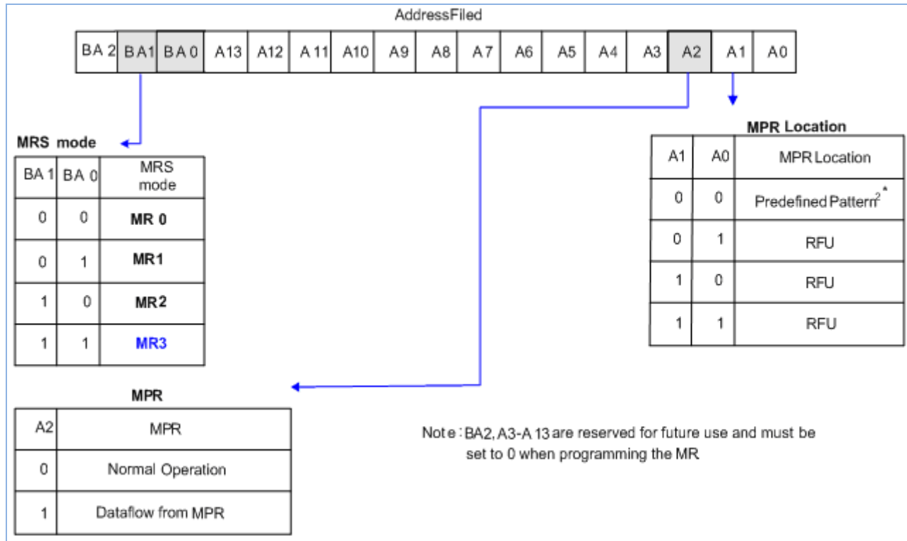
Fig. 8: MR3 Definition
