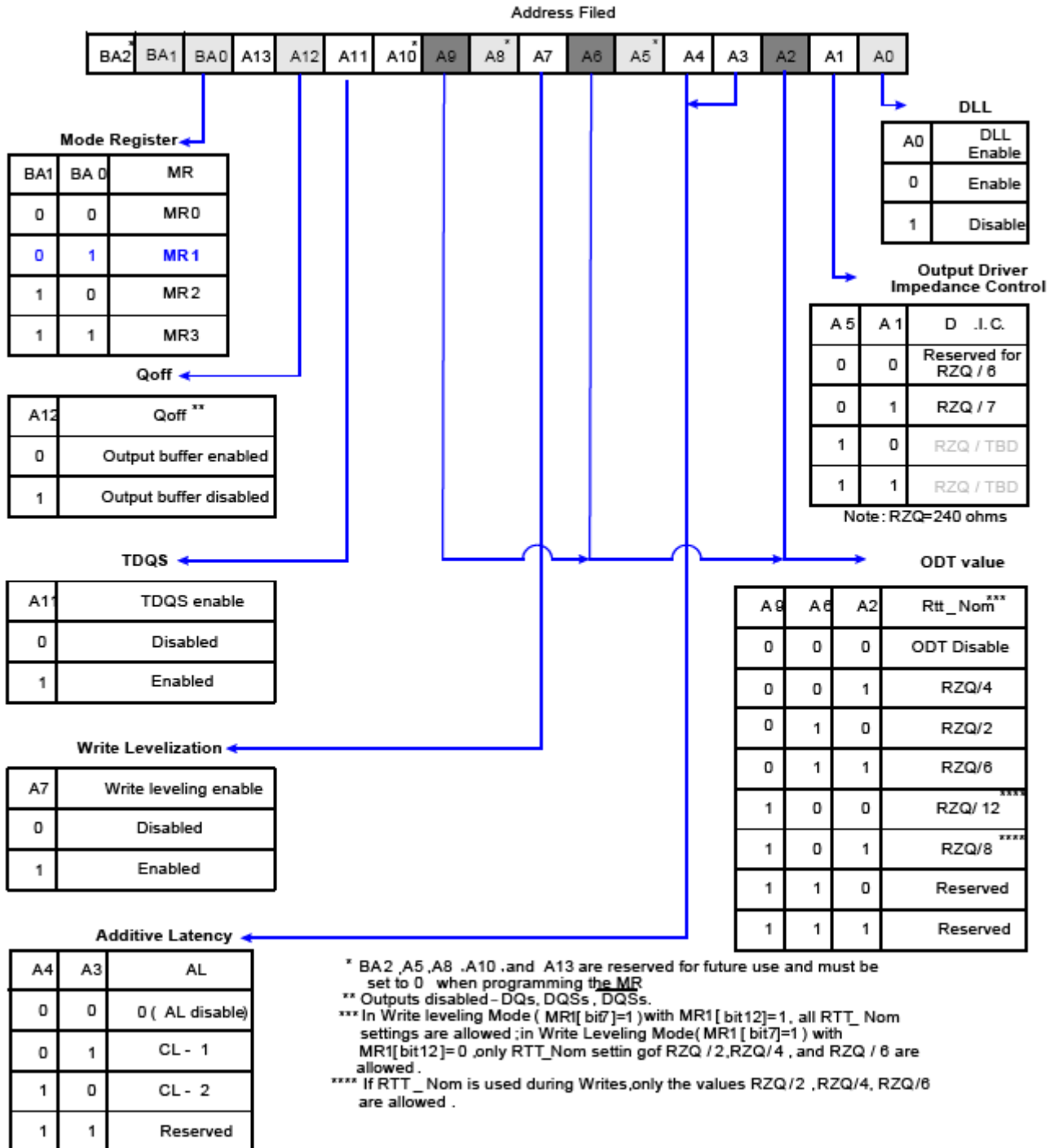
Fig. 6: MR1 Definition
