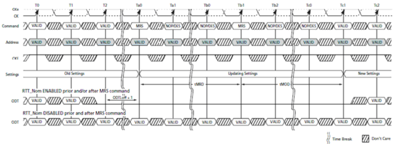
Fig. 3: tMRD Timing
