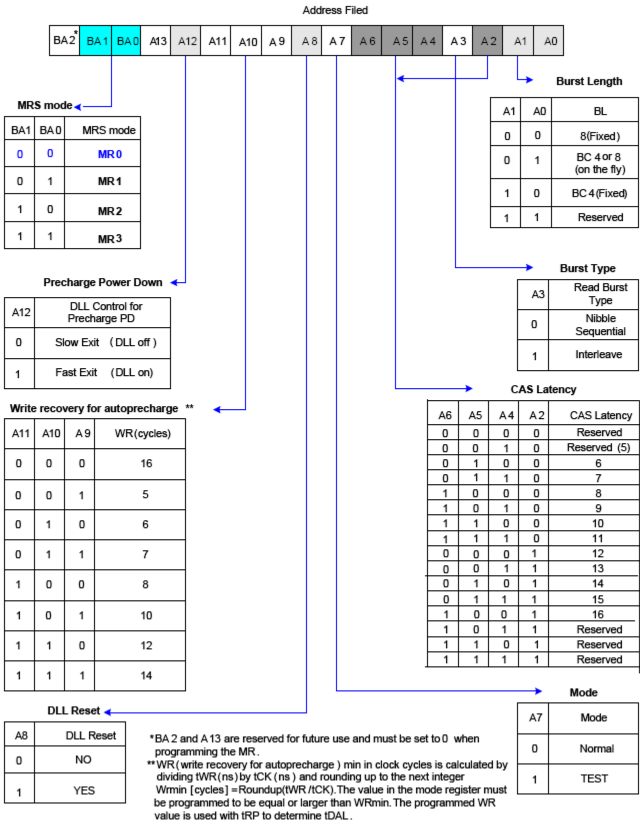
Fig. 5:MR0 Definition
