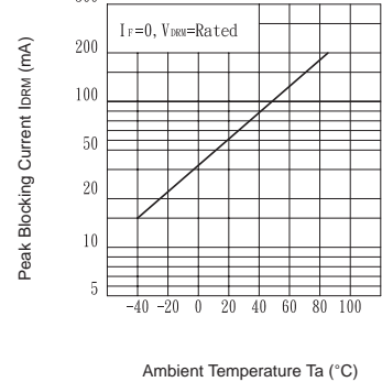
Fig.11 IDRM2, Leakage in Inhibit vs. Ambient Temperature
