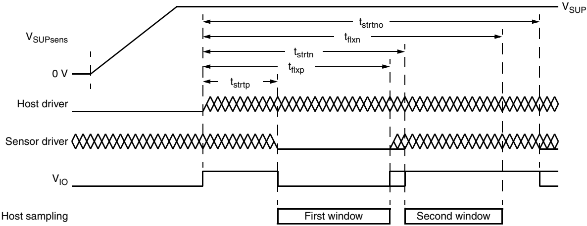
Fig. 3–2: Self-test timing diagram
