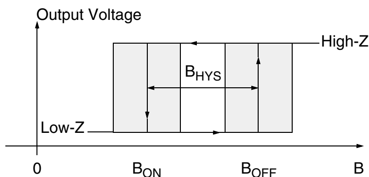
Fig. 4–12: Definition of magnetic switching points for the HAL 1509
