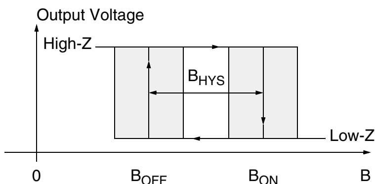
Fig. 4–10: Definition of magnetic switching points for the HAL 1507
