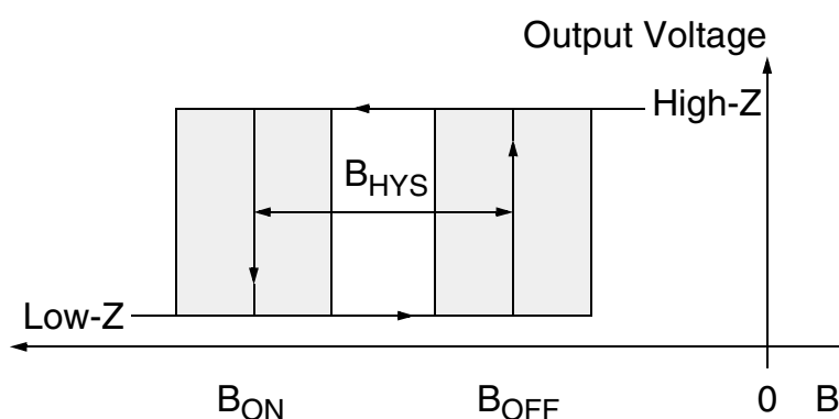
Fig. 4–11: Definition of magnetic switching points for the HAL 150y
