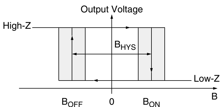
Fig. 4–7: Definition of magnetic switching points for the HAL 1502
