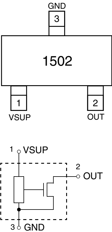
Fig. 4–5: Pin configuration
