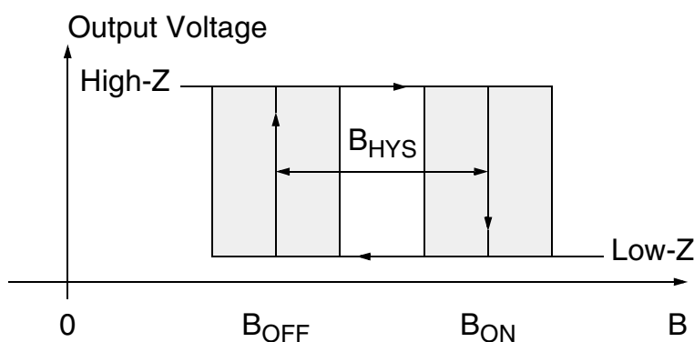
Fig. 4–9: Definition of magnetic switching points for the HAL 1506
