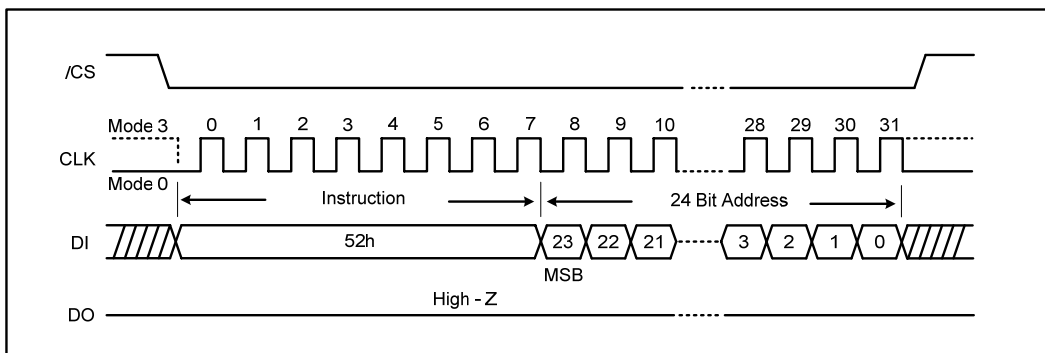
Figure 23a. 32KB Block Erase Instruction (SPI Mode)
