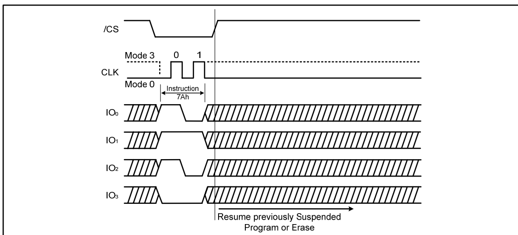
Figure 27b. Erase / Program Resume instruction (QPI Mode)
