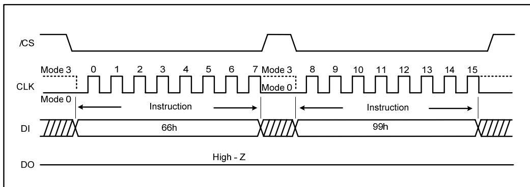
Figure 40a. Enable Reset and Reset Instruction (SPI Mode)
