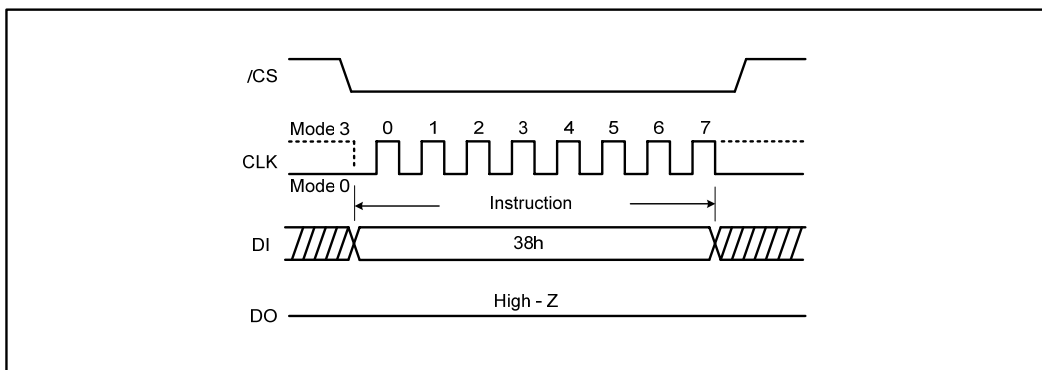
Figure 34. Enable QPI instruction (SPI Mode only)
