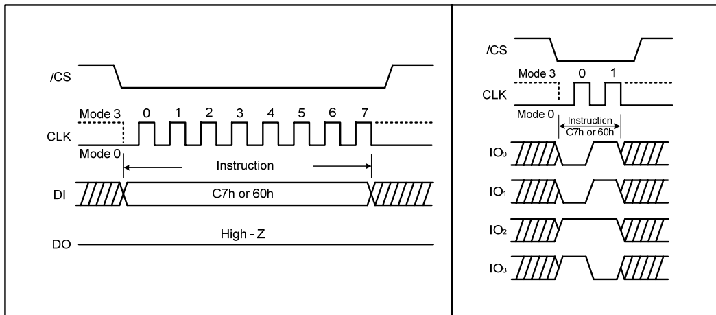
Figure 25. Chip Erase Instruction for SPI Mode (left) and QPI Mode (right)
