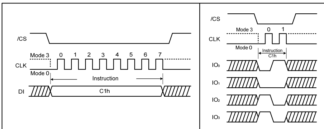
Figure 43. Exit Secured OTP instruction for SPI Mode (left) and QPI Mode (right)
