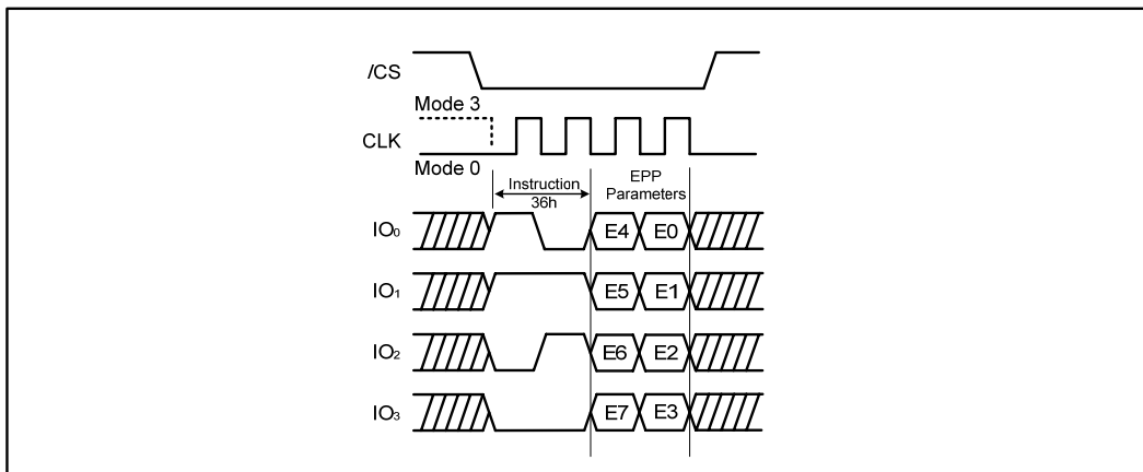
Figure 21 Set Enhance Page Program enable Instruction
