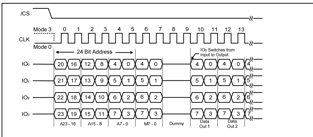
Figure 36b. Word Read Quad I/O instruction (Previous instruction set M7-0 = Ah, SPI Mode)
