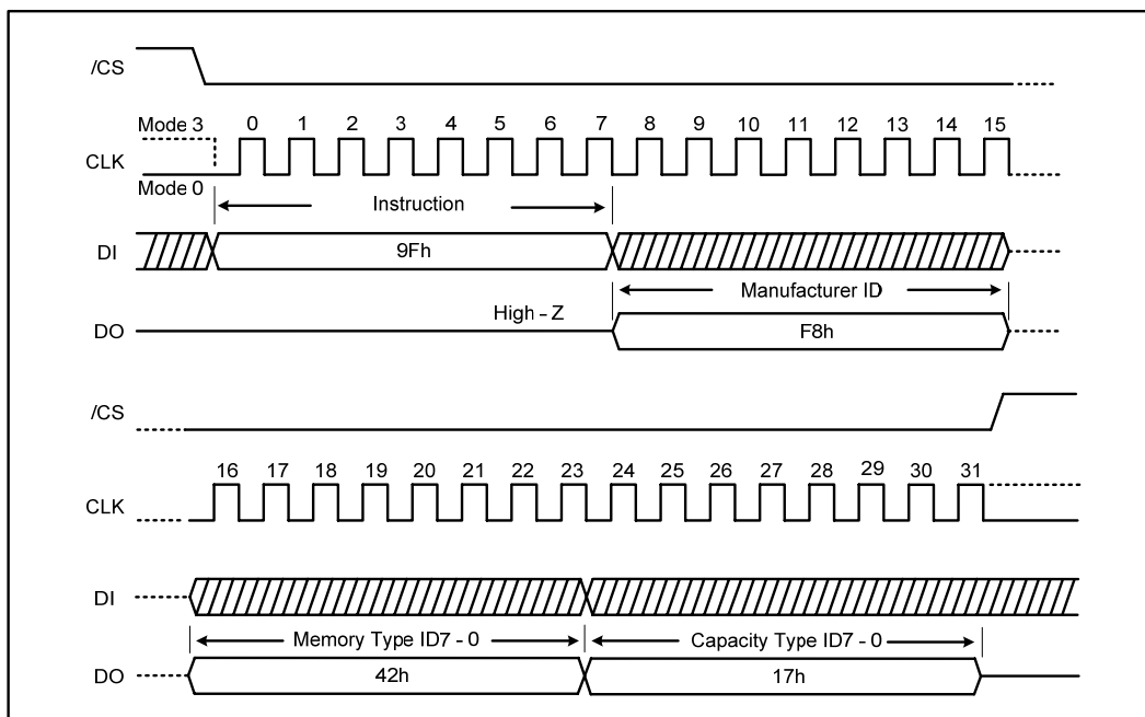
Figure 33a. Read JEDEC ID instruction (SPI Mode)
