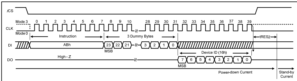
Figure 29c. Release power-down / Device ID Instruction (SPI Mode)
