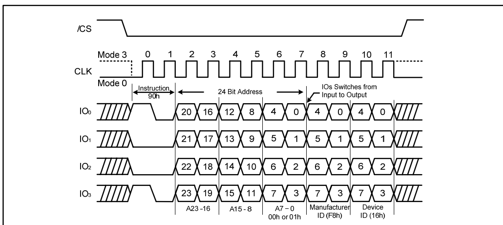
Figure 30b. Read Manufacturer/ Device ID instruction (QPI Mode)
