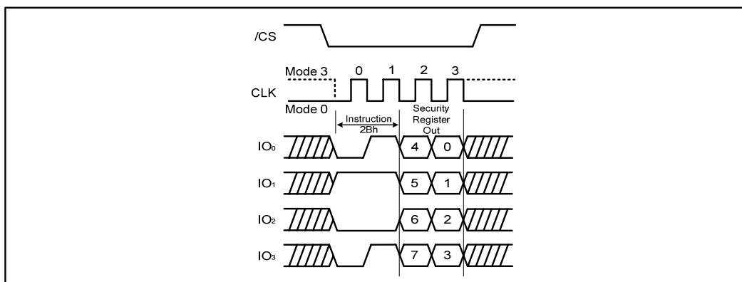
Figure 44b. Read Security Register instruction (QPI Mode)
