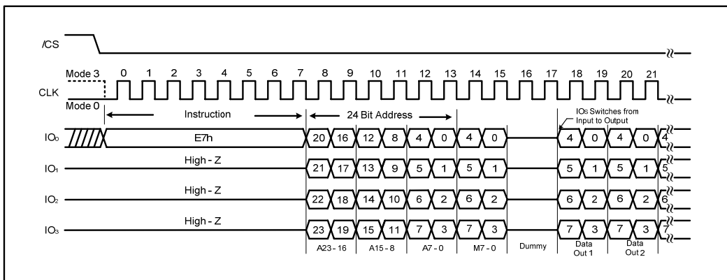
Figure 36a. Word Read Quad I/O instruction (Initial instruction or previous set M7-0 ≠ Ah, SPI Mode)
