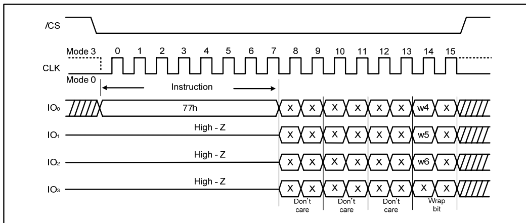
Figure 37. Set Burst with Wrap Instruction Sequence
