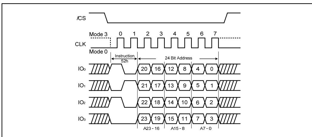
Figure 23b. 32KB Block Erase Instruction (QPI Mode)
