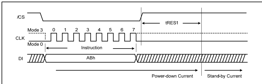
Figure 29a. Release power-down Instruction (SPI Mode)
