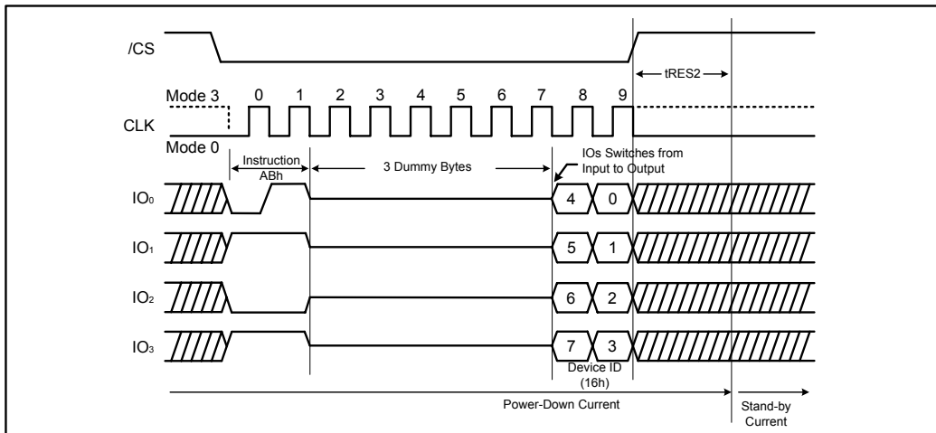
Figure 29d. Release power-down / Device ID Instruction (QPI Mode)
