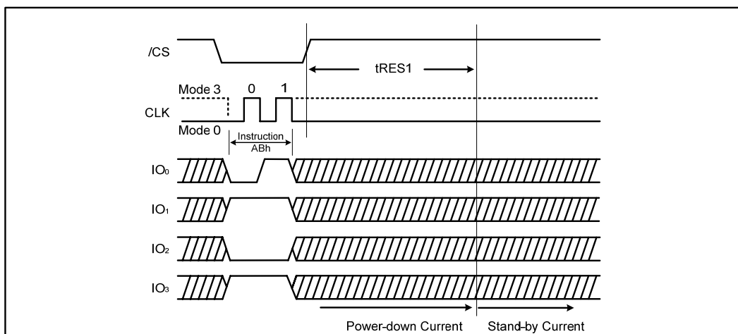
Figure 29b. Release power-down Instruction (QPI Mode)
