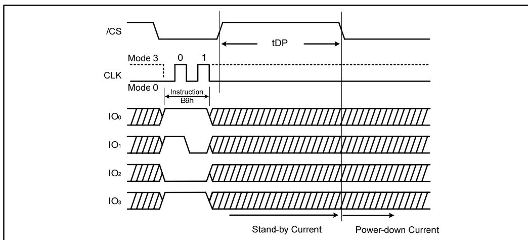
Figure 28b. Deep Power-down Instruction (QPI Mode)
