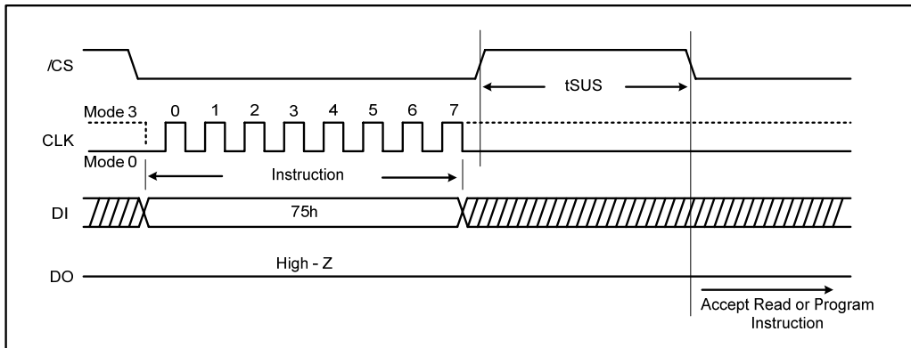
Figure 26a. Erase Suspend instruction (SPI Mode)
