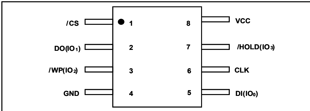
Figure 1a. Pin Assignments, 8-pin VSOP 208-mil
