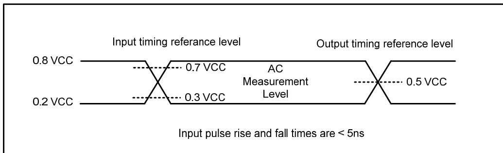
Figure 48. AC Measurement I/O Waveform
