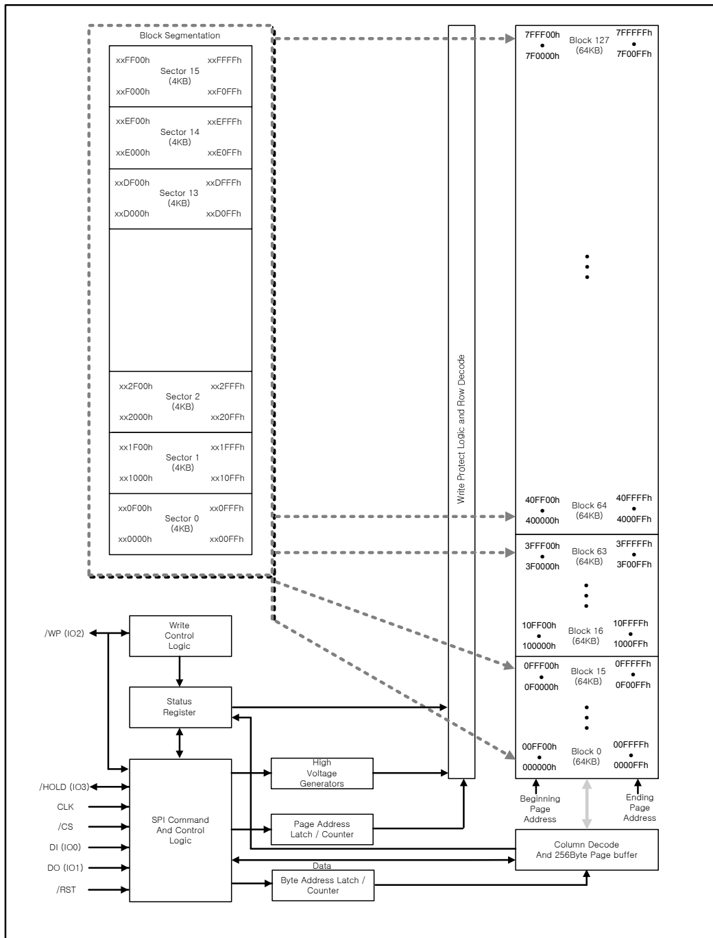
Figure 2. Block Diagram of FM25M64A
