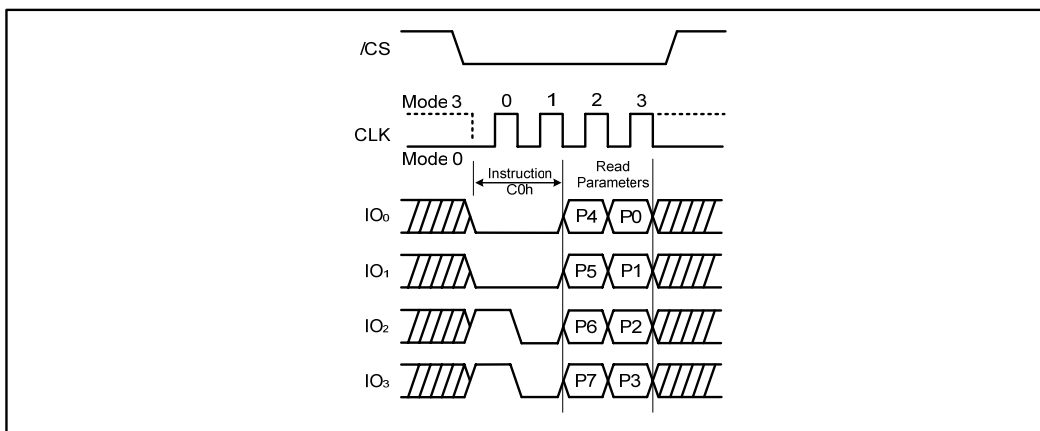
Figure 39. Set Read Parameters instruction (QPI Mode)
