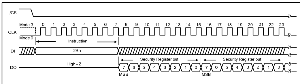
Figure 44a. Read Security Register instruction (SPI Mode)
