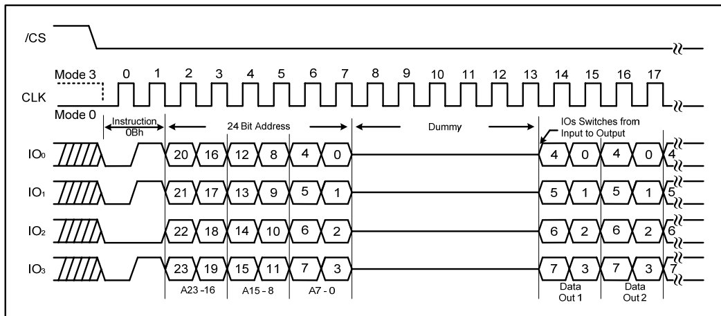
Figure 13c. Fast Read instruction (QPI Mode, 104MHz)
