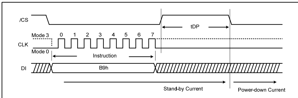
Figure 28a. Deep Power-down Instruction (SPI Mode)
