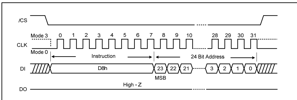
Figure 24a. 64KB Block Erase Instruction (SPI Mode)
