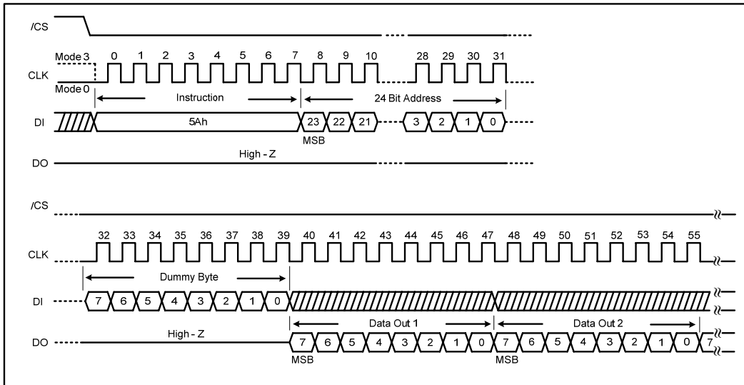
Figure 41. Read SFDP Register Instruction
