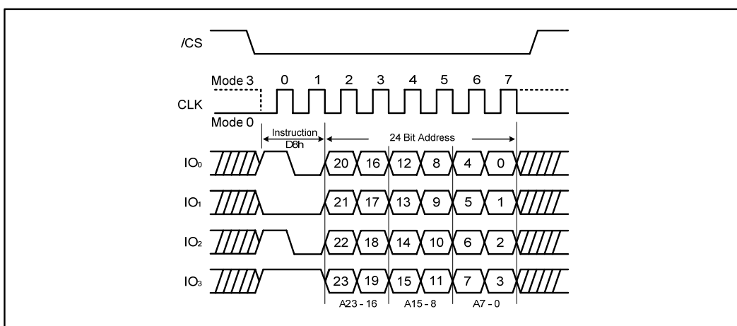
Figure 24b. 64KB Block Erase Instruction (QPI Mode)
