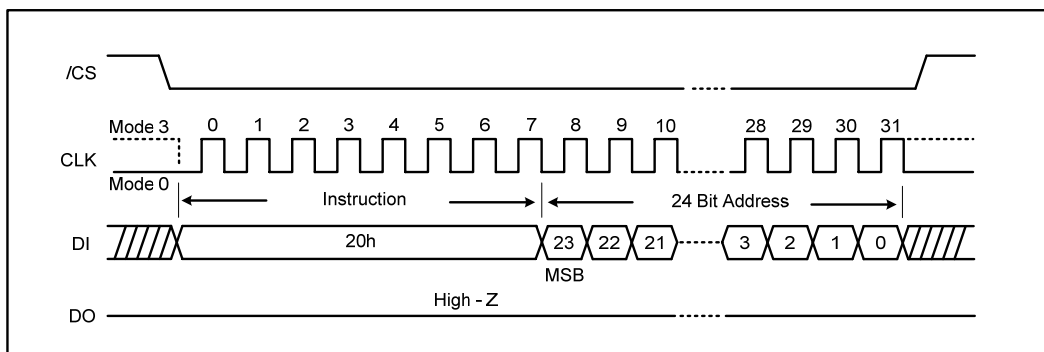
Figure 22a. Sector Erase Instruction (SPI Mode)
