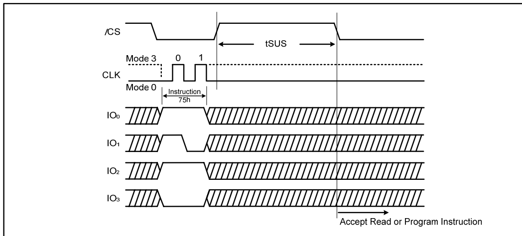
Figure 26b. Erase Suspend instruction (QPI Mode)
