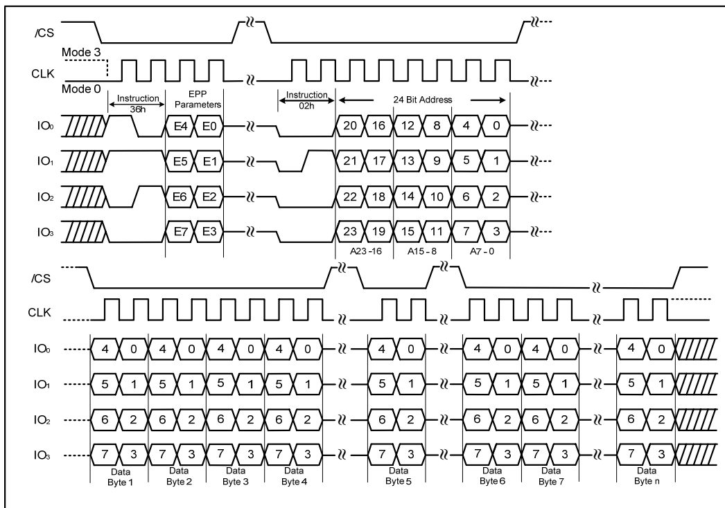
Figure 20. Enhance Page Program Instruction (QPI mode)
