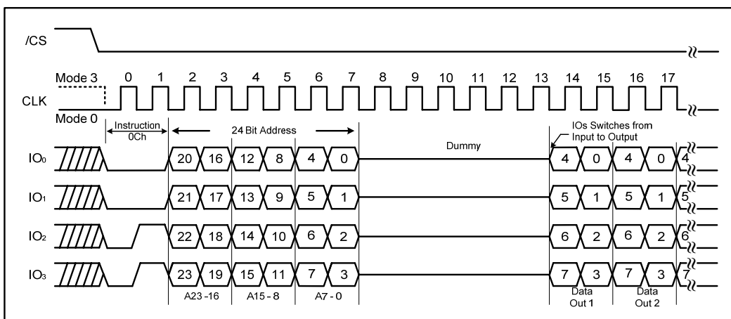
Figure 38b. Burst Read with Wrap instruction (QPI Mode, 104MHz)
