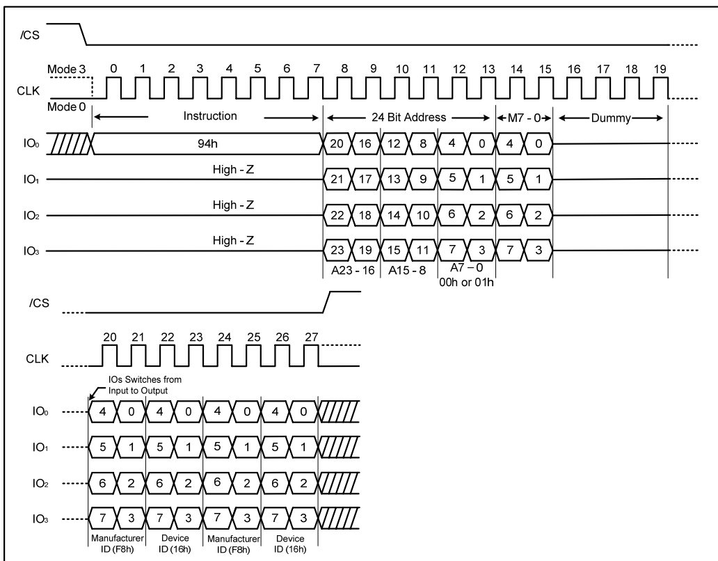
Figure 32. Read Quad Manufacturer/ Device ID Quad I/O instruction (SPI Mode)
