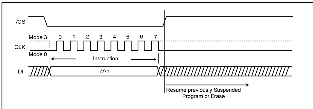
Figure 27a. Erase / Program Resume instruction (SPI Mode)
