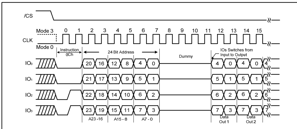
Figure 38a. Burst Read with Wrap instruction (QPI Mode, 80MHz)
