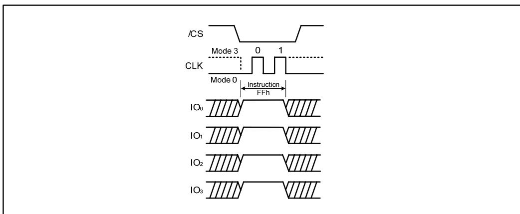
Figure 35. Disable QPI instruction for QPI mode
