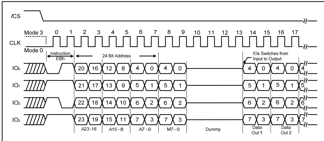
Figure 17d. Fast Read Quad I/O Instruction (Initial instruction or previous M_{7-0} \neq A_{xh} , QPI mode, 104MHz)
