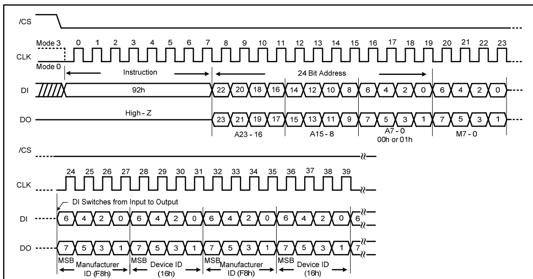
Figure 31. Read Dual Manufacturer/ Device ID Dual I/O instruction (SPI Mode)
