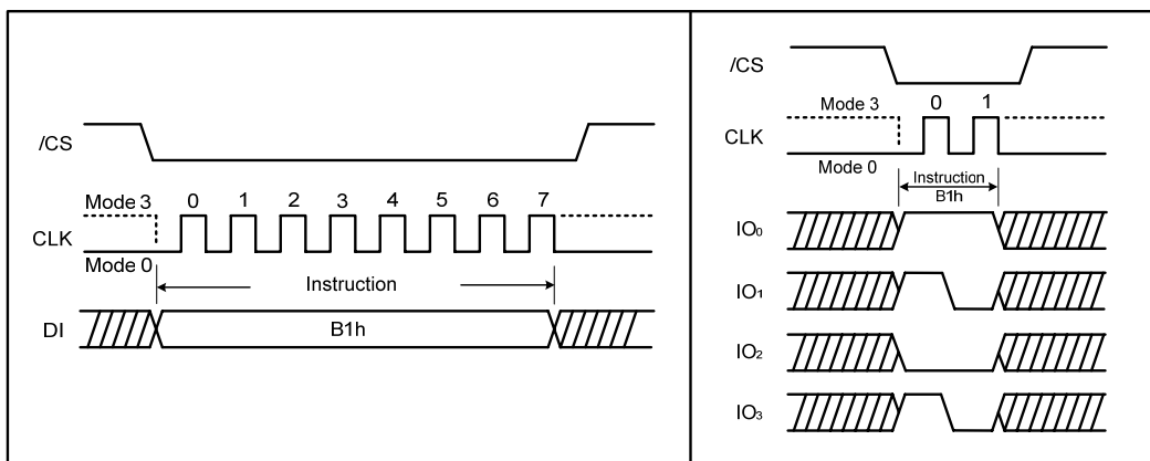
Figure 42. Enter Secured OTP instruction for SPI Mode (left) and QPI Mode (right)
