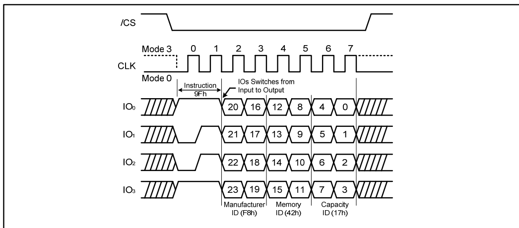
Figure 33b. Read JEDEC ID instruction (QPI Mode)
