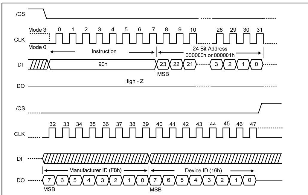
Figure 30a. Read Manufacturer/ Device ID instruction (SPI Mode)
