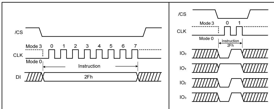
Figure 45. Write Security Register instruction for SPI Mode (left) and QPI Mode (right)
