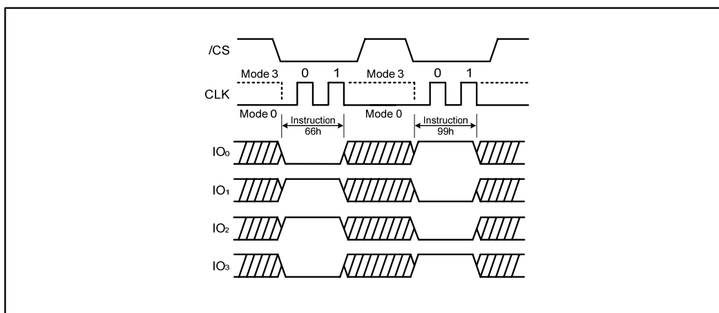
Figure 40b. Enable Reset and Reset Instruction (QPI Mode)
