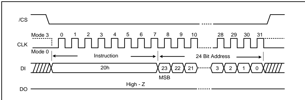
Figure 21a. Sector Erase Instruction (SPI Mode)
