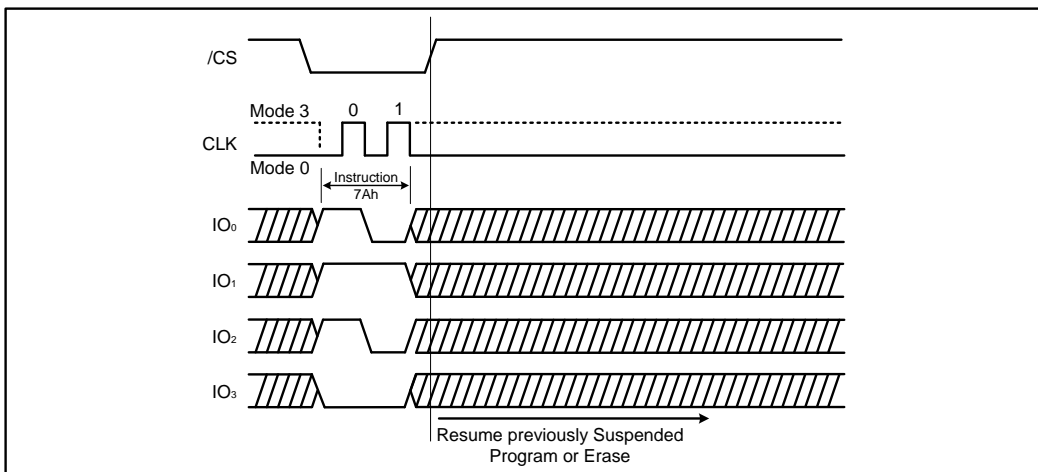
Figure 26b. Erase / Program Resume instruction (QPI Mode)
