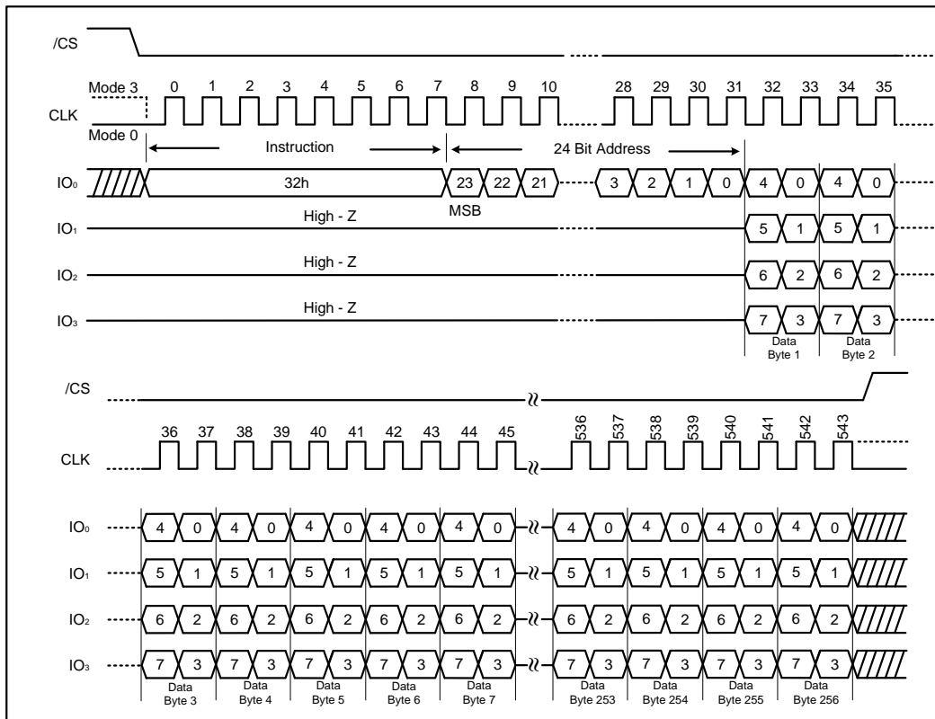
Figure 19. Quad Data Input Page Program Instruction
