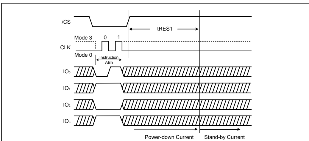
Figure 28b. Release power-down Instruction (QPI Mode)
