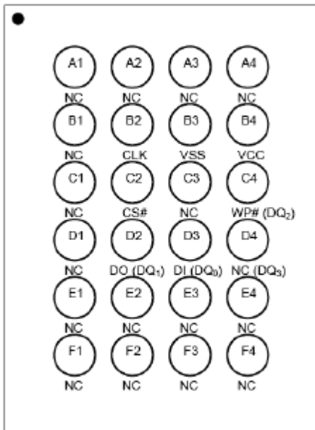
24 - Ball TFBGA
