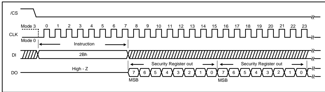
Figure 43a. Read Security Register instruction (SPI Mode)
