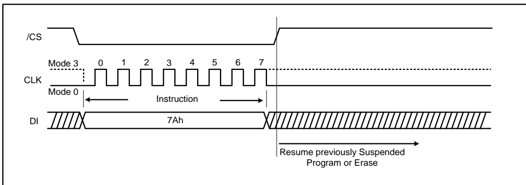
Figure 26a. Erase / Program Resume instruction (SPI Mode)
