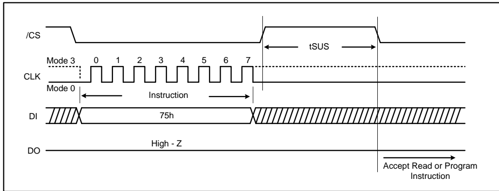
Figure 25a. Erase Suspend instruction (SPI Mode)
