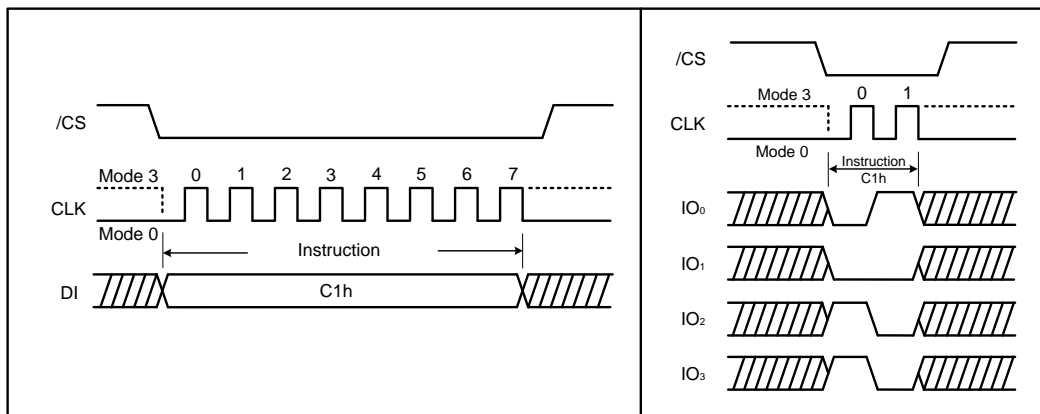
Figure 42. Exit Secured OTP instruction for SPI Mode (left) and QPI Mode (right)
