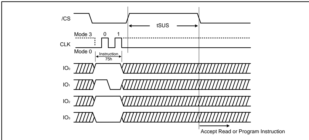
Figure 25b. Erase Suspend instruction (QPI Mode)
