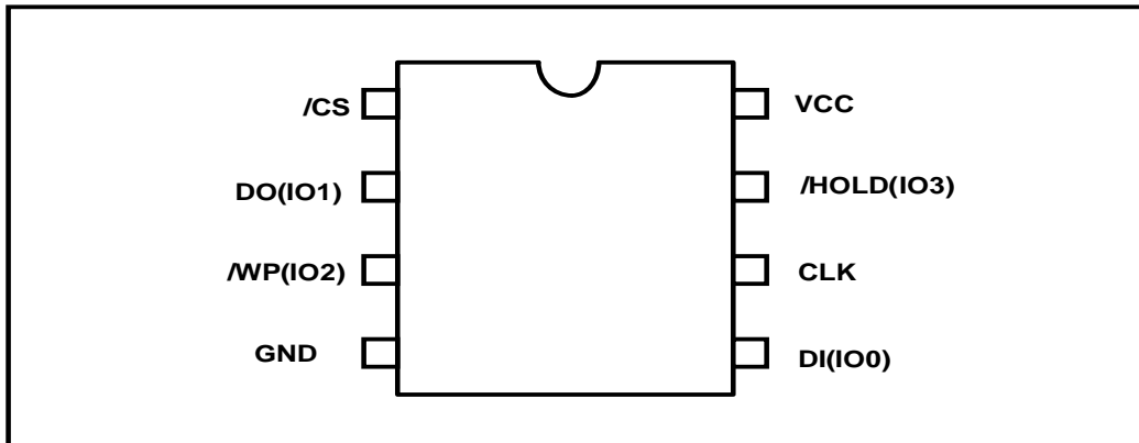
Figure 1c. Assignments, 8-pin PDIP 300-mil
