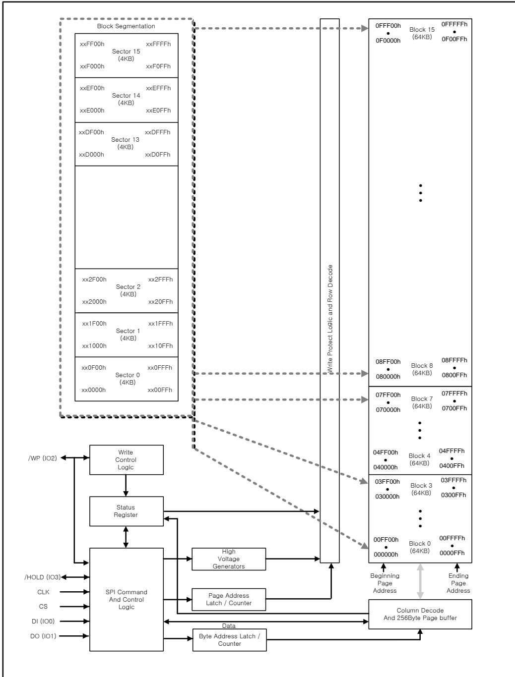
Figure 2. Block Diagram of FM25M08A
