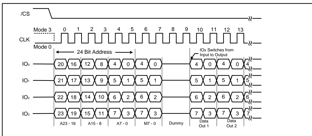
Figure 35b. Word Read Quad I/O instruction (Previous instruction set M7-0 = Ah, SPI Mode)
