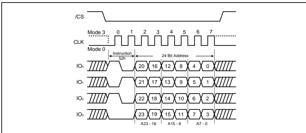
Figure 22b. 32KB Block Erase Instruction (QPI Mode)
