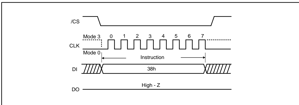
Figure 33. Enable QPI instruction (SPI Mode only)
