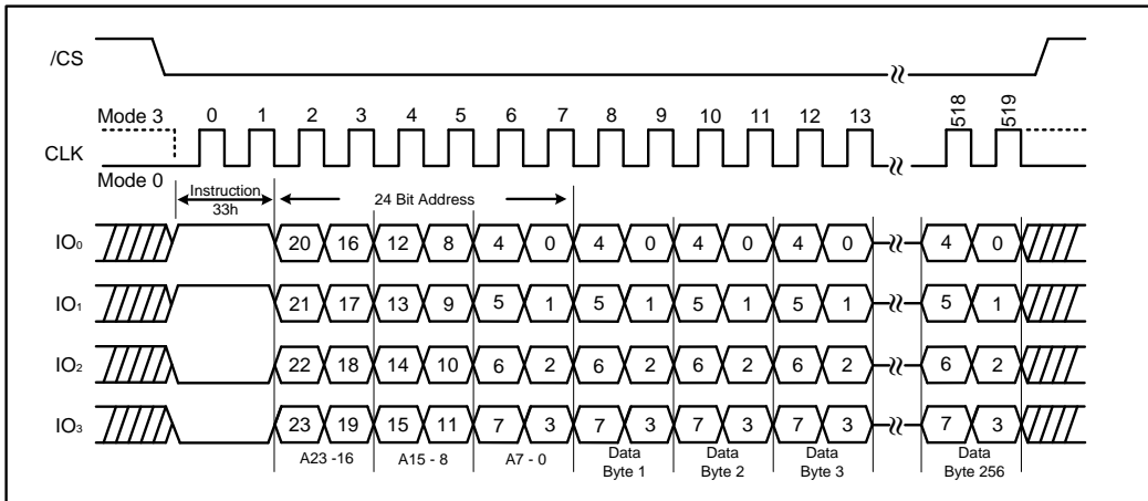
Figure 20b. Quad Page Program Instruction (QPI mode)
