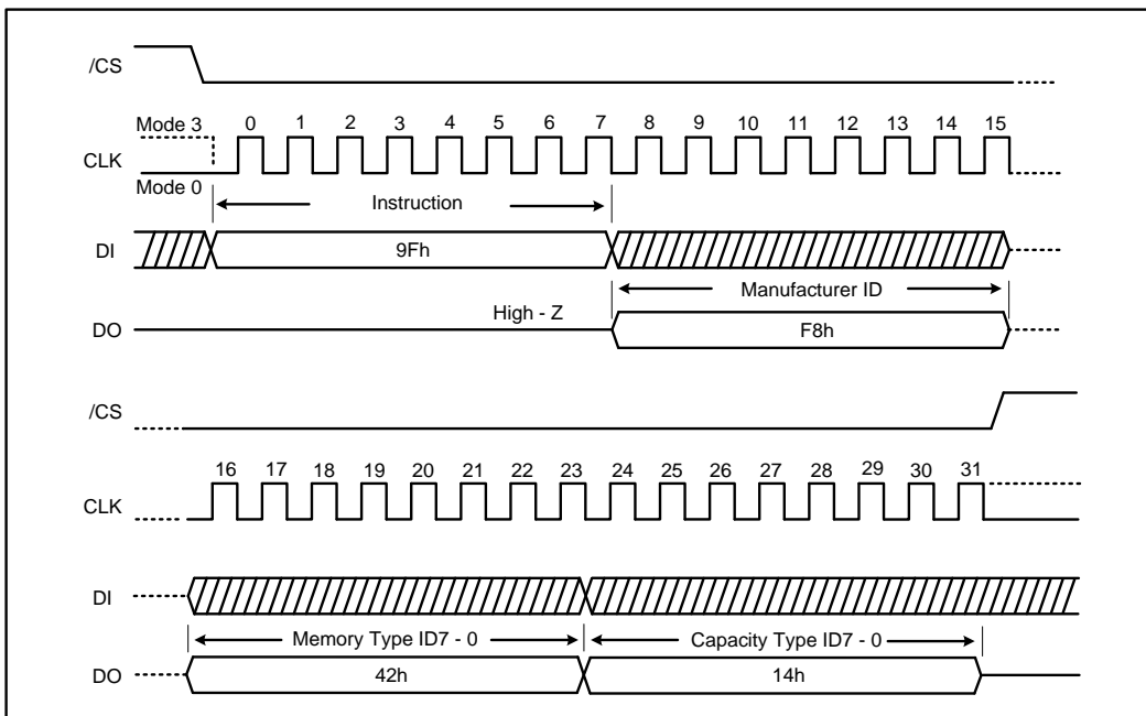
Figure 32a. Read JEDEC ID instruction (SPI Mode)
