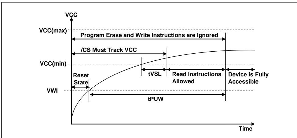
Figure 45. Power-up Timing and Voltage Levels
