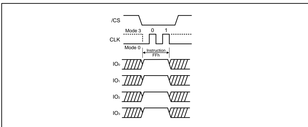
Figure 34. Disable QPI instruction for QPI mode
