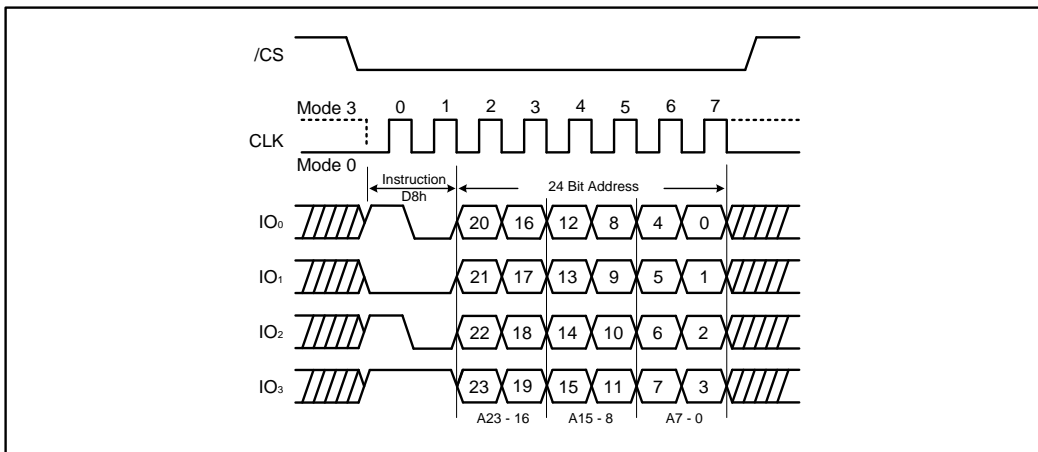
Figure 23b. 64KB Block Erase Instruction (QPI Mode)
