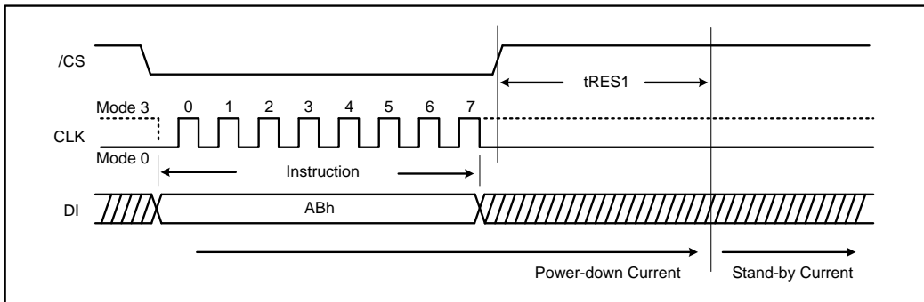
Figure 28a. Release power-down Instruction (SPI Mode)
