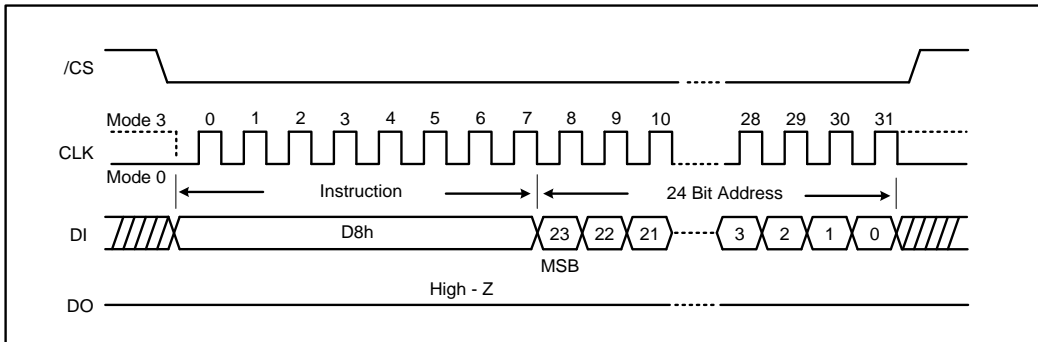
Figure 23a. 64KB Block Erase Instruction (SPI Mode)
