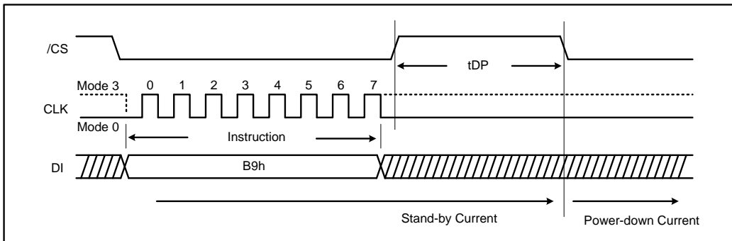
Figure 27a. Deep Power-down Instruction (SPI Mode)
