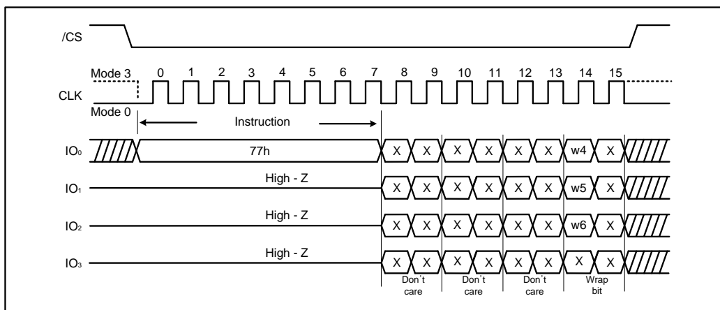
Figure 36. Set Burst with Wrap Instruction
