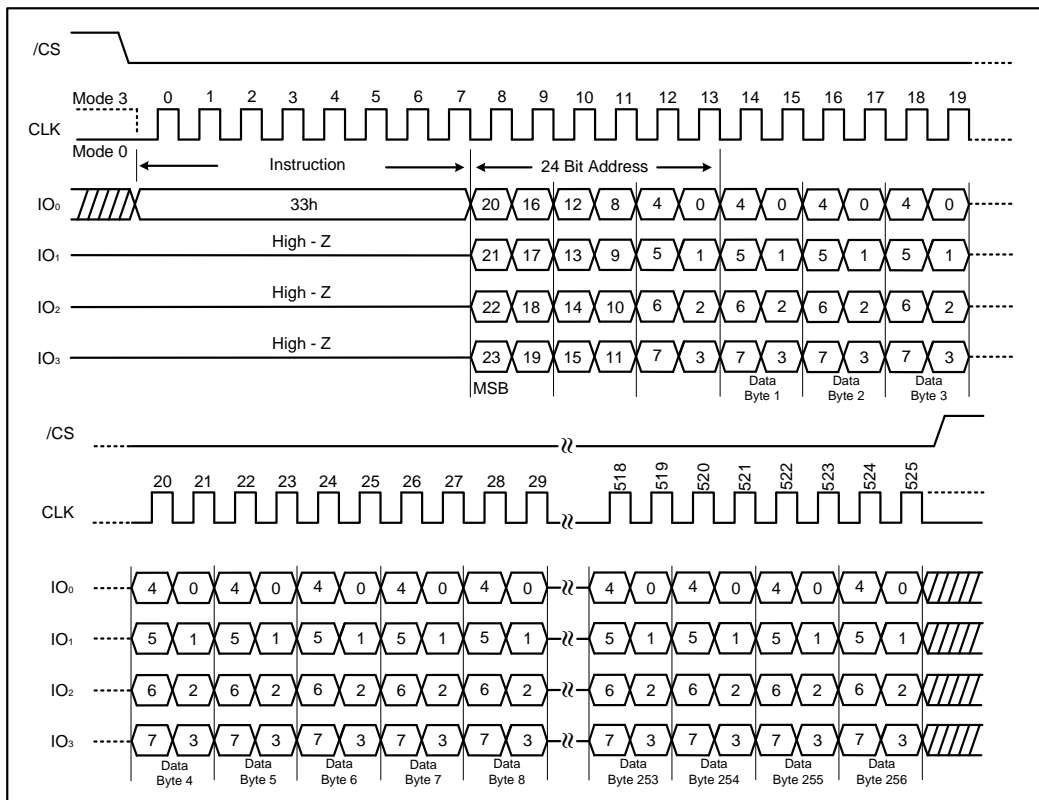
Figure 20a. Quad Page Program Instruction (SPI mode)
