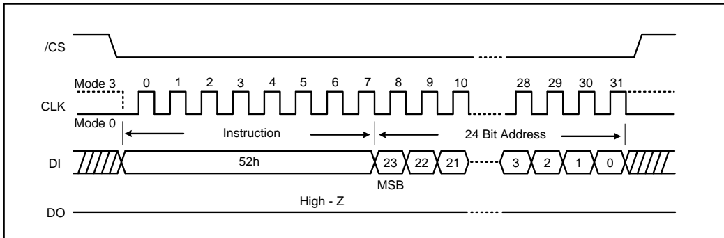
Figure 22a. 32KB Block Erase Instruction (SPI Mode)
