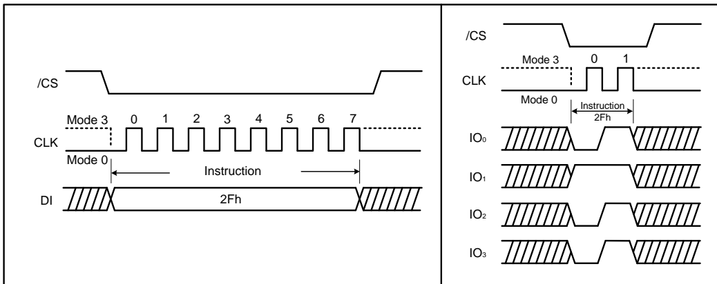
Figure 44. Write Security Register instruction for SPI Mode (left) and QPI Mode (right)
