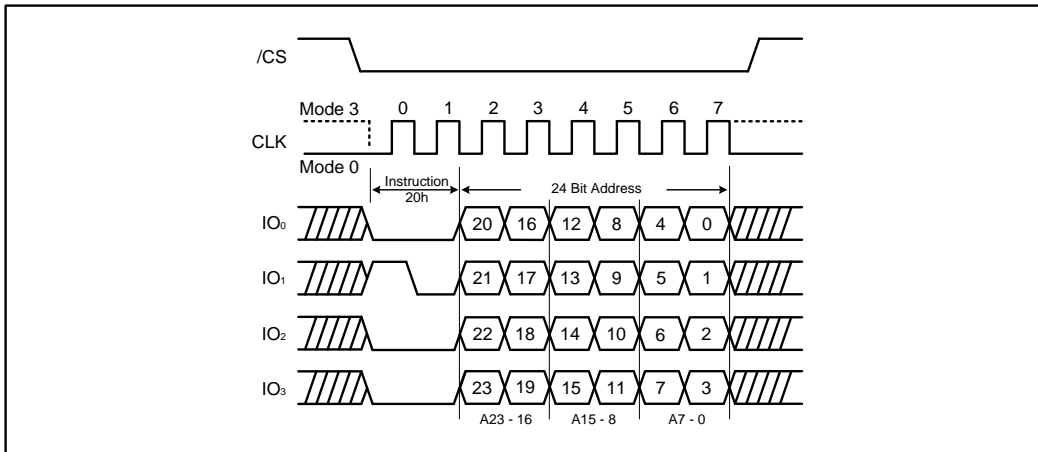
Figure 21b. Sector Erase Instruction (QPI Mode)
