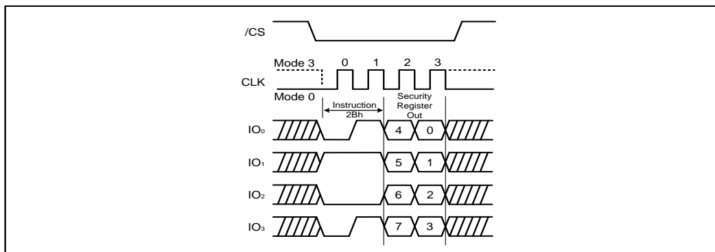
Figure 43b. Read Security Register instruction (QPI Mode)
