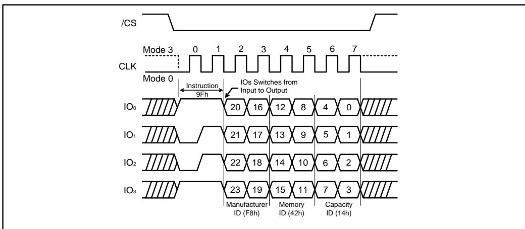
Figure 32b. Read JEDEC ID instruction (QPI Mode)
