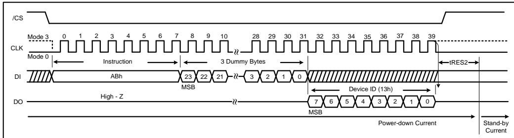
Figure 28c. Release power-down / Device ID Instruction (SPI Mode)
