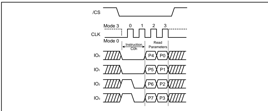
Figure 38. Set Read Parameters instruction (QPI Mode)
