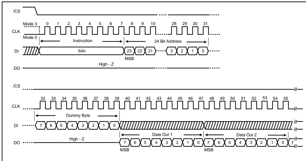
Figure 40. Read SFDP Register Instruction
