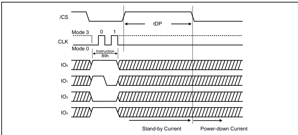
Figure 27b. Deep Power-down Instruction (QPI Mode)
