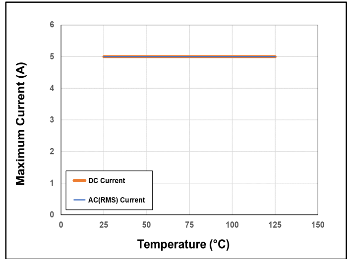
Figure 12. CT110FDx Maximum Current De-rating Curve
