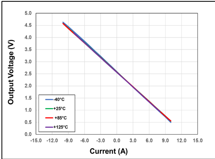
Figure 13. CT110PDx Output Voltage vs. Current vs. Temperature
