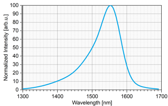
Optical Spectrum
