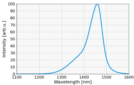
Optical Spectrum
