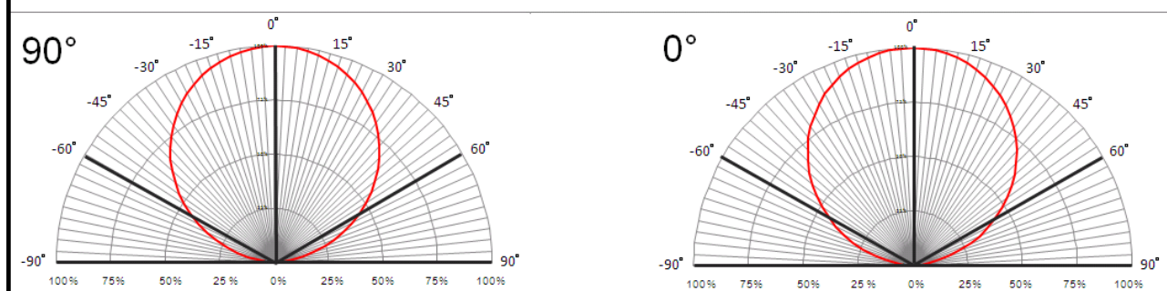
Directive Characteristics
