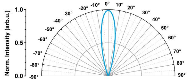
Radiation Pattern
