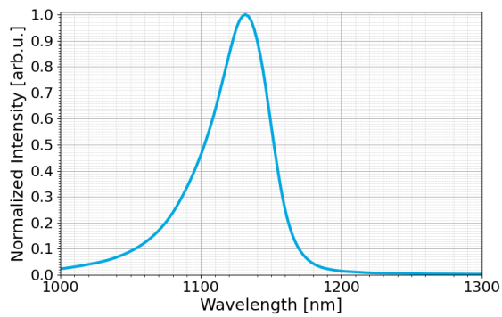
Optical Spectrum
