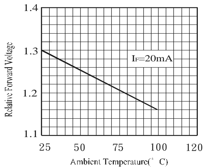
Forward Voltage vs Ambient Temperature(°C)
