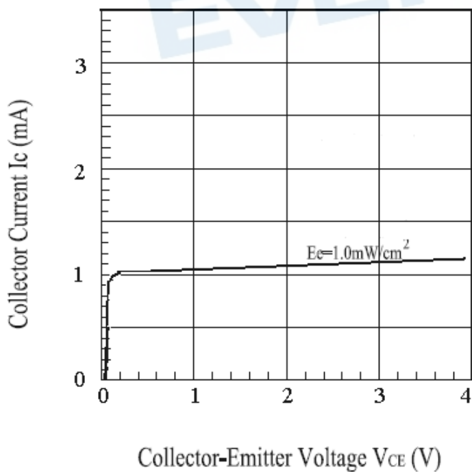
Fig.3 Collector Current vs.
