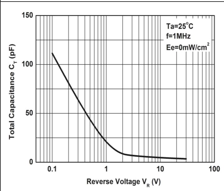
Terminal Capacitance vs. Reverse Voltage
