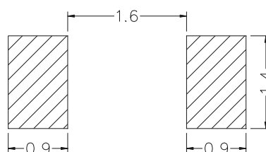
Recommended Soldering Pattern for Side Looker
