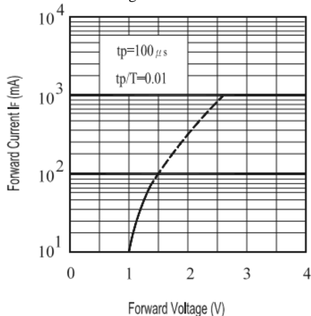
Fig.4 Forward Current
