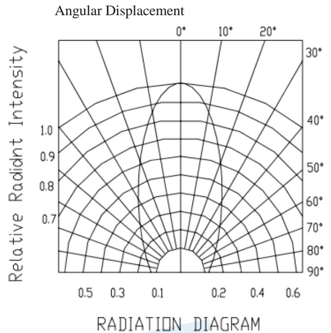
Fig.6 Relative Radiant Intensity vs.
