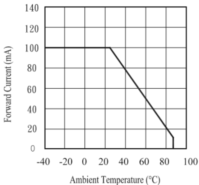
Fig.1 Forward Current vs.
