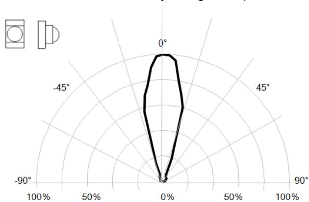
Relative Radiant Intensity vs Angular Displacement
