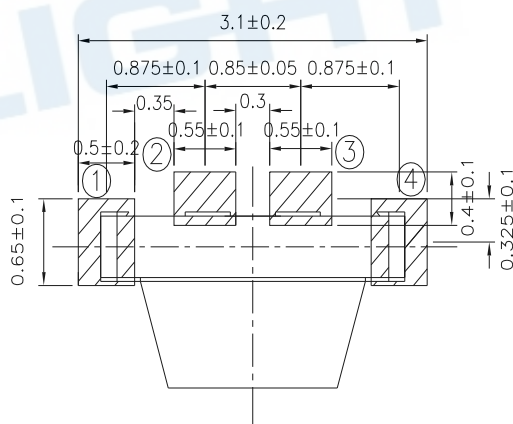
Recommend Soldering Pad
