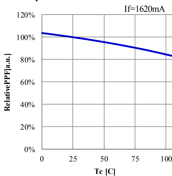
Case Temperature vs. Relative PPF
