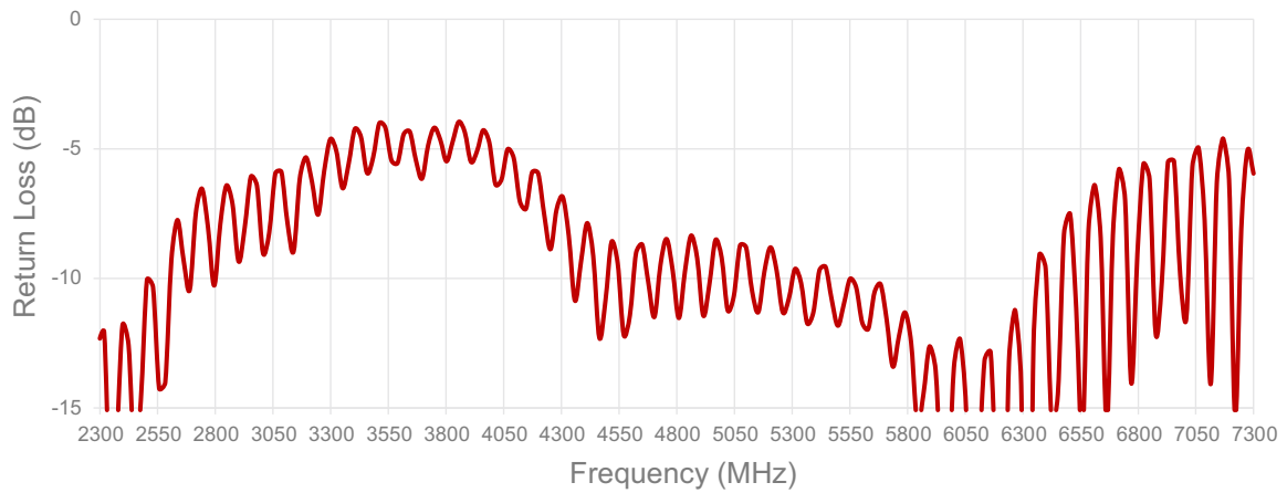
Cable 4: 2.4/5.0/6.0 GHz ISM
