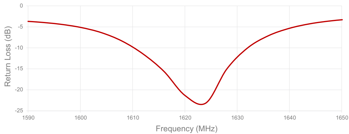
Cable 5: IRIDIUM
