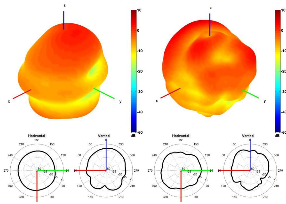
750 and 2500 MHz Radiation pattern
