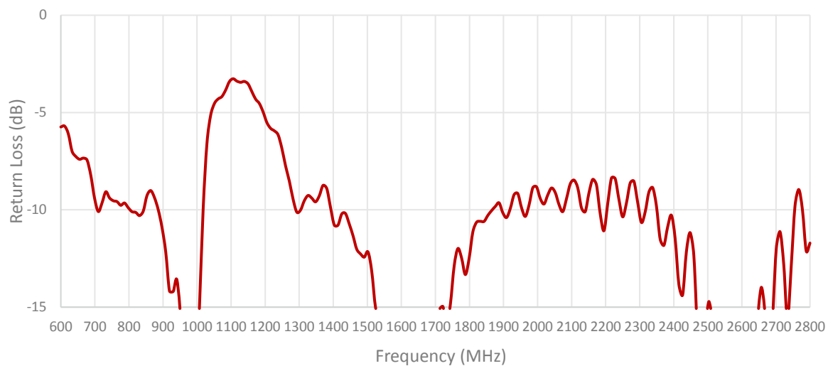
Cable 1: CELLULAR/LTE
