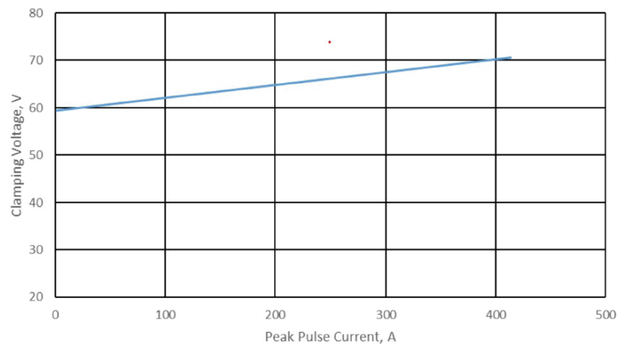
FIGURE 2 SM30KWE48CA CLAMPING VOLTAGE VS PEAK PULSE CURRENT 10/1000 \mu s
