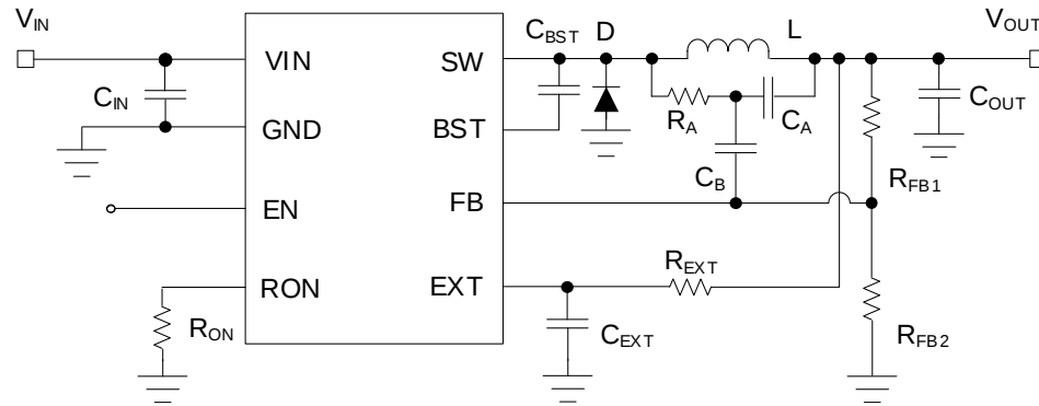
Figure 2 Typical Application Diagram of SC81A10E with 4µA Low Quiescent current
