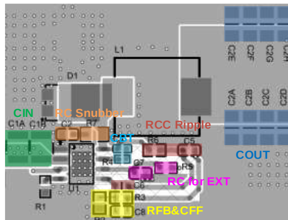
Figure 9 PCB layout Example
