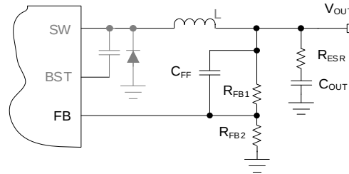
Figure 6 Type 2 Ripple Generated by R_{ESR} & C_{FF}
