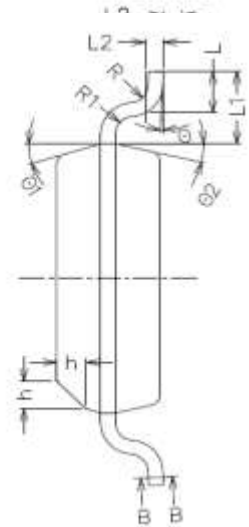
COMMON DIMENSIONS (UNITS OF MEASURE=MILLIMETER)
