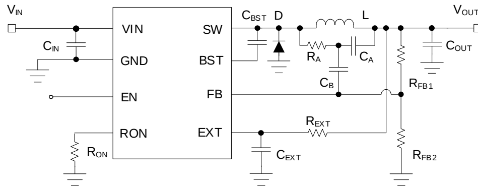
Figure 2 Typical Application Diagram of SC81B30E with 4µA Low Quiescent current
