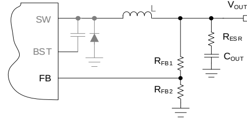
Figure 5 Type 1 Ripple Generated by R_{ESR}
