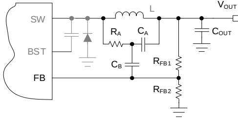
Figure 7 Type 3 Ripple Generated by RCC
