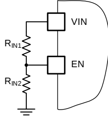
Figure 4 UVLO Threshold Programming
