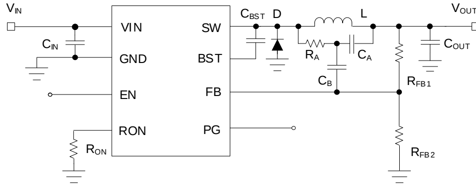
Figure 1 Typical Application Diagram of SC81B30 with Power Good Indicator and 10µA Low Quiescent current
