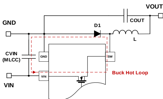
Figure 8 Minimizing the Hot Loop Helps Mitigate EMI
