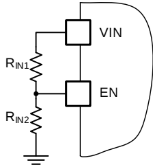
Figure.6 UVLO Threshold Programming
