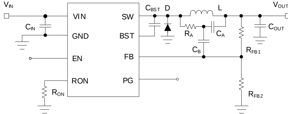
Figure 1 Typical Application Diagram of SC81B20 with Power Good Indicator and 10µA Low Quesicent current
