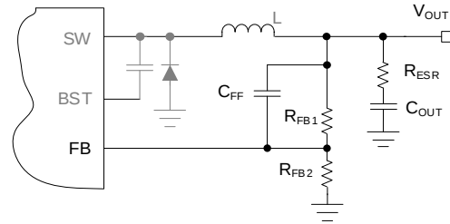
Figure.4 Type 2 Ripple Generated by R_{ESR} & C_{FF}
