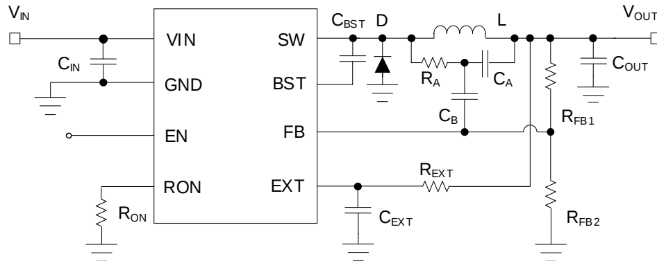
Figure 2 Typical Application Diagram of SC81B20E with 4µA Low Quesicent current
