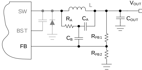
Figure.5 Type 3 Ripple Generated by RCC
