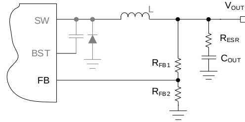
Figure.3 Type 1 Ripple Generated by R_{ESR}
