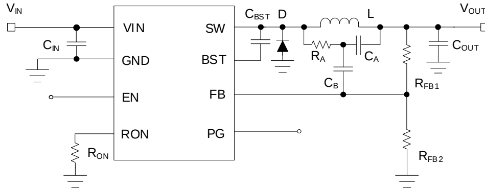
Figure 1 Typical Application Diagram of SC81B10 with Power Good Indicator and 10µA Low Quiescent current
