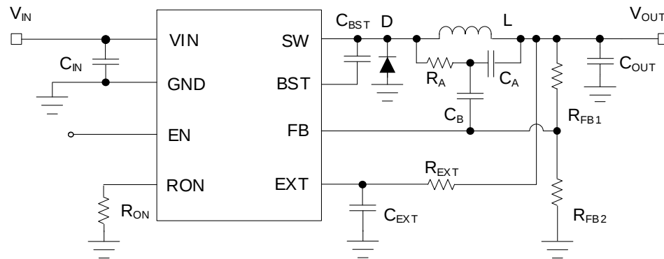
Figure 2 Typical Application Diagram of SC81B10E with 4µA Low Quiescent current
