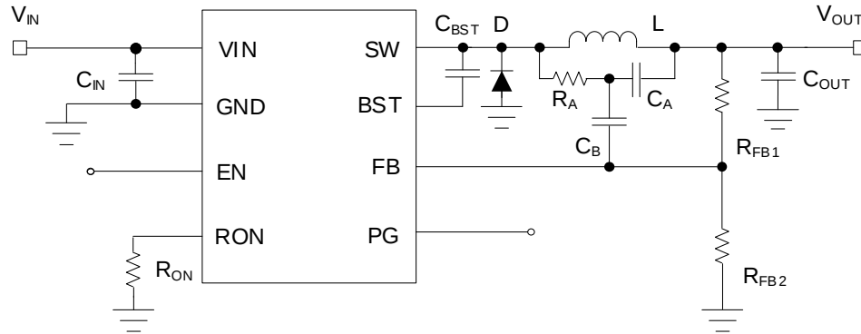
Figure 1 Typical Application Diagram of SC81A50 with Power Good Indicator and 10µA Low Quiescent current
