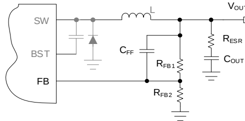
Figure 6 Type 2 Ripple Generated by R_{ESR} & C_{FF}
