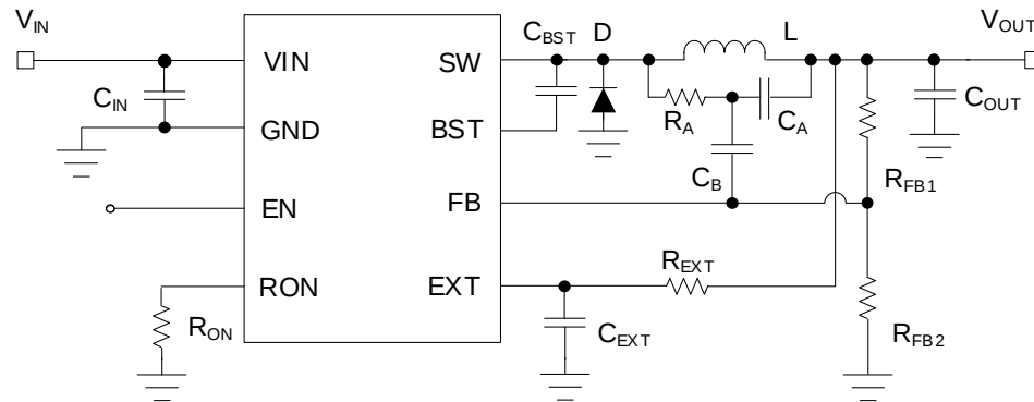
Figure 2 Typical Application Diagram of SC81A30E with 4µA Low Quiescent current
