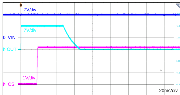
Figure 12-9 Short-to-battery Protection(Latch)
