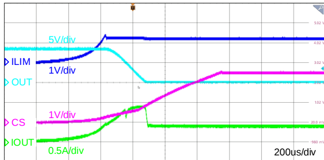
Figure 12-7 Current Limit
