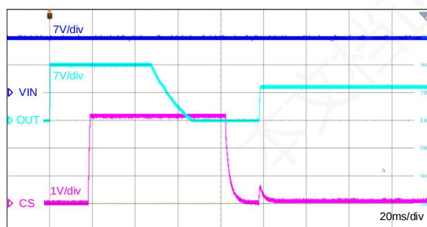
Figure 12-10 Short-to-battery Protection(Retry)
