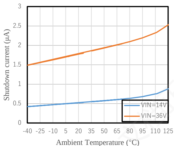
Figure 8-2 Shutdown current vs ambient temperature
