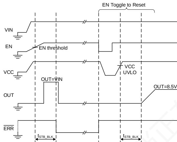
Figure 11-3 Short-to-battery Detection Window
