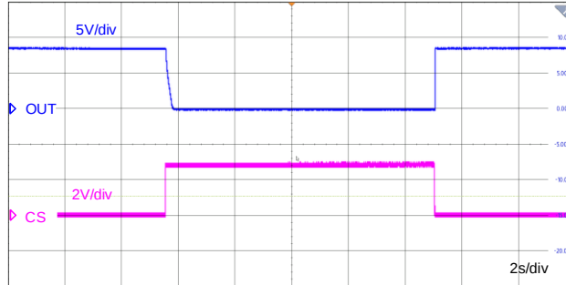
Figure 12-8 Thermal Shutdown Protection
