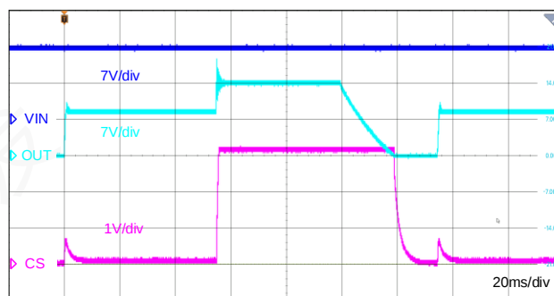
Figure 12-12 Reverse Current Protection(Retry)
