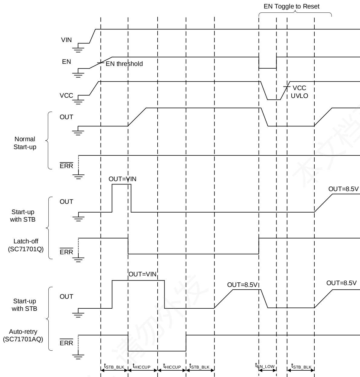
Figure 10-1 Timing Sequence for Start-up, Latch-off and Auto-retry
