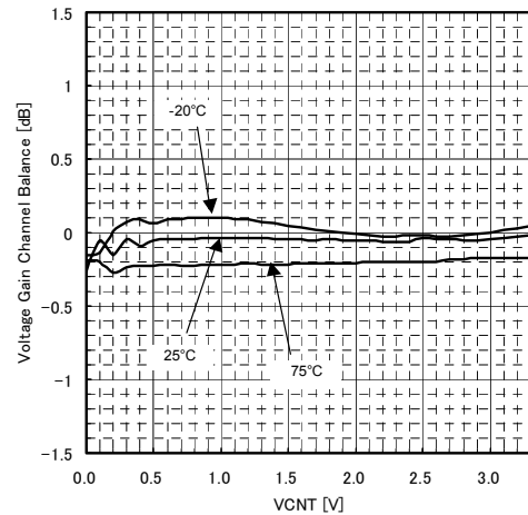
Voltage Gain Channel Balance vs. Control Voltage (Ambient Temperature) V_+ = 9V , V_{in} = -20dBV , f = 1kHz , R_L = 100\Omega
