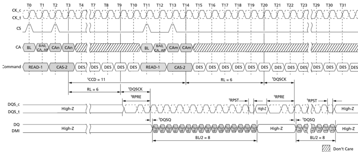
Figure 43. Consecutive READ: t_{CCD} = MIN + 3 , Preamble = Toggle, 0.5nCK Postamble
