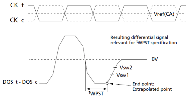
Figure 24. Method for Calculating tWPST Transitions and Endpoints
