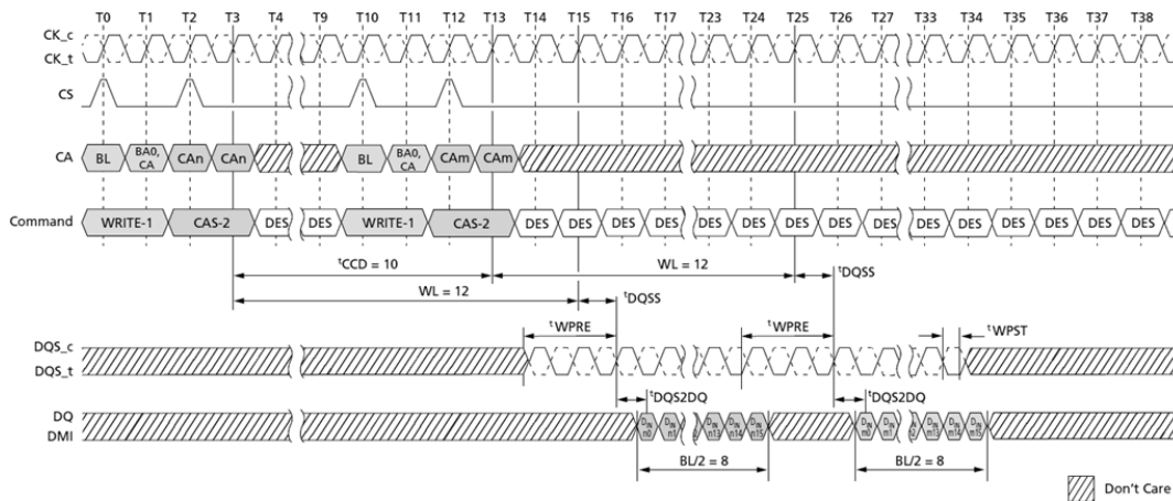
Figure 51. Consecutive WRITE: t_{CCD} = \text{MIN} + 2, 0.5nCK Postamble
