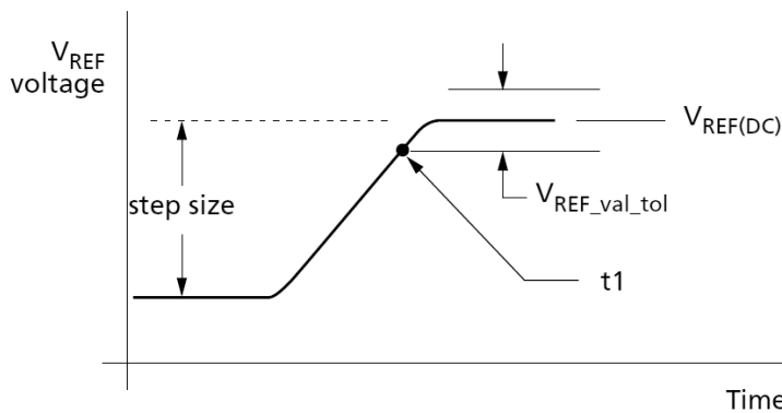
Figure 95. V_{REF(CA)} Single-Step Increment
