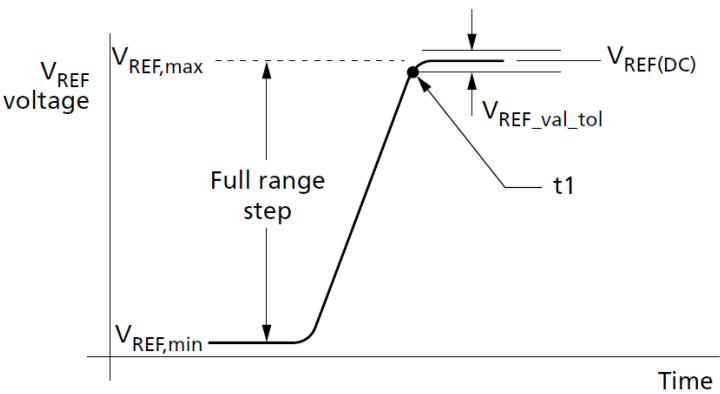
Figure 104. V_{REF(DQ)} Full Step from V_{REF,min} to V_{REF,max}
