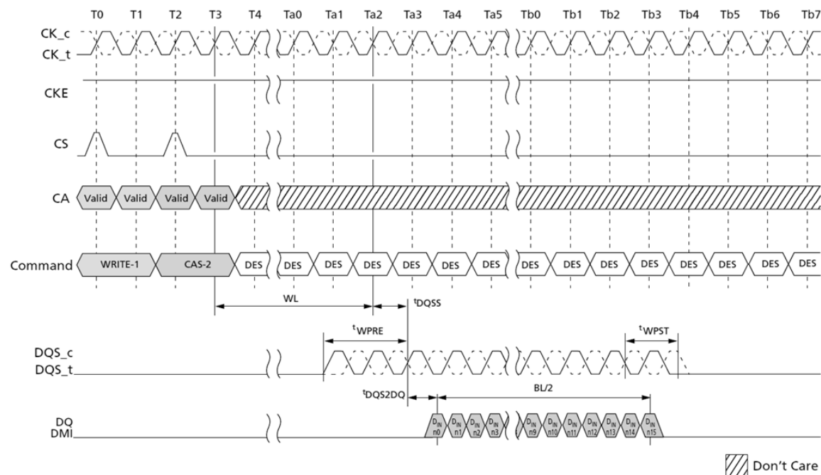
Figure 11. DQS Write Preamble and Postamble – 1.5nCK Postamble
