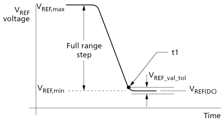
Figure 98. V_{REF(CA)} Full Step from V_{REF,max} to V_{REF,min}
