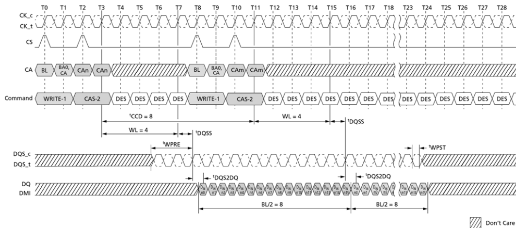
Figure 46. Seamless WRITE: t_{CCD} = \text{MIN} , 0.5nCK Postamble
