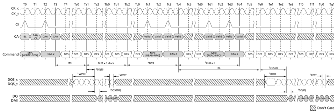
Figure 121. MPC[WRITE-FIFO]-to-MPC[READ-FIFO] Timing
