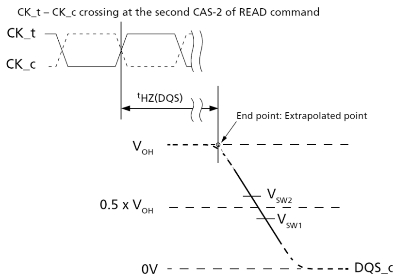
Figure 17. t_{HZ}(DQS) Method for Calculating Transitions and Endpoint
