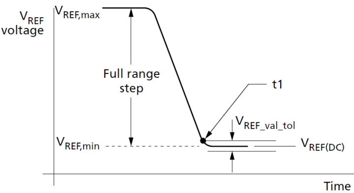
Figure 105. V_{REF(DQ)} Full Step from V_{REF,max} to V_{REF,min}
