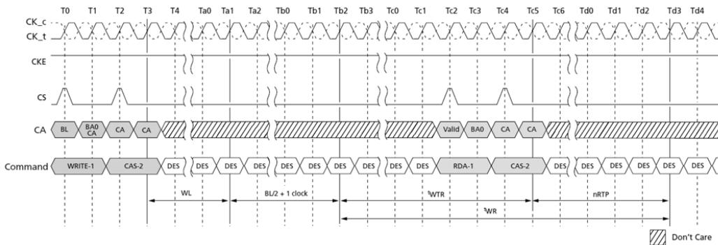
Figure 63. Delay Time From WRITE-to-READ with Auto Precharge
