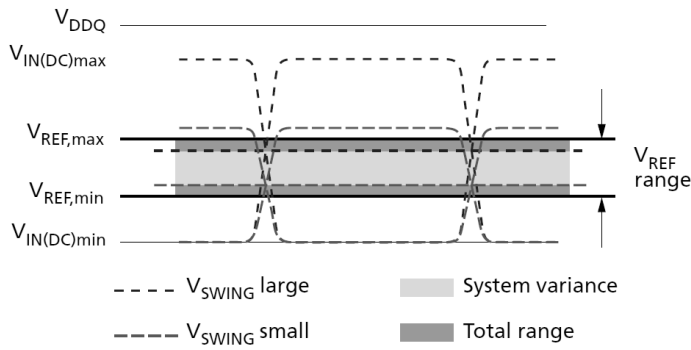
Figure 188. V_{REF} Operating Range ( V_{REF,max} , V_{REF,min} )
