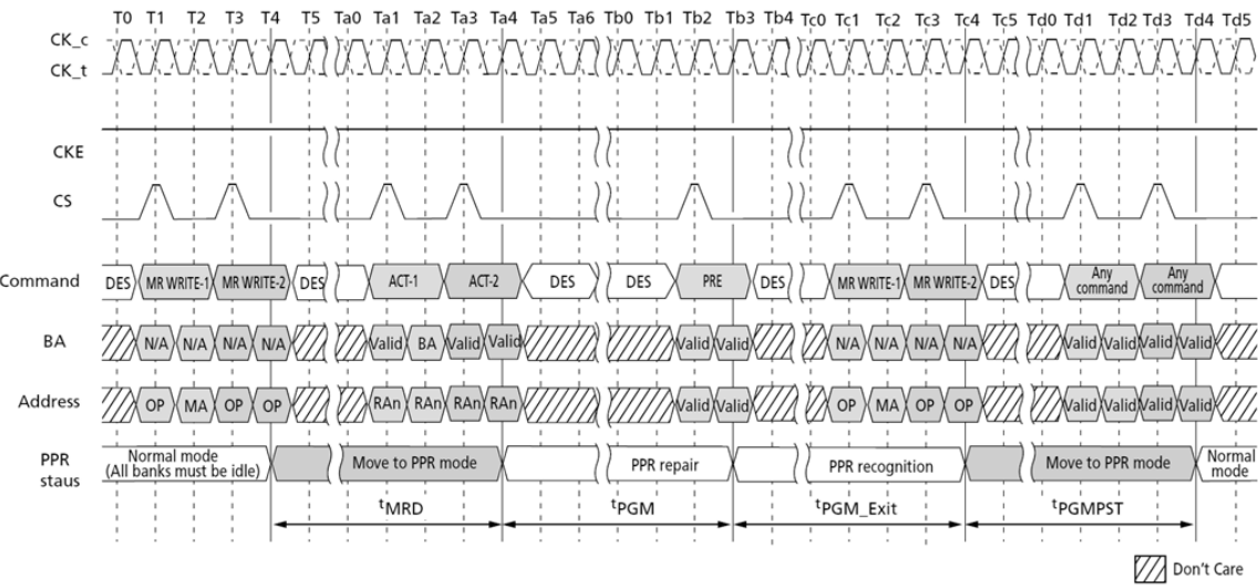
Figure 139. Post-Package Repair Timing
