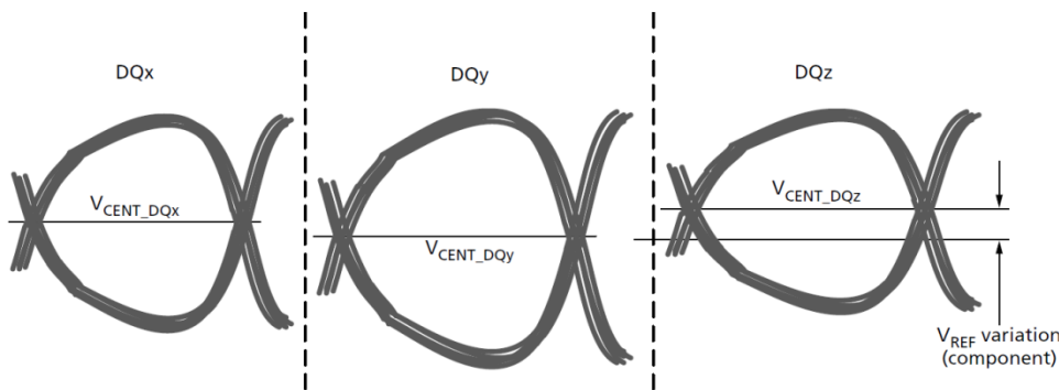
Figure 168. Across Pin V_{REF} DQ Voltage Variation
