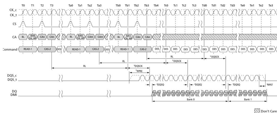
Figure 14. Seamless Burst Read
