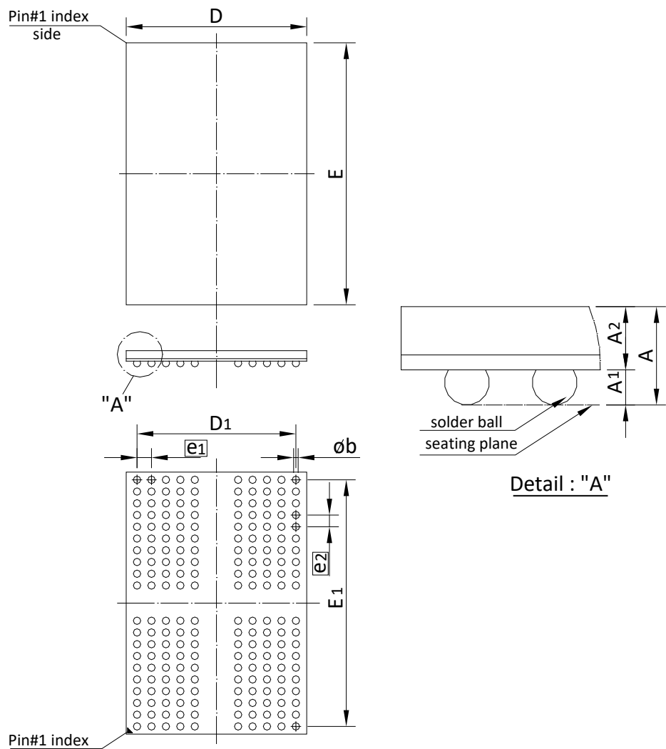
Figure 205. 200-BALL (10x14.5 mm)
