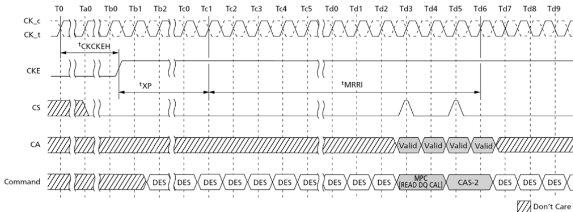
Figure 119. MPC[READ DQ CALIBRATION] Following Power-Down State
