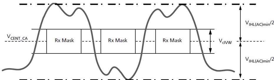
Figure 165. CA V_{IHL\_AC} Definition (for Each Input Pulse)
