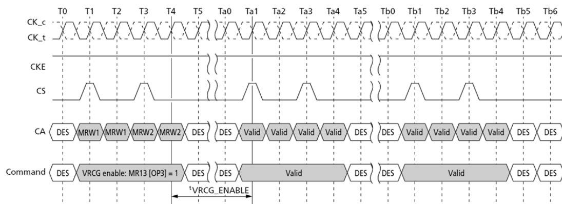
Figure 90. VRCG Enable Timing
