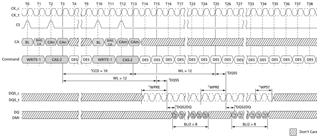
Figure 52. Consecutive WRITE: t_{CCD} = \text{MIN} + 2, 1.5nCK Postamble
