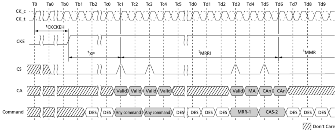
Figure 88. MRR Following Power-Down
