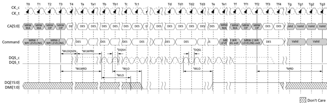
Figure 111. Write Leveling Timing – t_{DQSL}(\text{MIN})
