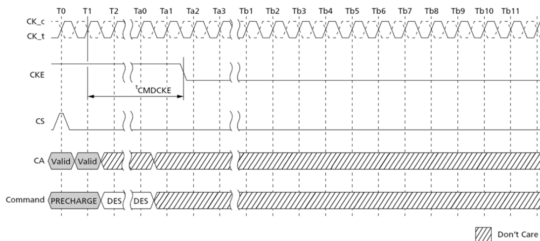
Figure 81. PRECHARGE Command to Power-Down Entry
