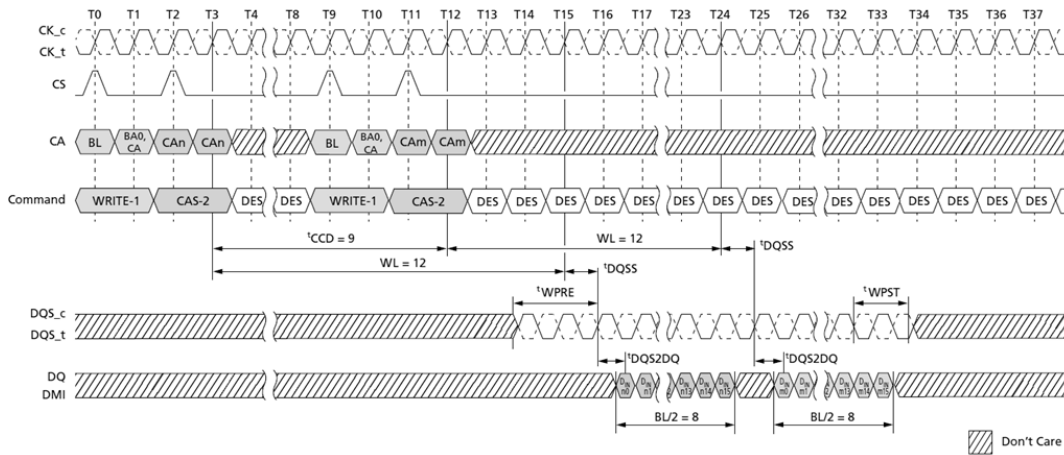
Figure 50. Consecutive WRITE: t_{CCD} = \text{MIN} + 1, 1.5nCK Postamble
