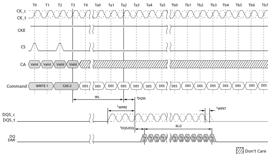
Figure 10. DQS Write Preamble and Postamble – 0.5nCK Postamble
