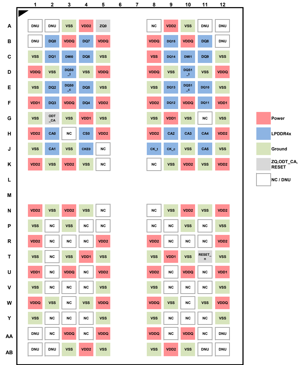
Figure 2. Ball Configuration (Top View)
