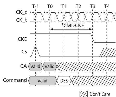
Figure 159. t_{CMDCKE} Timing
