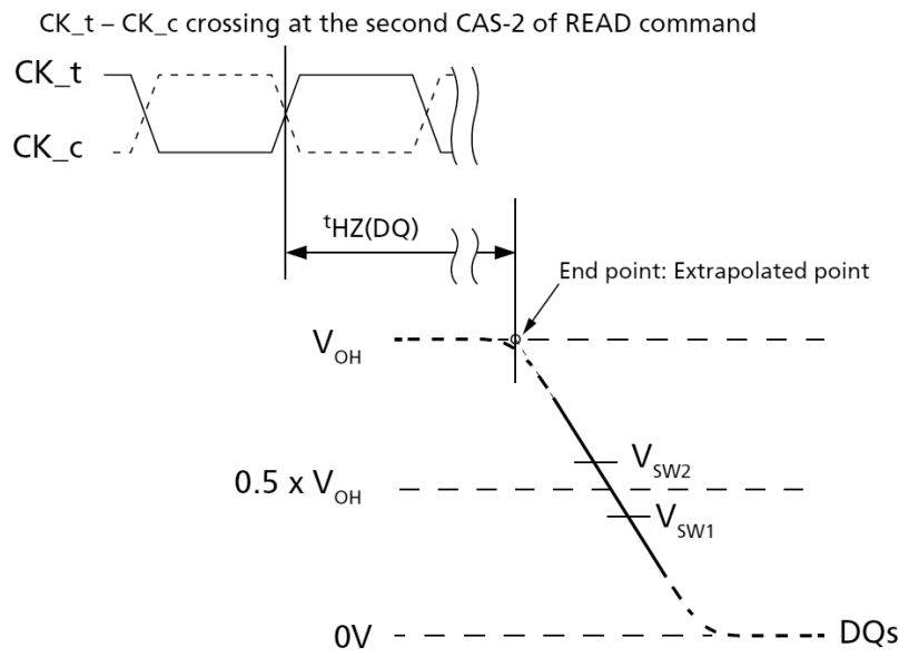
Figure 19. t HZ(DQ) Method for Calculating Transitions and Endpoint
