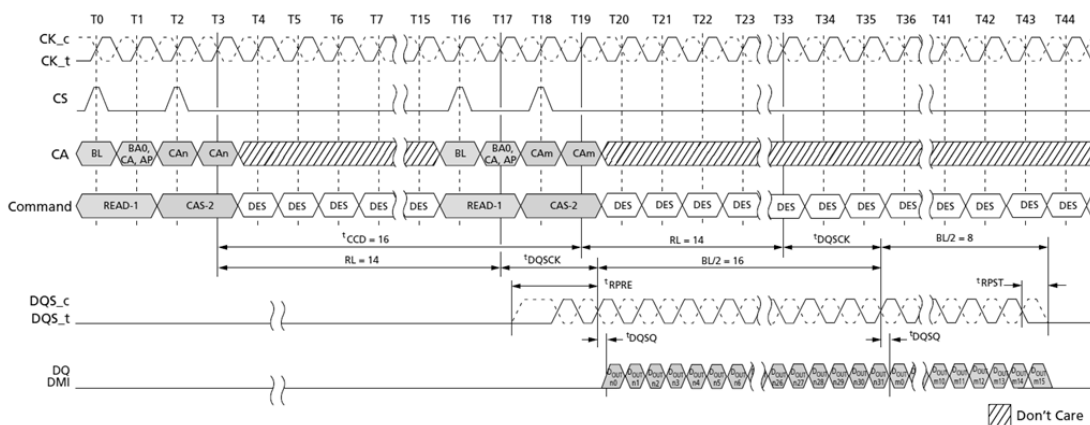
Figure 173. Burst Read Timing
