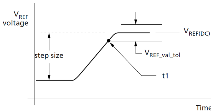
Figure 102. V_{REF(DQ)} Single-Step Size Increment
