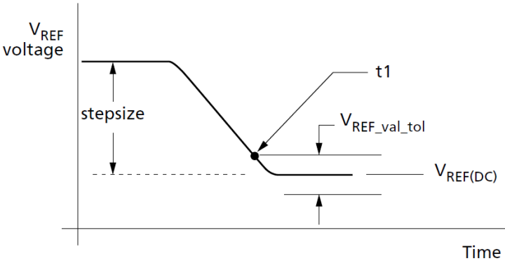
Figure 103. V_{REF(DQ)} Single-Step Size Decrement
