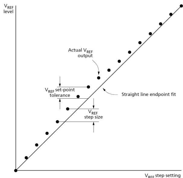
Figure 182. V_{REF} Set-Point Tolerance and Step Size
