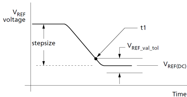
Figure 185. V_{REF(CA)} Single-Step Decrement
