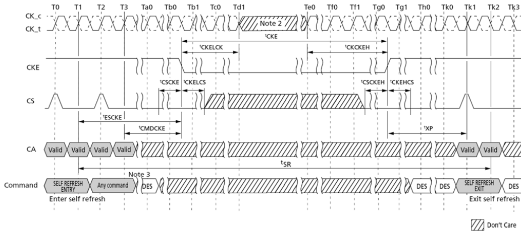
Figure 71. Self Refresh Entry/Exit Timing with Power-Down Entry/Exit
