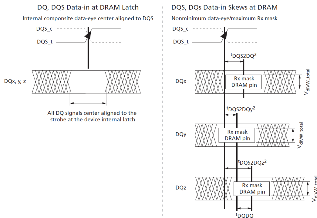
Figure 169. DQ-to-DQS t_{DQS2DQ} and t_{DQDQ}
