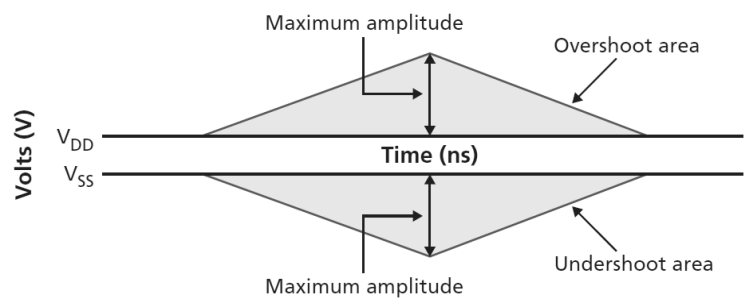
Figure 155. Overshoot and Undershoot Definition
