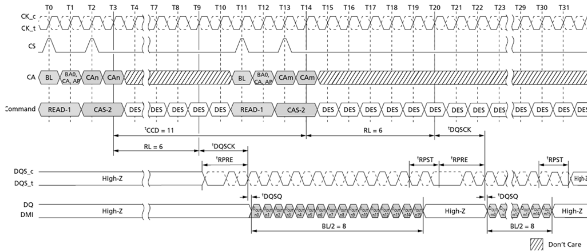
Figure 42. Consecutive READ: t_{CCD} = MIN + 3 , Preamble = Toggle, 1.5nCK Postamble
