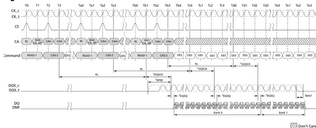
Figure 175. Seamless Burst Read
