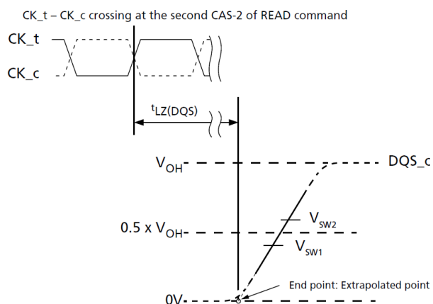
Figure 177. t LZ(DQS) Method for Calculating Transitions and Endpoint
