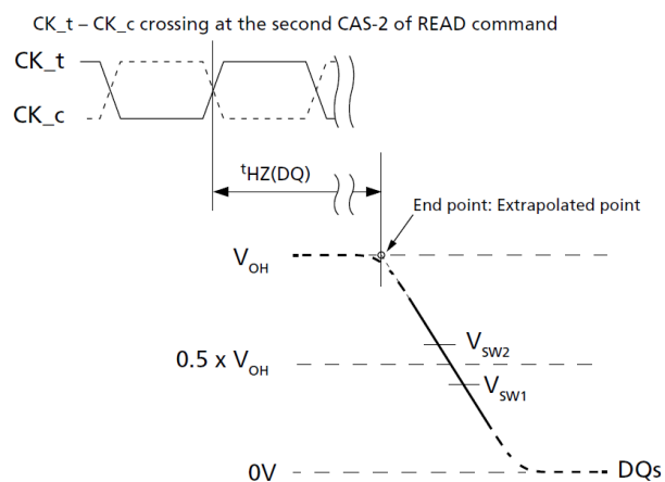
Figure 180. t_{HZ}(DQ) Method for Calculating Transitions and Endpoint
