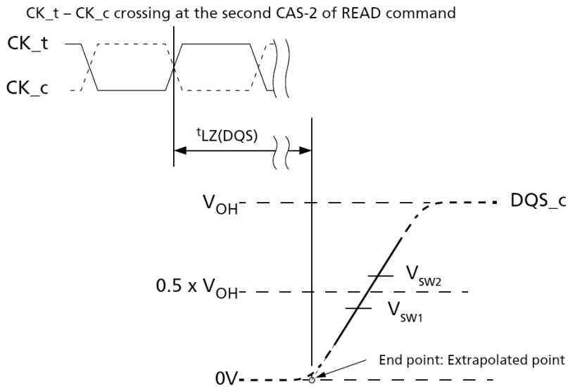
Figure 16. t_{LZ}(DQS) Method for Calculating Transitions and Endpoint
