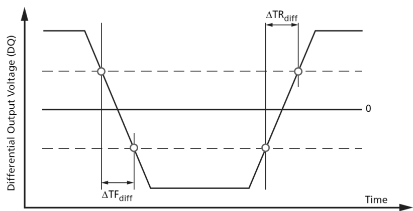
Figure 154. Differential Output Slew Rate Definition
