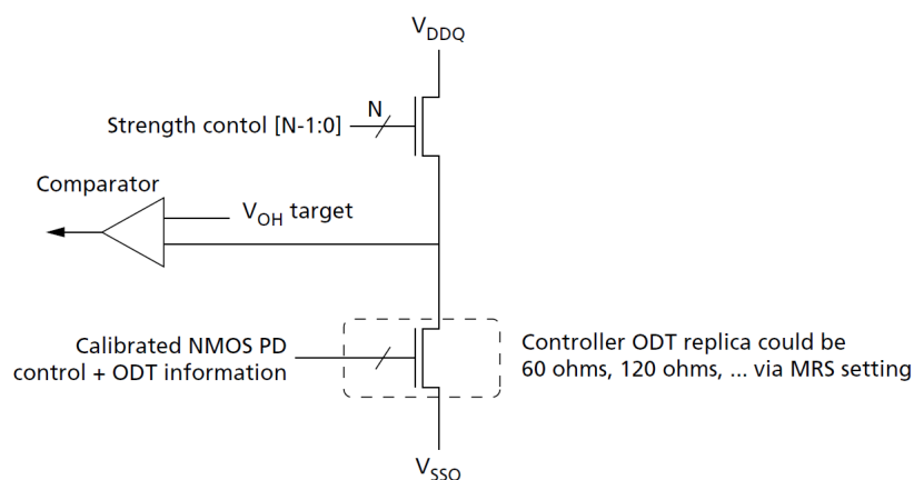
Figure 204. Pull-Up Calibration
