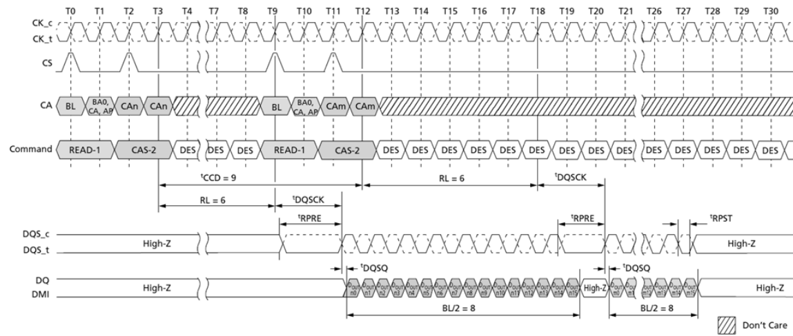
Figure 37. Consecutive READ: t_{CCD} = \text{MIN} + 1 , Preamble = Static, 0.5nCK Postamble
