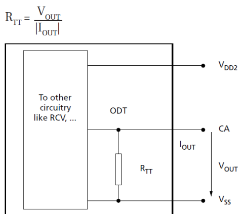
Figure 134. ODT for CA
