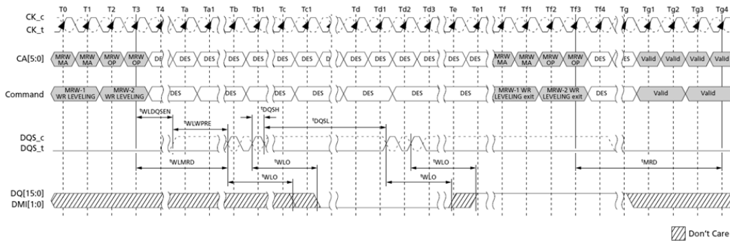
Figure 110. Write Leveling Timing – t_{DQSL}(\text{MAX})
