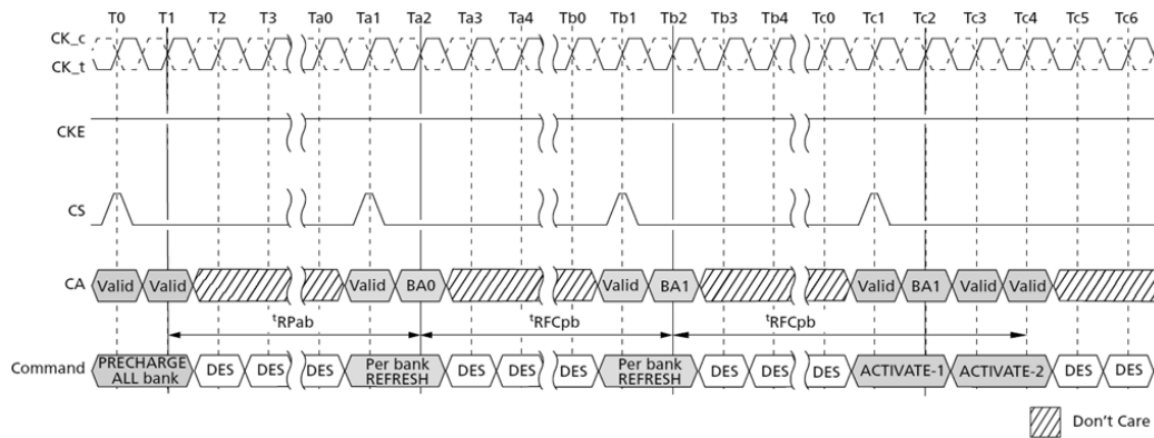
Figure 65. Per Bank REFRESH Operation
