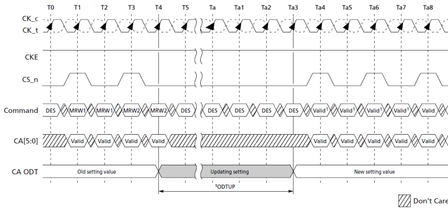
Figure 196. ODT for CA Setting Update Timing in 4-Clock Cycle Command
