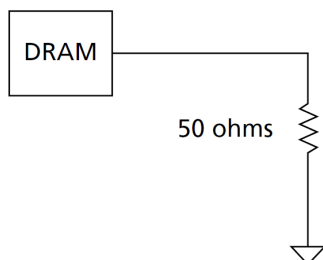
Figure 202. Driver Output Timing Reference Load
