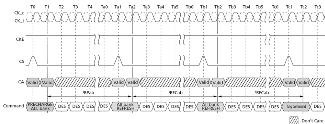
Figure 64. All-Bank REFRESH Operation
