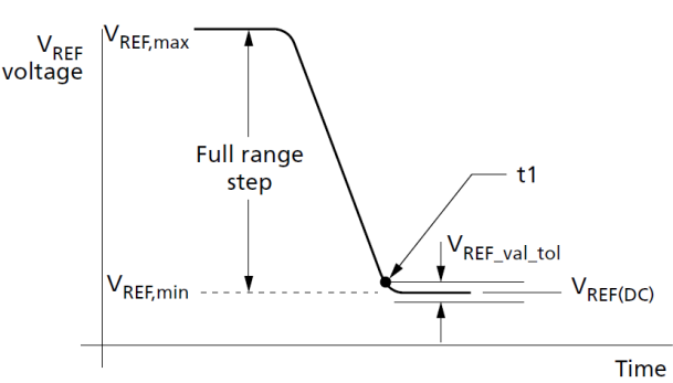
Figure 194. V_{REF(DQ)} Full Step from V_{REF,max} to V_{REF,min}
