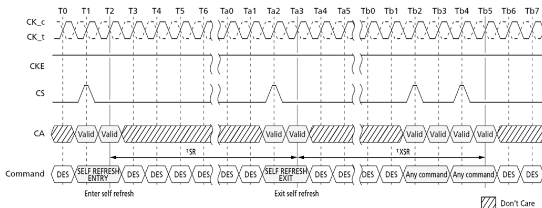
Figure 70. Self Refresh Entry/Exit Timing
