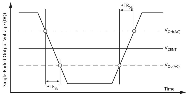
Figure 199. Single-Ended Output Slew Rate Definition
