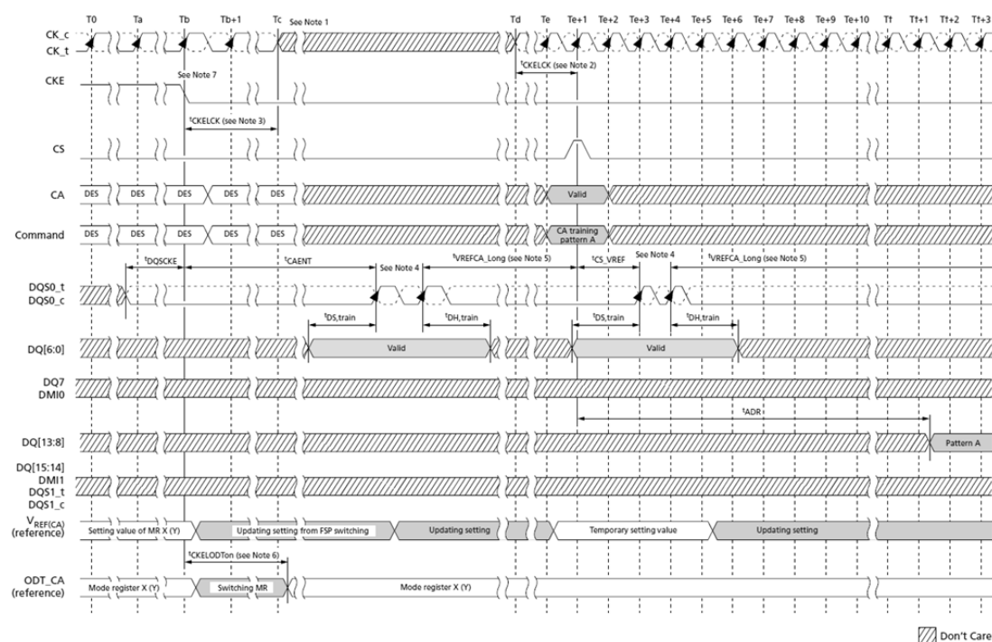
Figure 107. Consecutive V_{REF(CA)} Value Update
