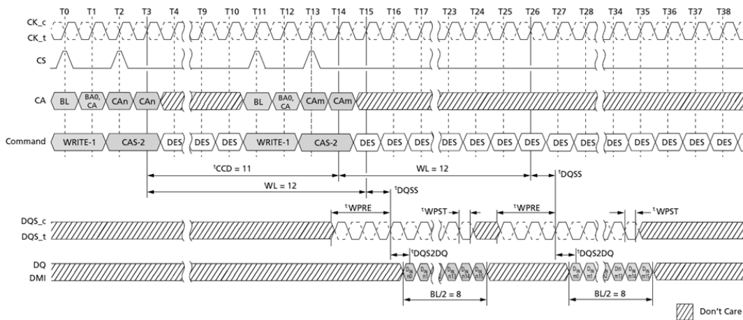
Figure 53. Consecutive WRITE: t_{CCD} = \text{MIN} + 3, 0.5nCK Postamble
