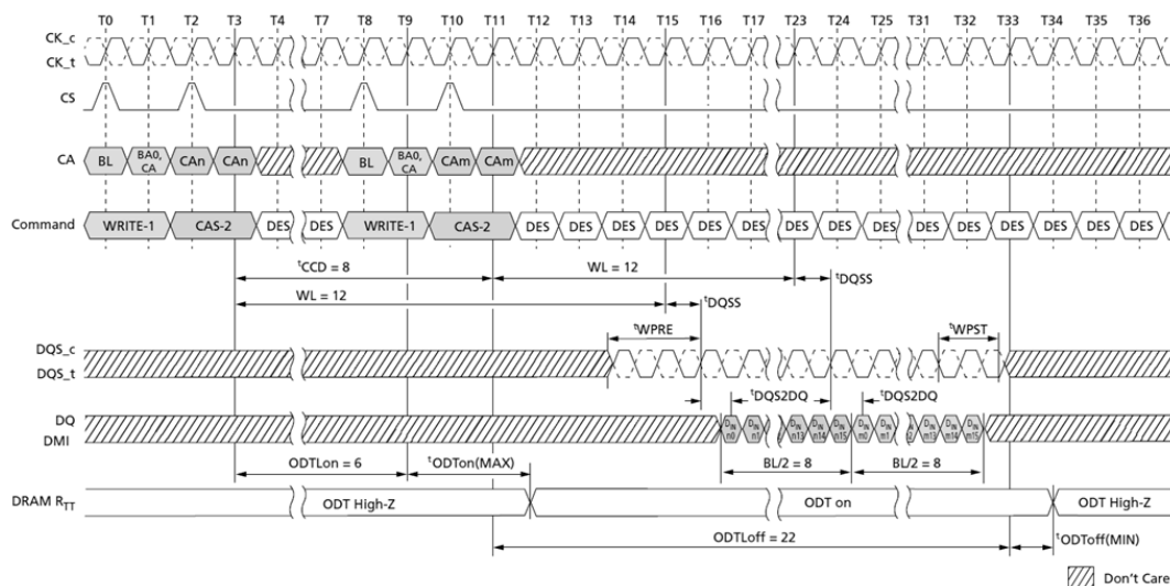
Figure 47. Seamless WRITE: t_{CCD} = \text{MIN} , 1.5nCK Postamble, 533 \text{ MHz} < \text{Clock Frequency} \leq 800 \text{ MHz} , ODT Worst Timing Case
