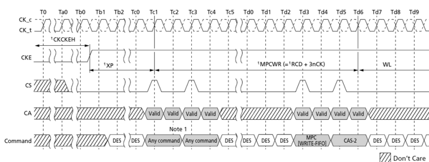
Figure 124. Power-Down Exit to MPC[WRITE-FIFO] Timing
