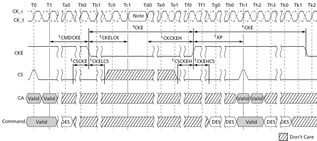
Figure 75. Basic Power-Down Entry and Exit Timing
