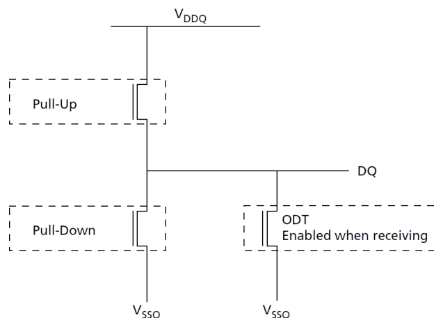
Figure 203. LVSTL I/O Cell
