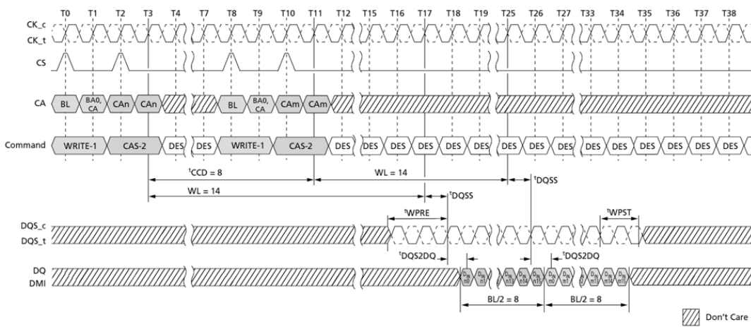
Figure 48. Seamless WRITE: t_{CCD} = \text{MIN} , 1.5nCK Postamble
