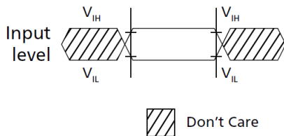
Figure 142. Input Timing Definition for RESET n
