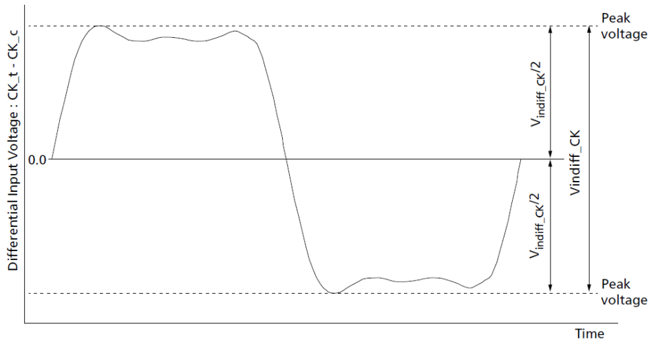
Figure 143. CK Differential Input Voltage
