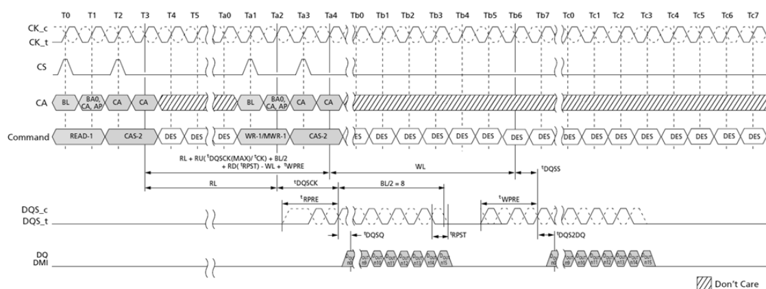
Figure 13. Burst Read Followed by Burst Write or Burst Mask Write
