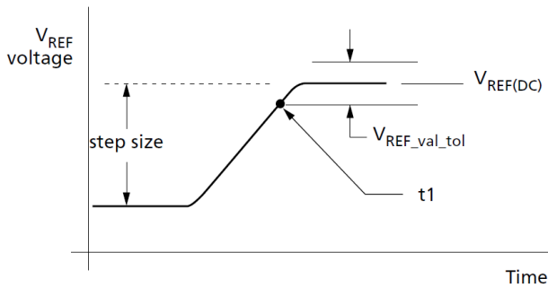
Figure 191. V_{REF(DQ)} Single-Step Size Increment
