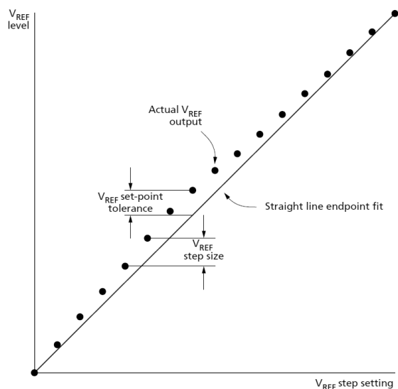
Figure 189. V_{REF} Set Tolerance and Step Size
