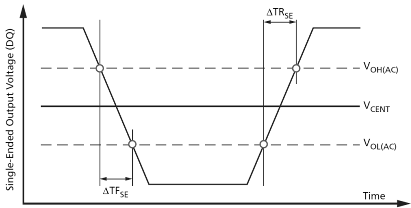
Figure 153. Single-Ended Output Slew Rate Definition
