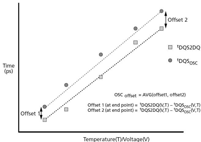
Figure 125. Interval Oscillator Offset – OSC_{offset}
