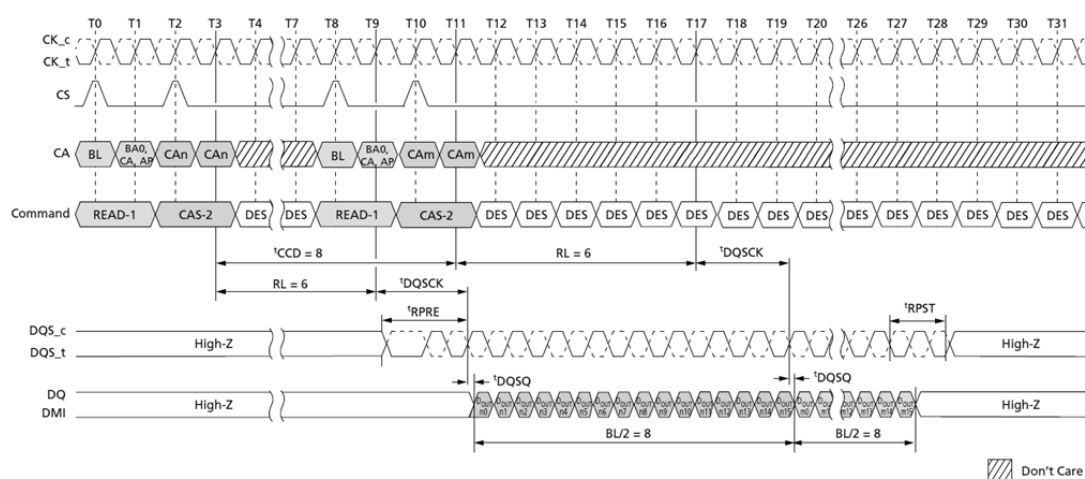
Figure 33. READ Operations: t_{CCD} = \text{MIN} , Preamble = Toggle, 1.5nCK Postamble
