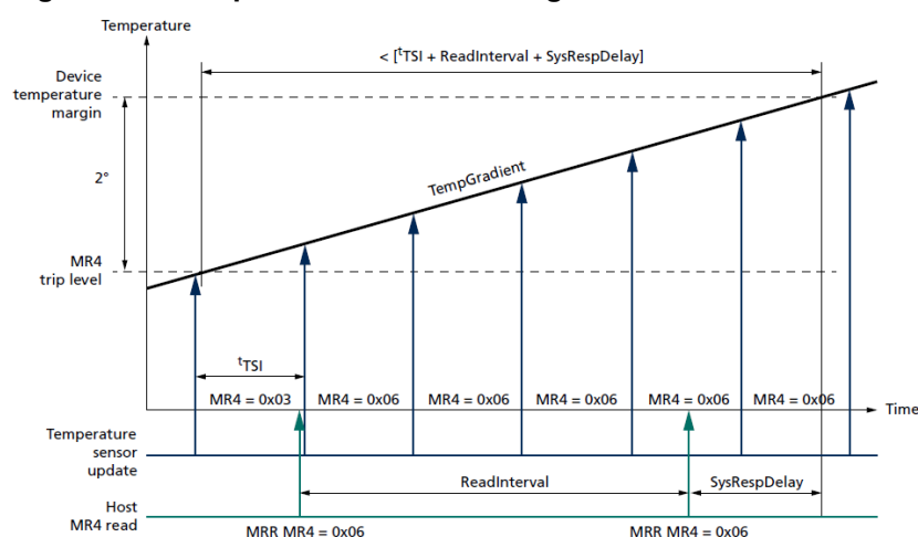
Figure 128. Temperature Sensor Timing
