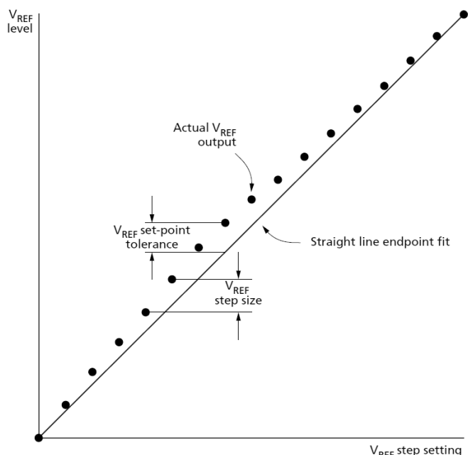
Figure 100. V_{REF} Set Tolerance and Step Size
