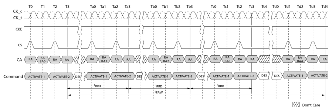
Figure 7. t_{FAW} Timing
