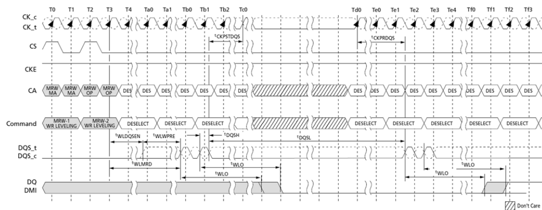
Figure 112. Clock Stop and Timing During Write Leveling
