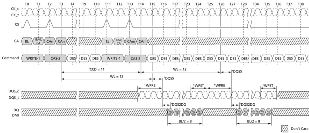
Figure 54. Consecutive WRITE: t_{CCD} = \text{MIN} + 3, 1.5nCK Postamble
