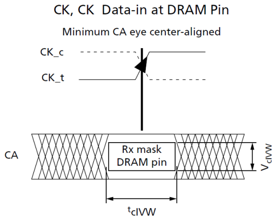
Figure 163. CA Timings at the DRAM Pins
