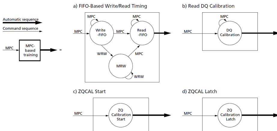
Figure 4. Simplified State Diagram
