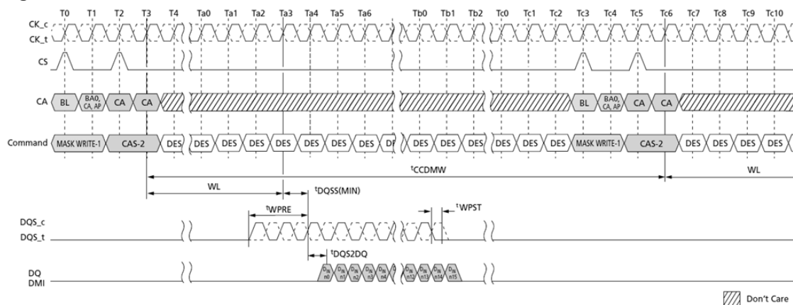
Figure 25. MASK WRITE Command – Same Bank
