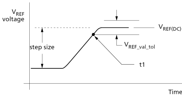
Figure 184. V_{REF(CA)} Single-Step Increment
