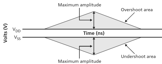
Figure 201. Overshoot and Undershoot Definition
