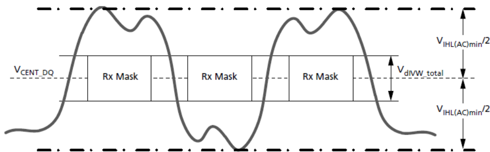
Figure 171. DQ V_{IHL(AC)} Definition (for Each Input Pulse)
