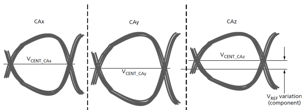
Figure 162. Across Pin V_{REF(CA)} Voltage Variation
