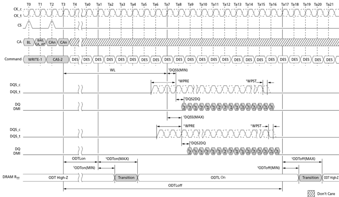
Figure 198. Asynchronous ODTon/ODToff Timing
