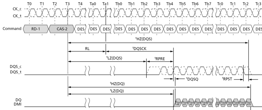
Figure 176. Read Timing
