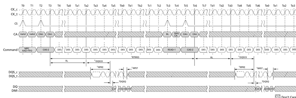
Figure 122. MPC[READ-FIFO] to Read Timing
