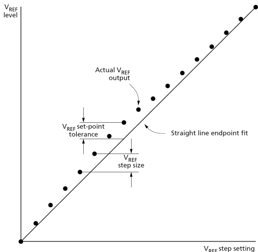
Figure 93. V_{REF} Set-Point Tolerance and Step Size
