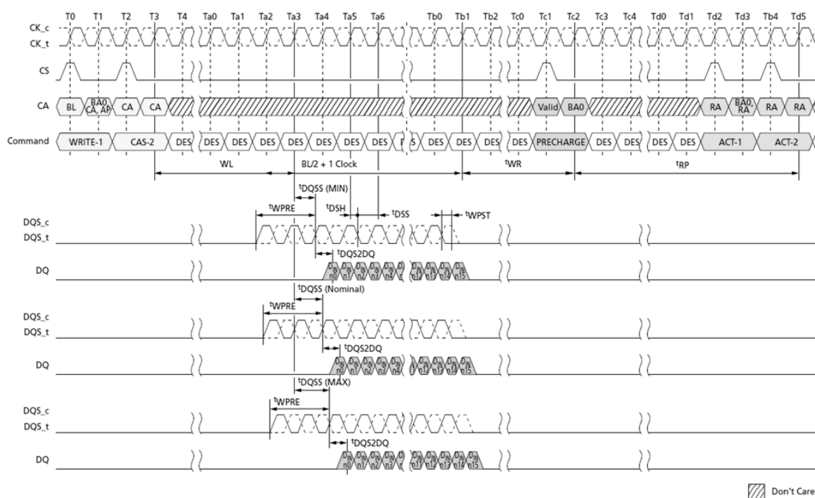
Figure 20. Burst WRITE Operation
