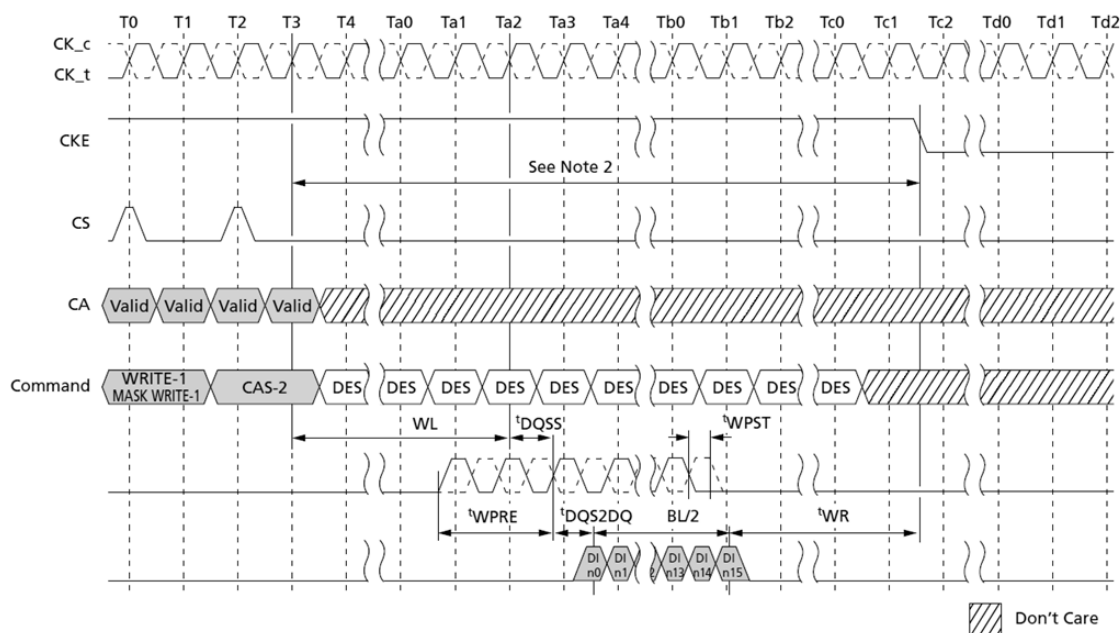
Figure 77. Write and Mask Write to Power-Down Entry
