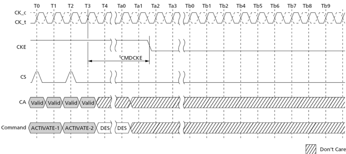
Figure 80. ACTIVATE Command to Power-Down Entry
