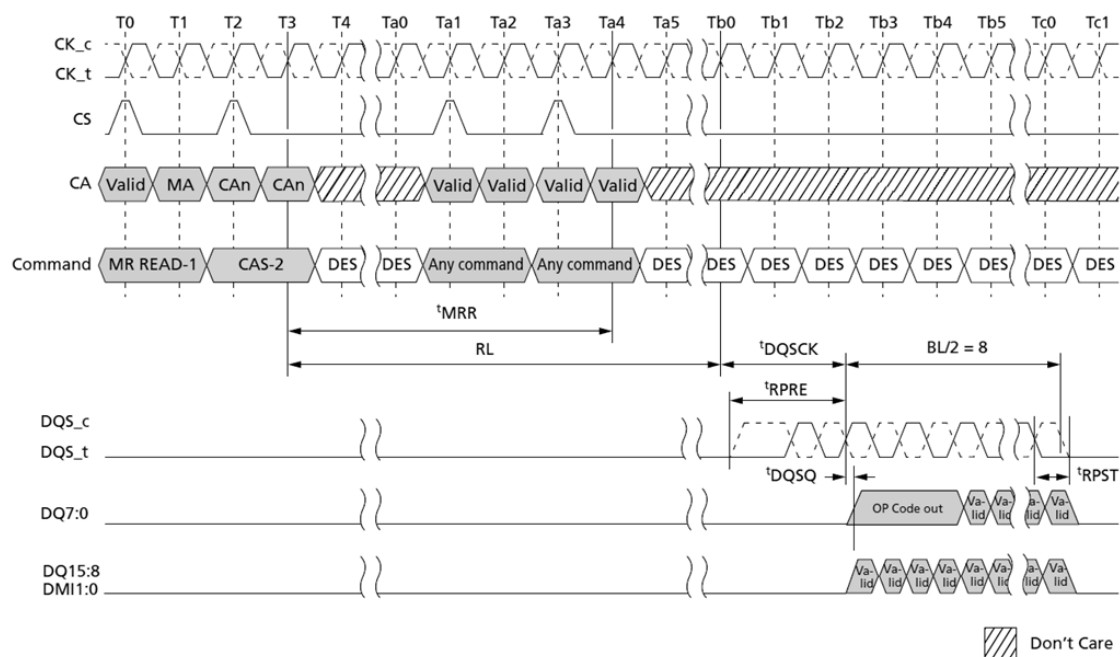
Figure 85. MODE REGISTER READ Operation
