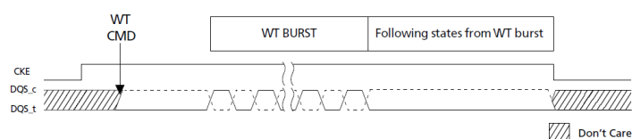
Figure 29. WDQS Control Mode 1
