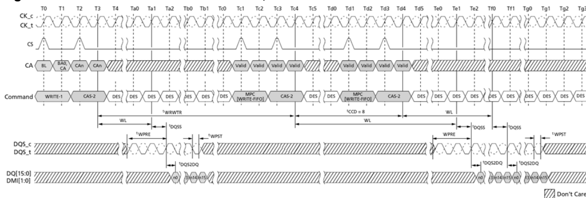
Figure 114. WRITE-FIFO – t_{WPRE} = 2nCK , t_{WPST} = 0.5nCK
