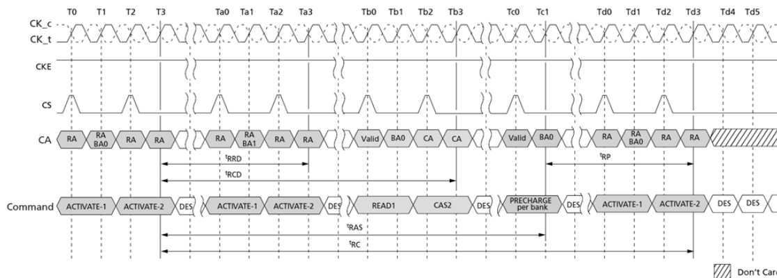
Figure 6. ACTIVATE Command
