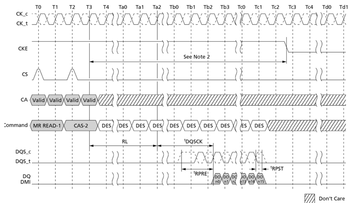
Figure 82. Mode Register Read to Power-Down Entry
