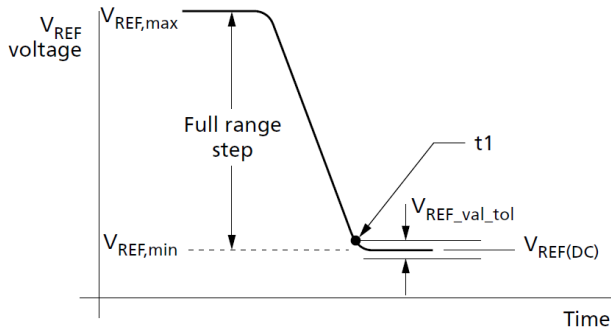
Figure 187. V_{REF(CA)} Full Step from V_{REF,max} to V_{REF,min}
