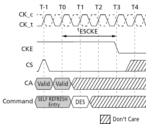
Figure 160. t ESCKE Timing
