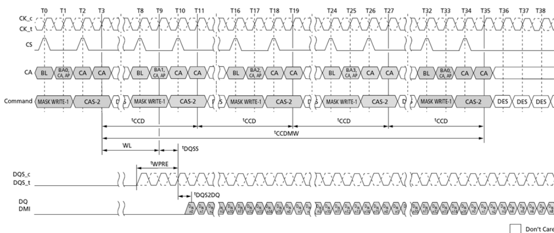
Figure 26. MASK WRITE Command – Different Bank
