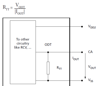
Figure 195. ODT for CA
