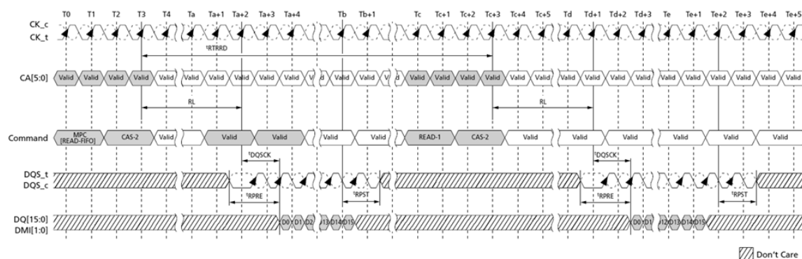
Figure 116. READ-FIFO – t_{RPRE} = \text{Toggle} , t_{RPST} = 1.5nCK
