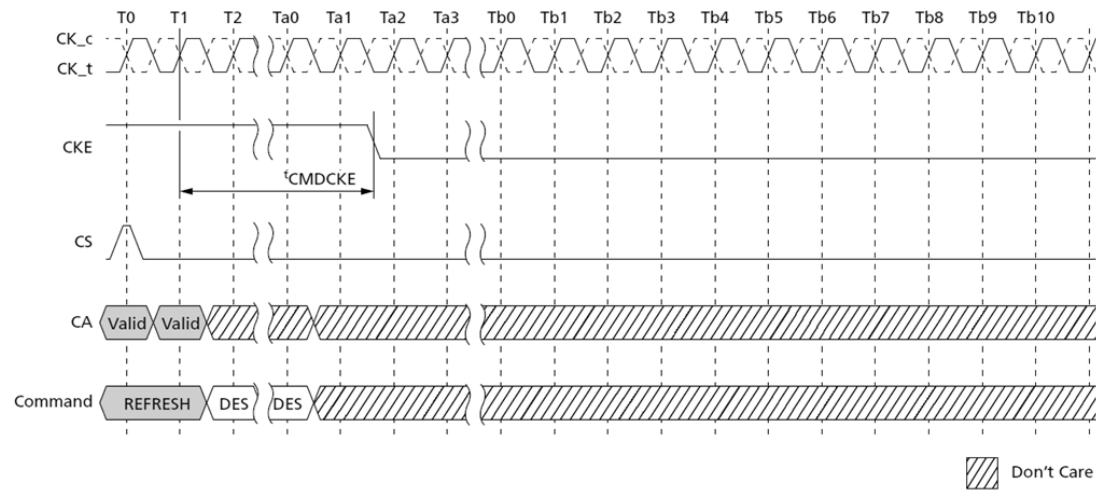
Figure 79. Refresh Entry to Power-Down Entry
