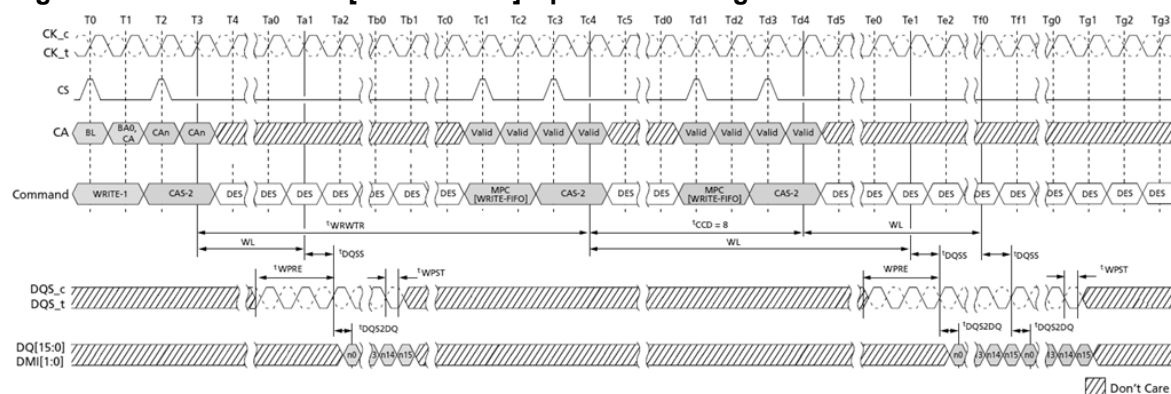
Figure 120. WRITE-to-MPC[WRITE-FIFO] Operation Timing
