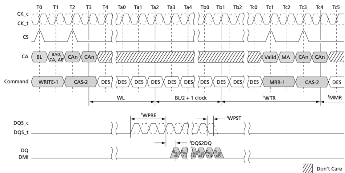
Figure 87. WRITE-to-MRR Timing
