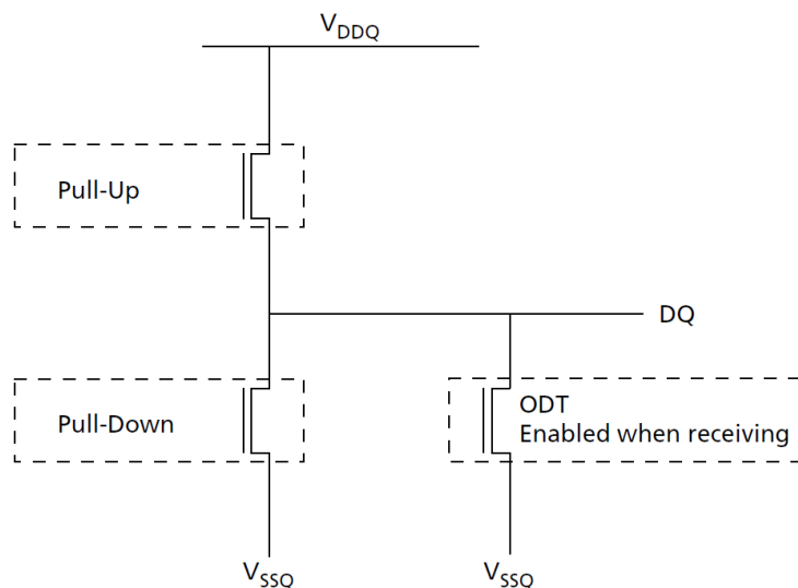
Figure 157. LVSTL I/O Cell
