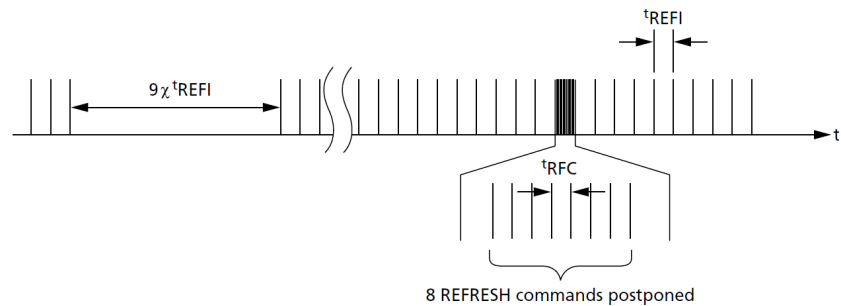
Figure 66. Postponing REFRESH Commands (Example)
