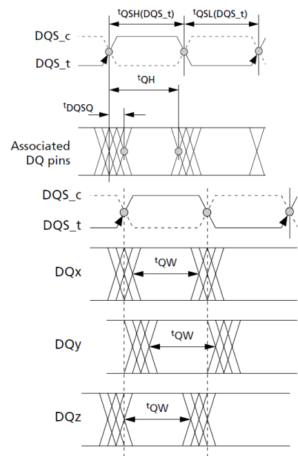
Figure 166. Read Data Timing Definitions – t_{QH} and t_{DQSQ} Across DQ Signals per DQS Group
