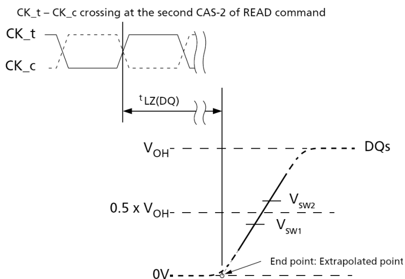
Figure 18. t_{LZ}(DQ) Method for Calculating Transitions and Endpoint
