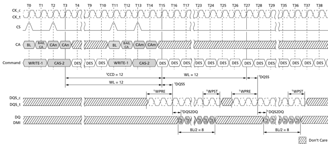
Figure 55. Consecutive WRITE: t_{CCD} = \text{MIN} + 4, 1.5nCK Postamble
