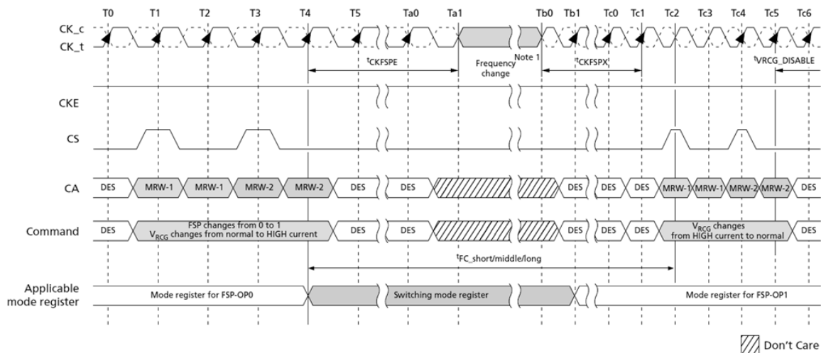
Figure 130. Frequency Set Point Switching Timing
