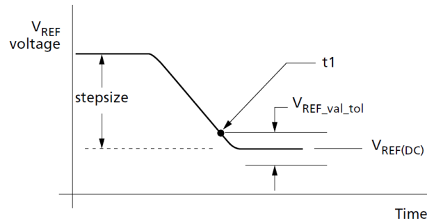
Figure 192. V_{REF(DQ)} Single-Step Size Decrement
