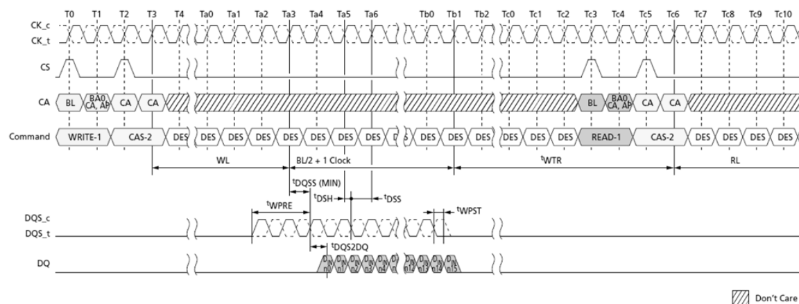
Figure 21. Burst Write Followed by Burst Read
