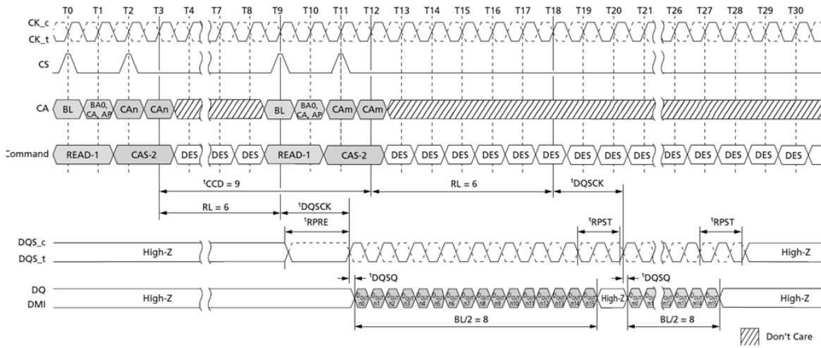
Figure 36. Consecutive READ: t_{CCD} = \text{MIN} + 1 , Preamble = Static, 1.5nCK Postamble
