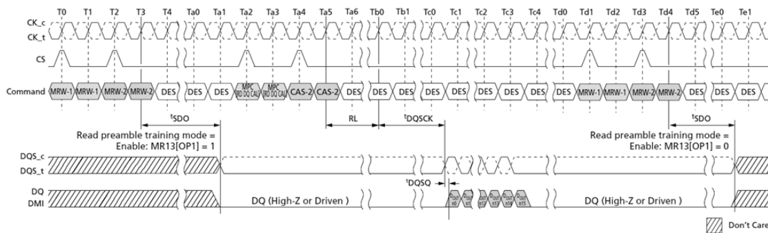
Figure 140. Read Preamble Training
