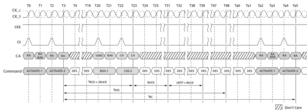
Figure 62. Command Input Timing with RAS Lock
