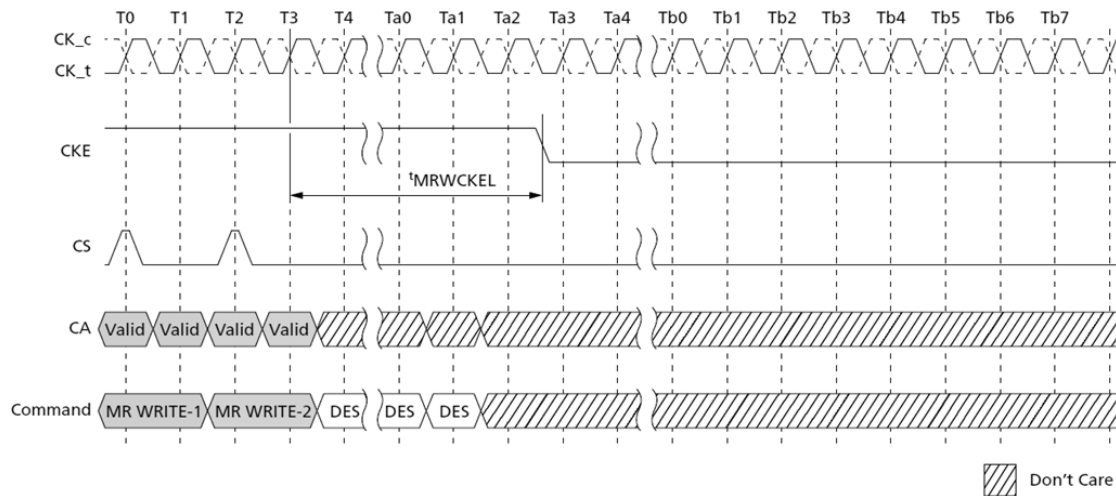
Figure 83. Mode Register Write to Power-Down Entry
