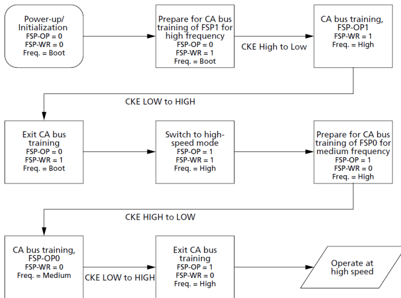
Figure 131. Training for Two Frequency Set Points
