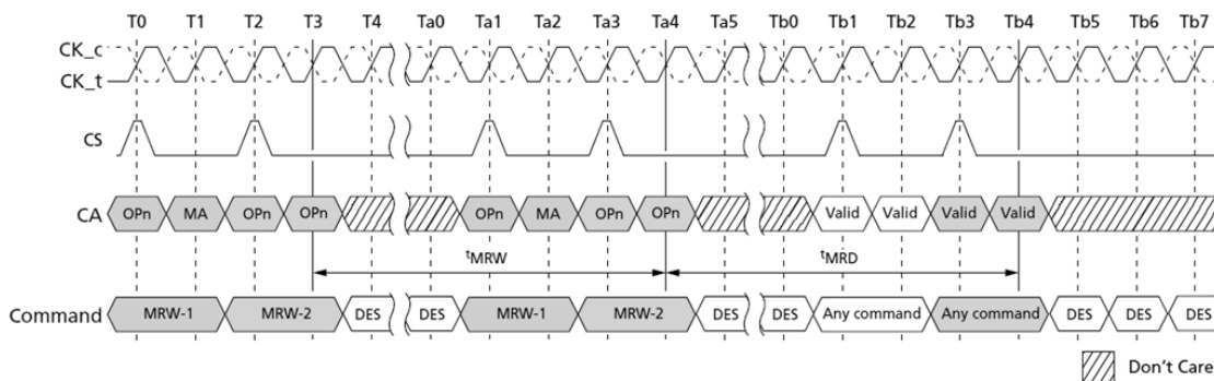
Figure 89. MODE REGISTER WRITE Timing
