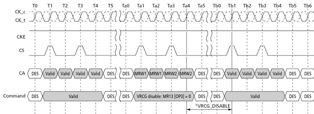
Figure 91. VRCG Disable Timing
