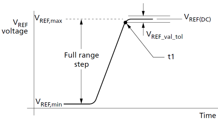
Figure 97. V_{REF(CA)} Full Step from V_{REF,min} to V_{REF,max}
