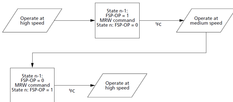
Figure 132. Example of Switching Between Two Trained Frequency Set Points
