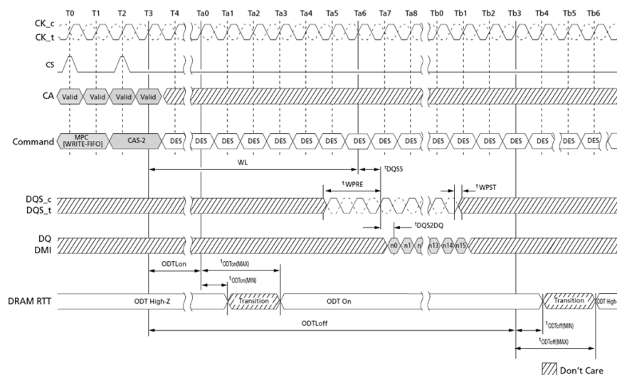
Figure 123. MPC[WRITE-FIFO] with DQ ODT Timing
