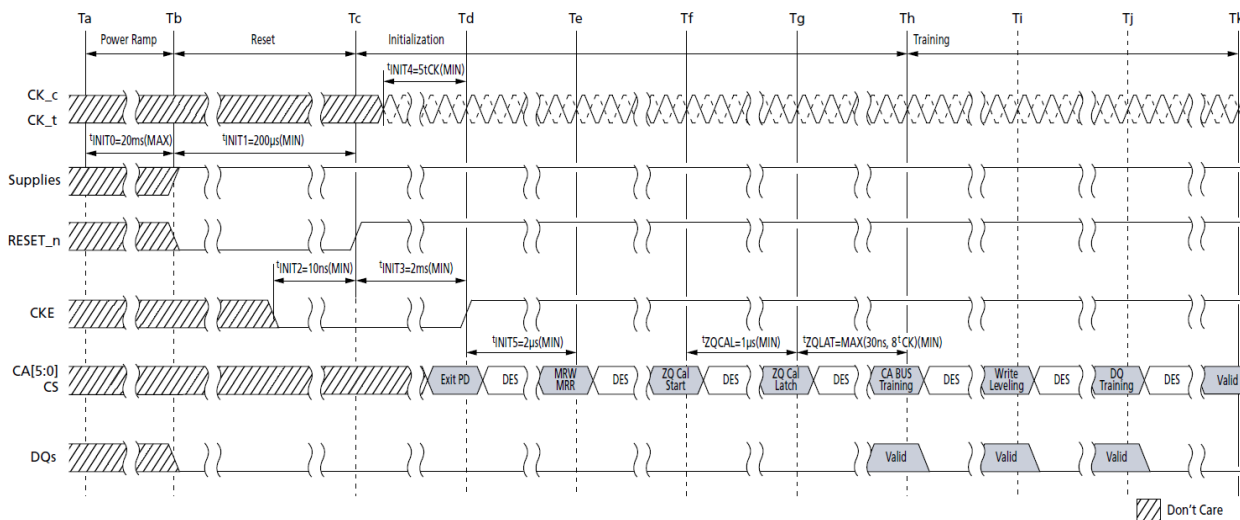
Figure 172. Voltage Ramp and Initialization Sequence
