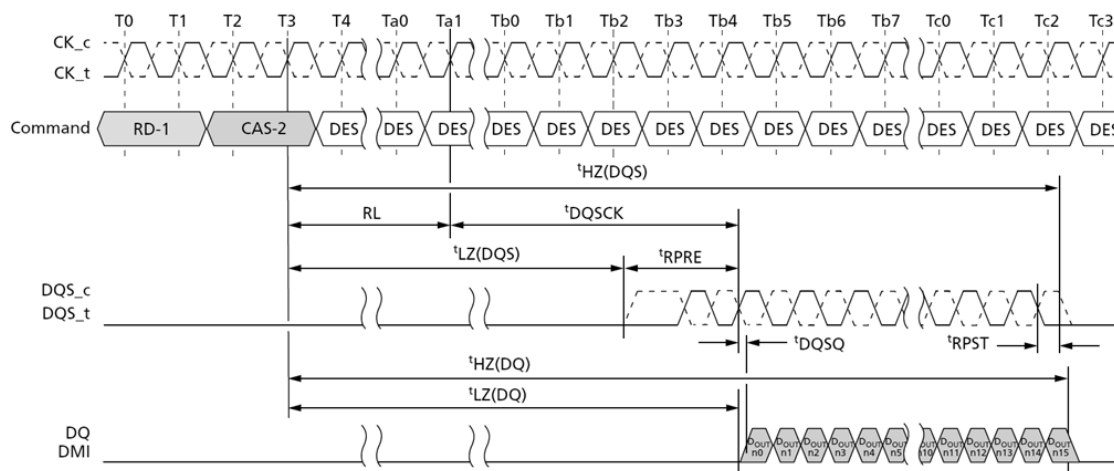
Figure 15. Read Timing
