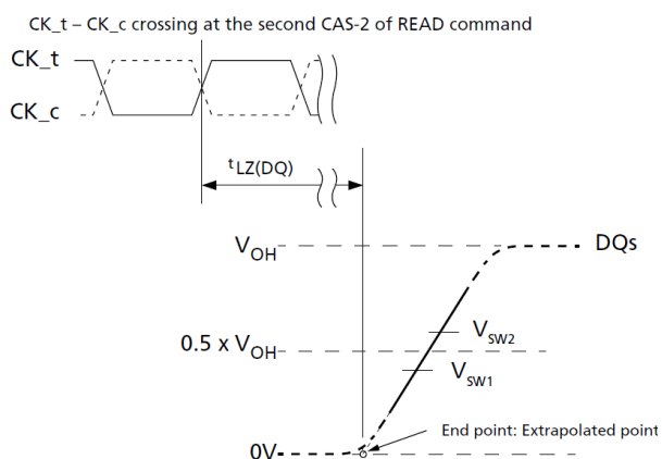
Figure 179. t_{LZ}(DQ) Method for Calculating Transitions and Endpoint
