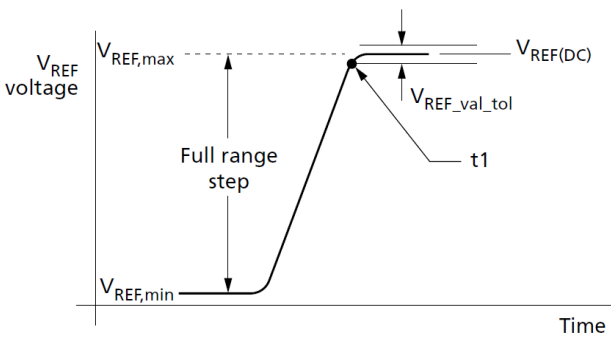
Figure 186. V_{REF(CA)} Full Step from V_{REF,min} to V_{REF,max}
