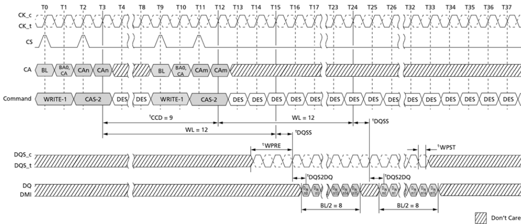
Figure 49. Consecutive WRITE: t_{CCD} = \text{MIN} + 1 , 0.5nCK Postamble
