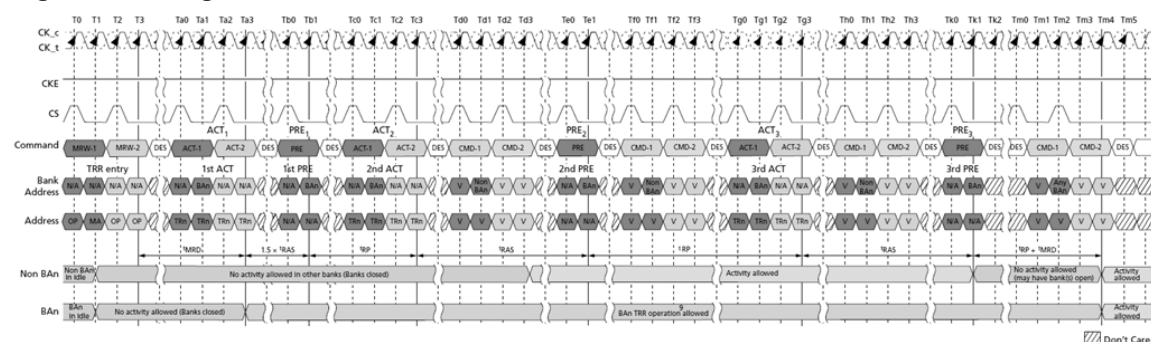
Figure 138. Target Row Refresh Mode
