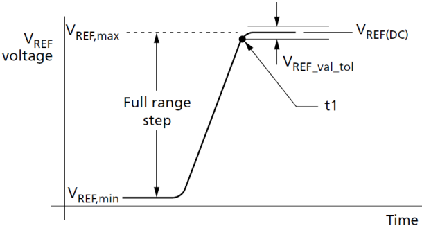
Figure 193. V_{REF(DQ)} Full Step from V_{REF,min} to V_{REF,max}
