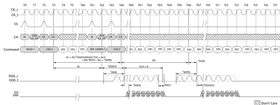
Figure 174. Burst Read Followed by Burst Write or Burst Mask Write
