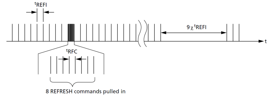
Figure 67. Pulling in REFRESH Commands (Example)
