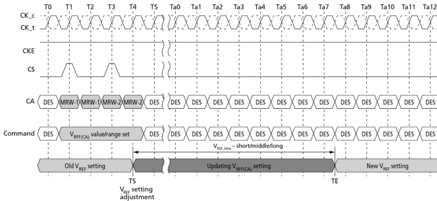
Figure 183. t_{V_{REF}} for Short, Middle, and Long Timing Diagram
