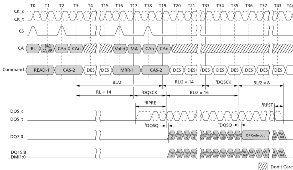
Figure 86. READ-to-MRR Timing
