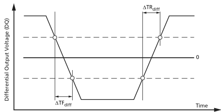
Figure 200. Differential Output Slew Rate Definition
