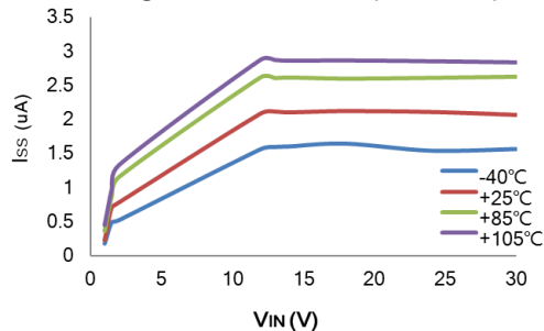
I_{SSL} vs V_{IN} : HT75RC0-7( I_{OUT}=0mA )
