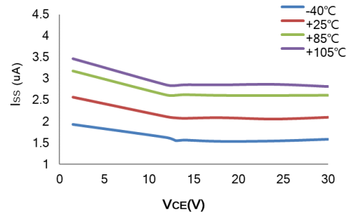
I_{SSL} vs V_{CE} : HT75RC0-7( I_{OUT}=0mA )
