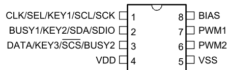
HT68RV032/HT68RV033/HT68RV034/HT68RV035 8 SOP-A
