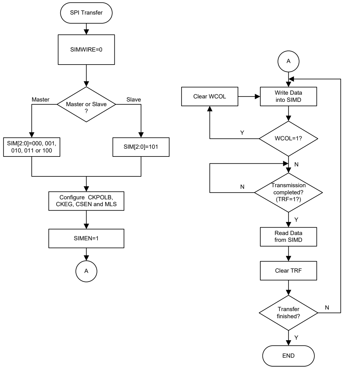
SPI Transfer Control Flow Chart – 4-wire Mode
