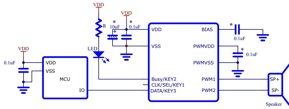
One-wire Mode Application Circuit
