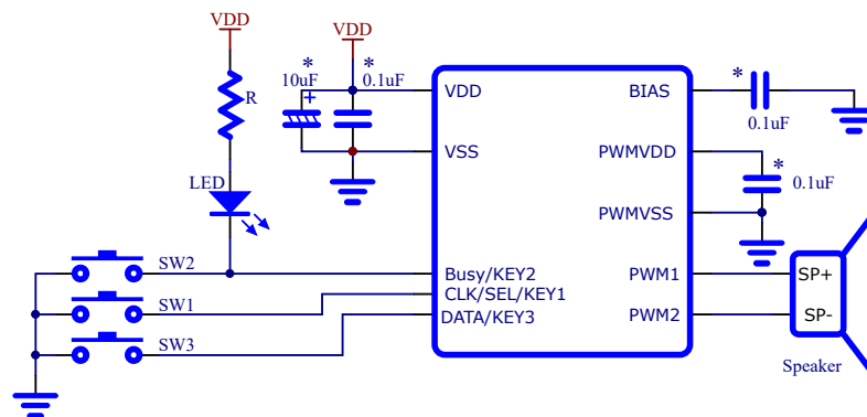
Direct Mode Application Circuit
