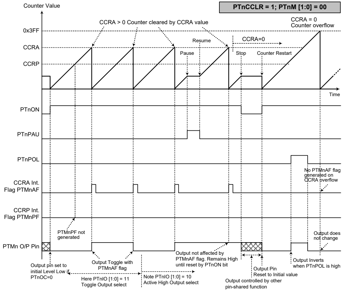
Compare Match Output Mode – PTnCCLR=1 ( n=0\sim1 )
