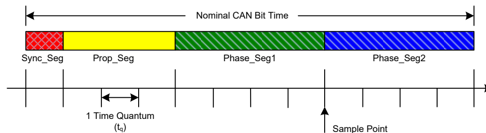
Bit Timing
