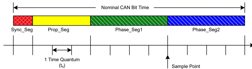
Bit Timing
