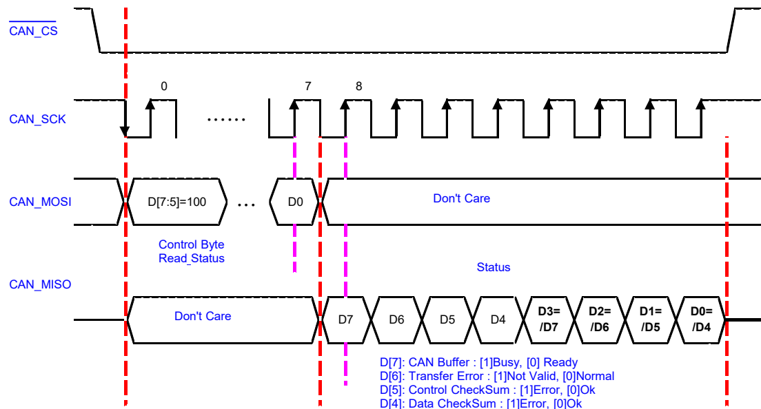
Read Status Timing Diagram
