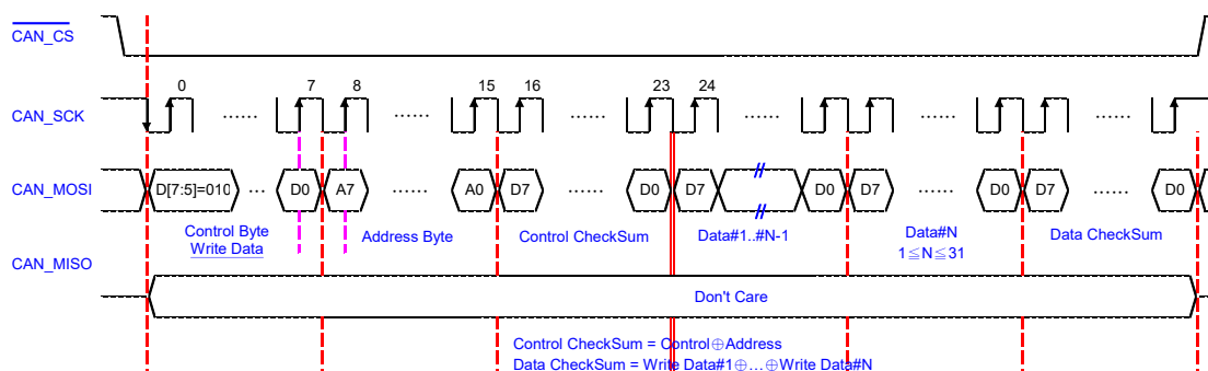
Write Data to Buffer Timing Diagram
