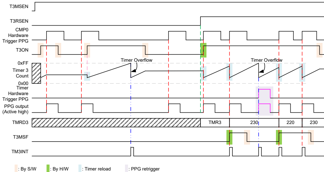
PPG Retrigger Function Mode Timing Chart
