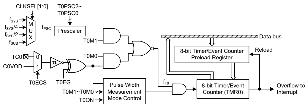
8-bit Timer/Event Counter 0
