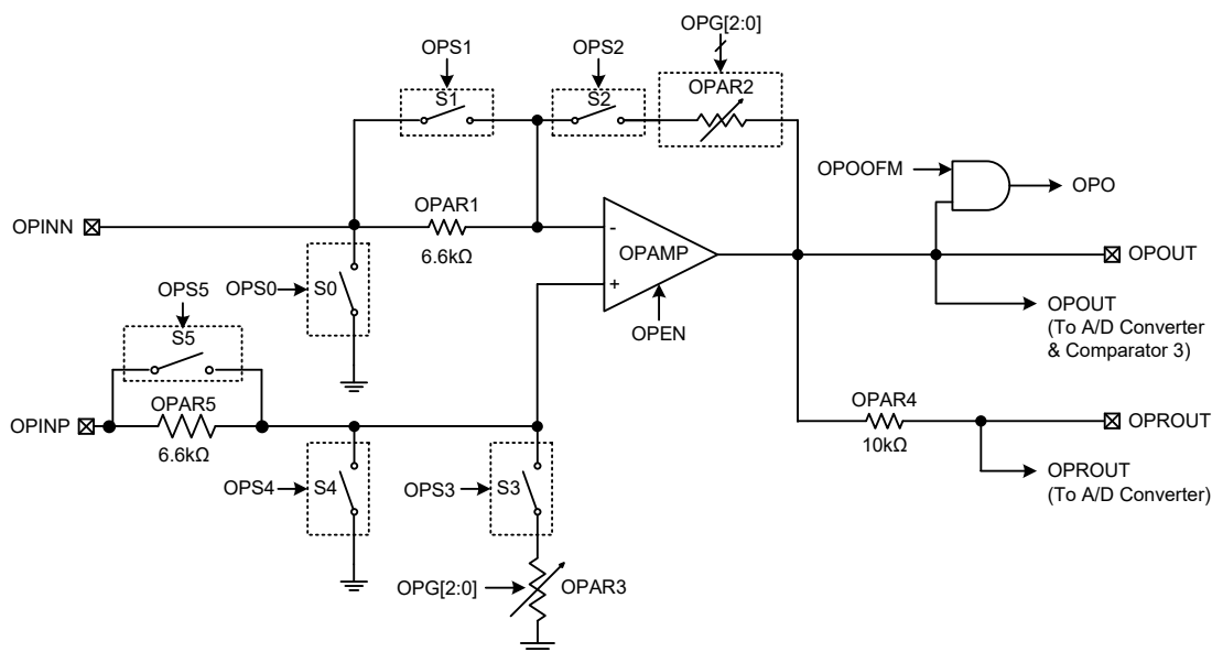
Operational Amplifier Block Diagram
