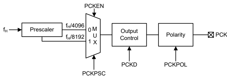
Peripheral Clock Output Block Diagram
