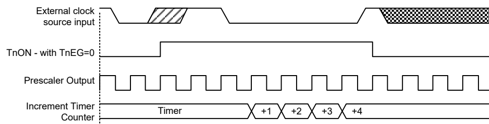
Pulse Width Measurement Mode Timing Chart – TnEG=0 (n=0/1/3)
