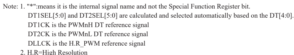
High Resolution PWM Registers
