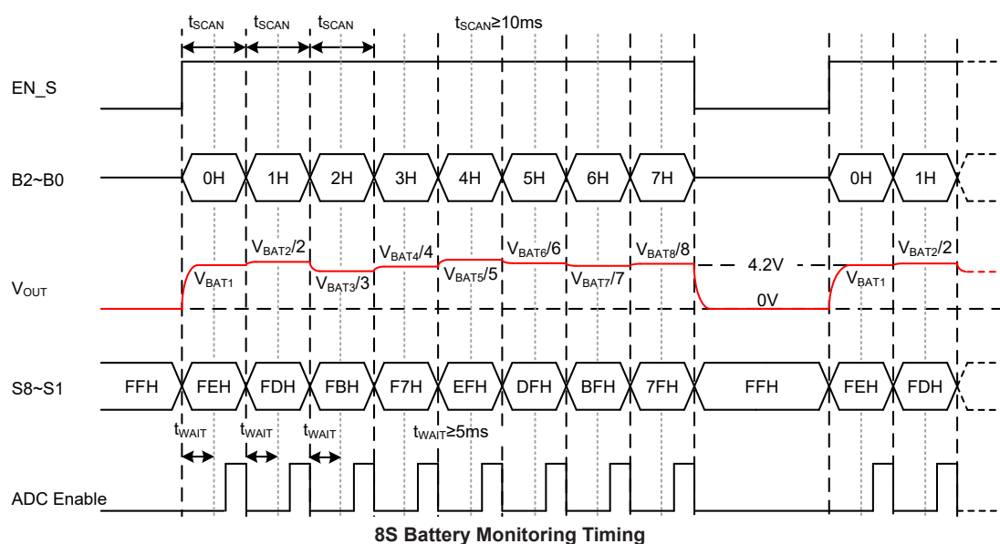
8S Battery Monitoring Timing
