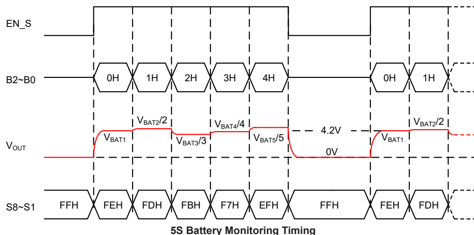
5S Battery Monitoring Timing
