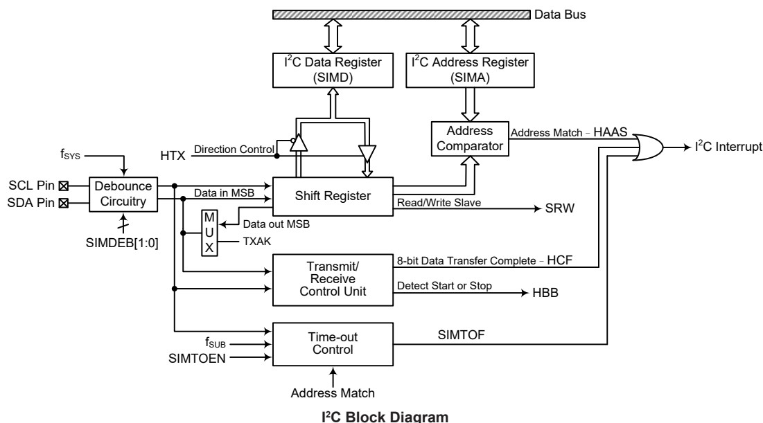
I²C Block Diagram
