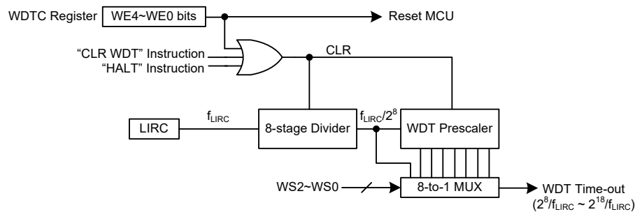
Watchdog Timer
