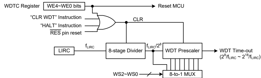
Watchdog Timer
