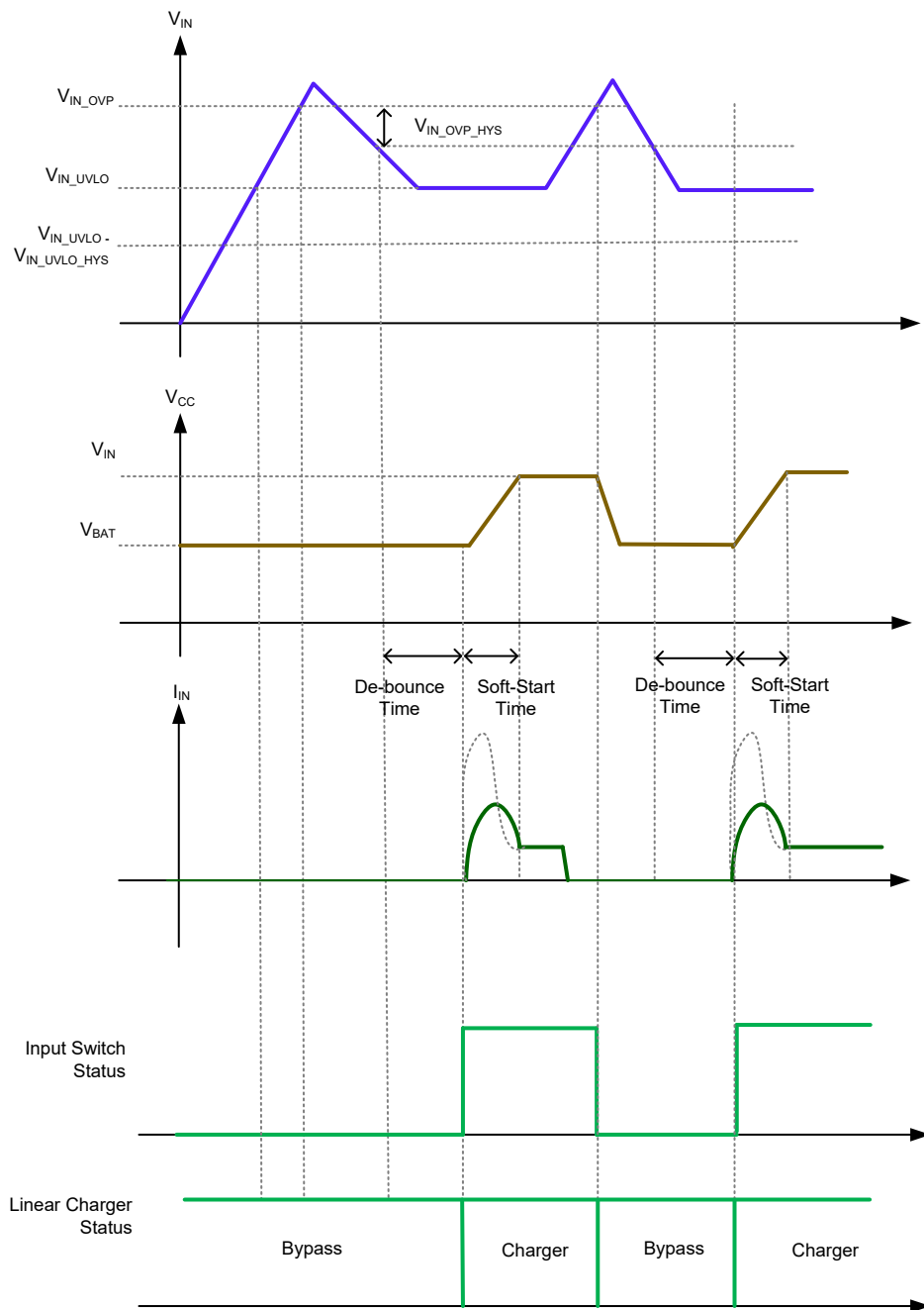
Principle Waveform and Block for Input OVP ( V_{IN} Power ON)
