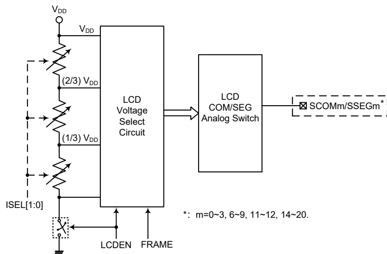
Software Controlled LCD Driver Structure
