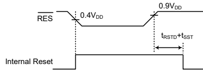
RES Reset Timing Chart
