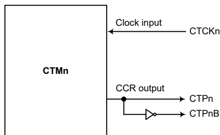
CTMn Function Pin Block Diagram (n=0~2)
