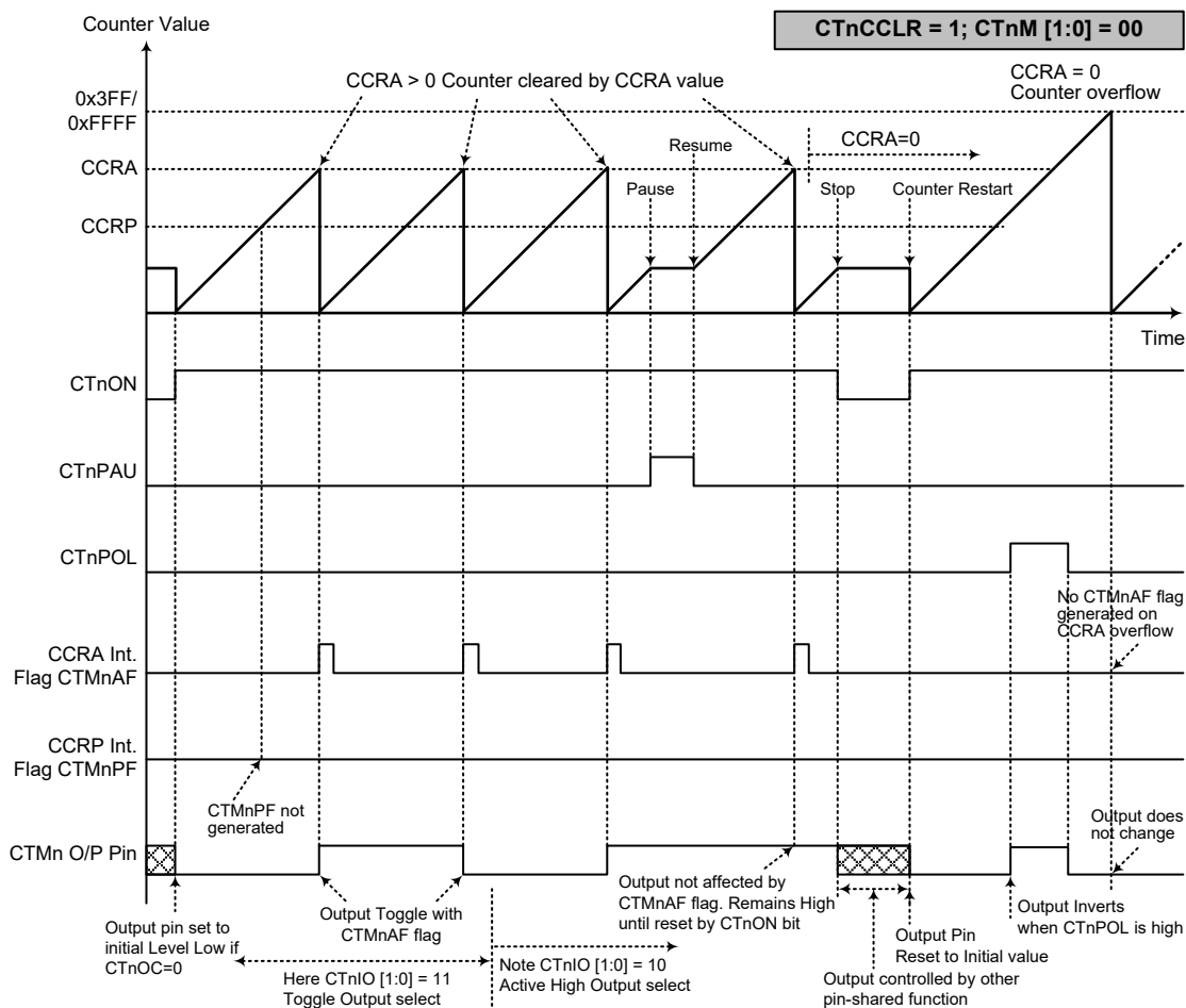
Compare Match Output Mode – CTnCCR=1
