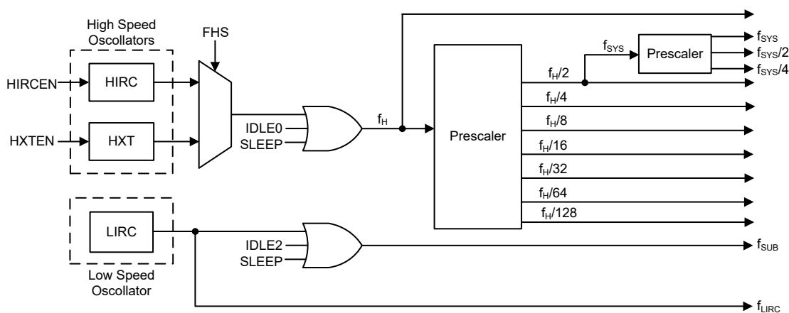
System Clock Configurations
