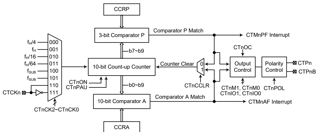
10-bit Compact Type TM Block Diagram (n=0~1)
