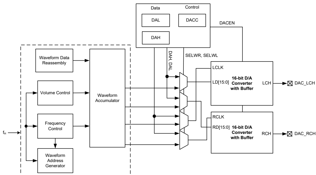
Music Music Synthesis Engine Block Diagram
