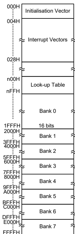
Program Memory Structure
