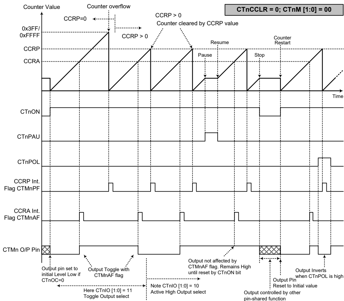
Compare Match Output Mode – CTnCCLR=0
