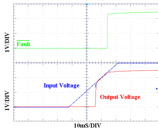
Power-Up Response
