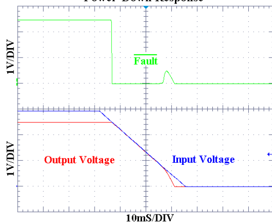
Power-Down Response
