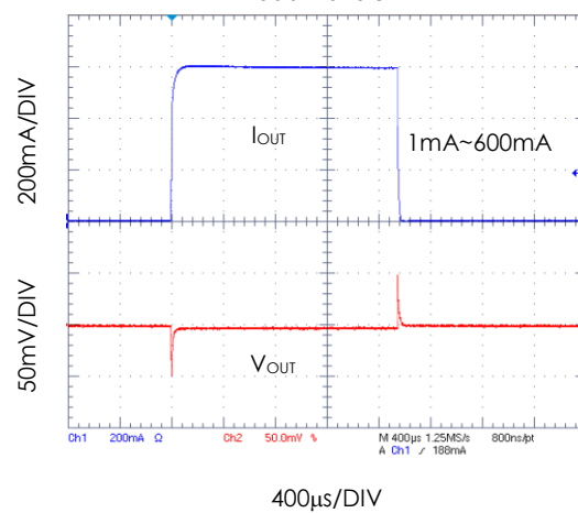
Load Transient
