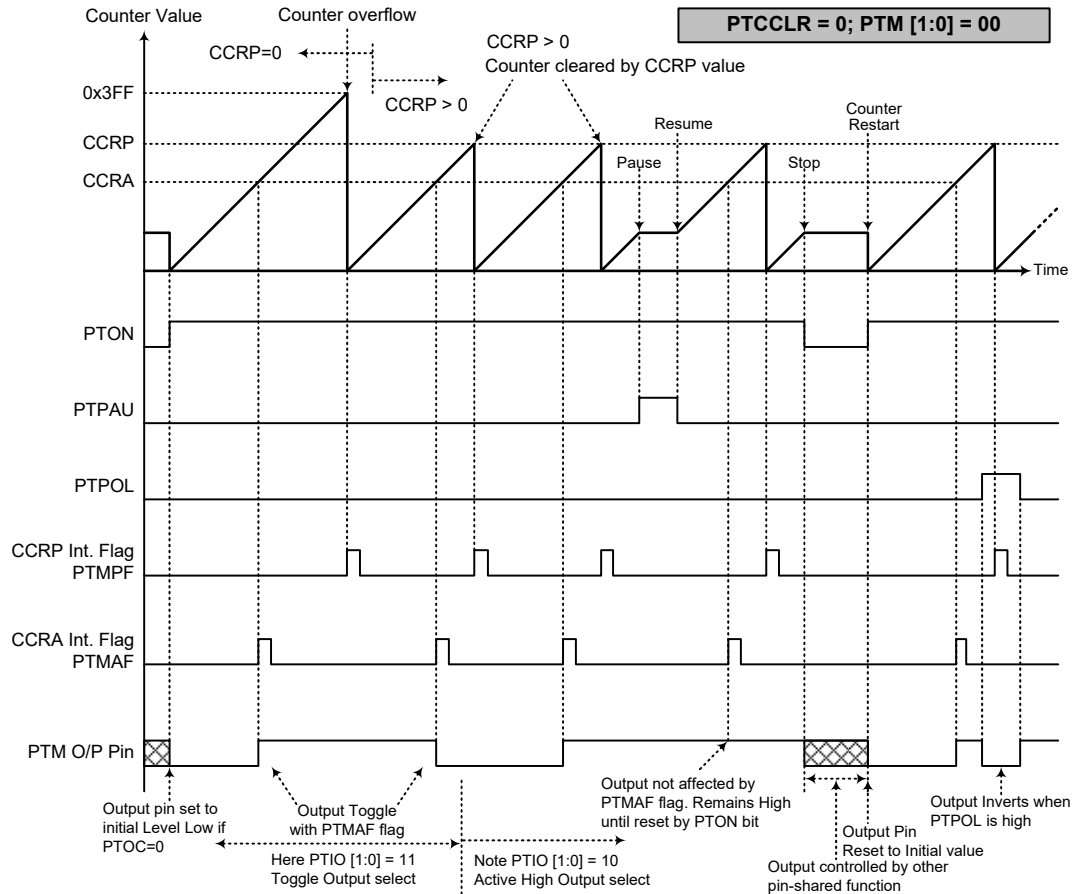
Compare Match Output Mode – PTCCLR=0
