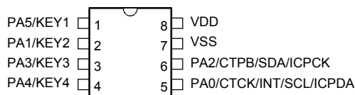
BS83B04C 8 SOP-A
