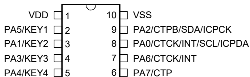
BS83B04C 10 MSOP-A/DFN-A
