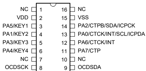
BS83BV04C 16 NSOP-A
