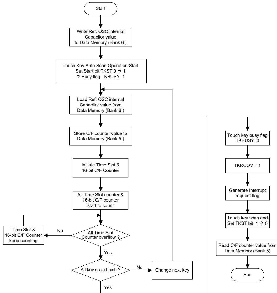
Touch Key Auto Scan Mode Flowchart
